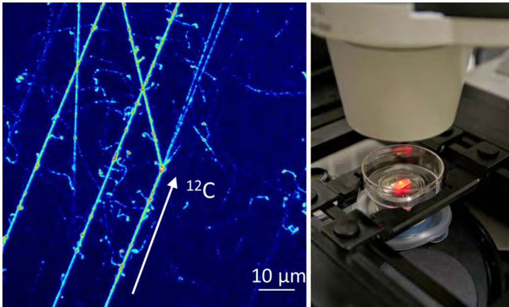
Figure 1: FNTD image (left) obtained using the Zeiss LSM710 ConfoCor 3 laser scanning confocal microscope (right) equipped with avalanche photo diodes. Carbon ions with a kinetic energy of 270\ \text{MeV/u} were incident parallel to the images crystal plane. The images is a maximum intensity projection of 13 images from different optical slices, resp. Beside the primary ion tracks, secondary electron tracks (curly features), a fragmentation event (center of left panel) and light fragments tracks (thin straight lines) are clearly visible.
