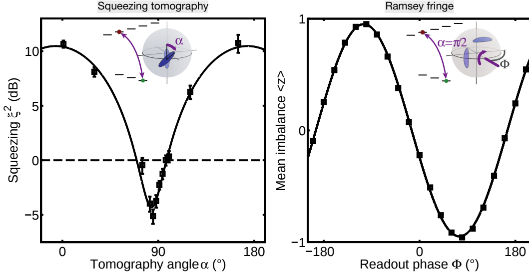
Figure 7.3.: Squeezing after state swapping. A squeezing tomography after the full interferometric sequence, consisting of state swapping, a hold time of 1\ \mu\text{s} , and swapping back, verifies that relative squeezing between left and right part of the full array of \xi_{\text{rel}}^2 = -5.1^{+0.6}_{-0.7}\text{ dB} is present (left panel). For a Ramsey fringe obtained after the same hold time of 1\ \mu\text{s} and a \pi/2 -pulse with varying readout phase, we find a visibility \mathcal{V} = 0.950(5) (right panel). Combined, using the Wineland criterion [101], this yields metrologically relevant spin squeezing of \xi_{\text{R}}^2 = -4.7(6)\text{ dB} after subtraction of detection noise and directly applicable squeezing of \xi_{\text{R}}^2 = -3.4(5)\text{ dB} without noise subtraction.
