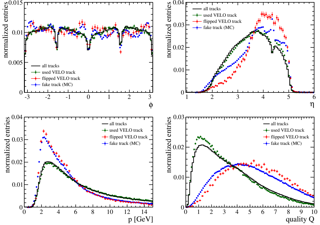
Figure 10.2.: Comparison of the track parameters \phi , \eta , p and the quality variable Q of the forward tracking algorithm, in different long track categories. Details are given in the text.
