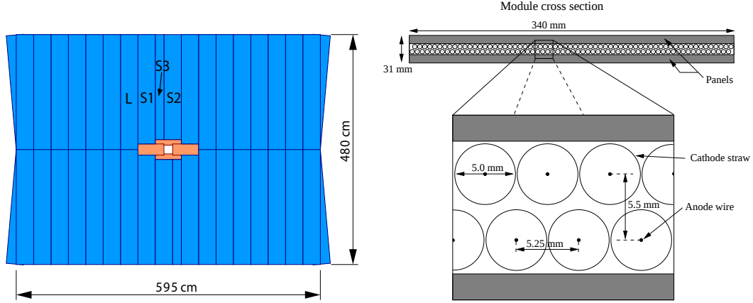
Figure 4.9.: a) Schematic view of an OT-station, the orange part indicates the IT. b) Cross section of an OT straw-tube module. Figures taken from Refs [63, 73].
