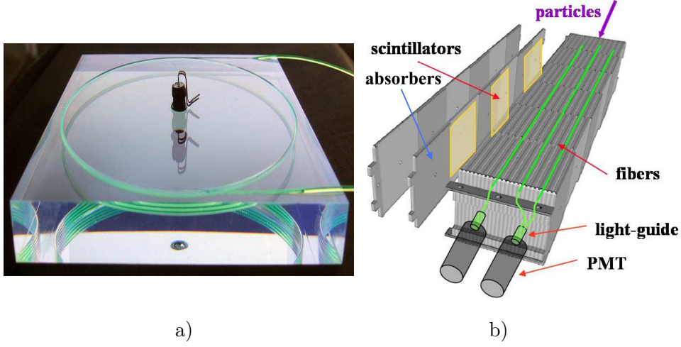
Figure 4.13.: Scintillator pad used in the SPD and PS (a). Schematic view of a HCAL cell showing the periodic absorber/scintillator design (b). Figures taken from Ref. [63].
