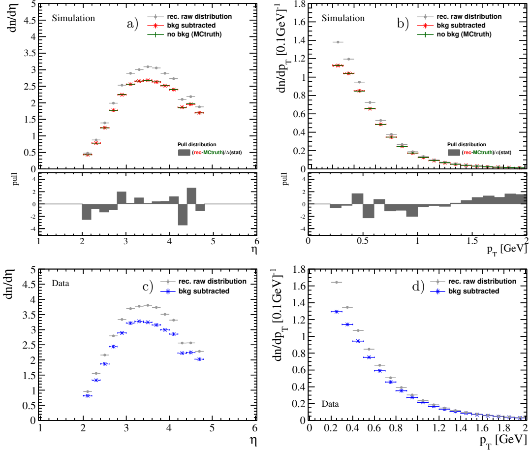
Figure 9.5.: Background correction applied to particle densities, dn/d\eta (left) and dn/dp_T (right). Simulated distributions (a,b) compare the raw track sample (grey), the same sample after applying purity weighting factors, and a sample free of background by using generator information. The corresponding pull distribution is given below. Data distributions (c,d) are compared w/ and w/o correction. All errors are statistical.
