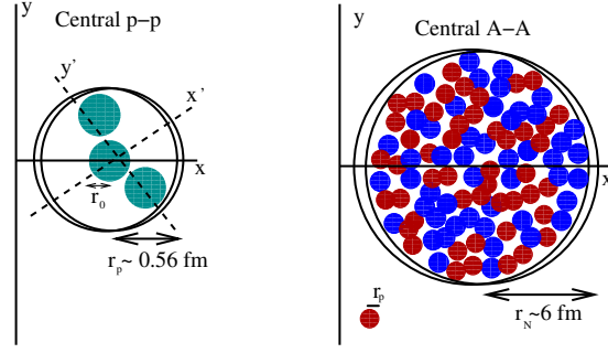
Figure 12.8.: Schematic view of the overlap region in pp (left) and nucleus-nucleus (right) collisions, displayed in the transverse plane. The coloured circles indicate hadronically active regions. Depending on the number and size of these regions, large eccentricities can result, even in central collisions. Figure taken from Ref. [156].
