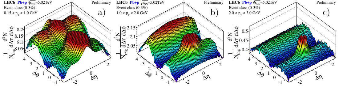
Figure 16.8.: Two-particle correlation functions for Pb+p data in the highest event-activity class using the high-occupancy data sample. Activity-classes are defined by using VELO-hit multiplicity. The near-side ridge appears to be present in all p_T -ranges at this multiplicity regime. In the low- p_T range (a) various structures are present in the correlations function, also a near-side ridge appears to be present. In the intermediate- (b) and high- p_T ranges (c) the near-side ridge is clearly visible.
