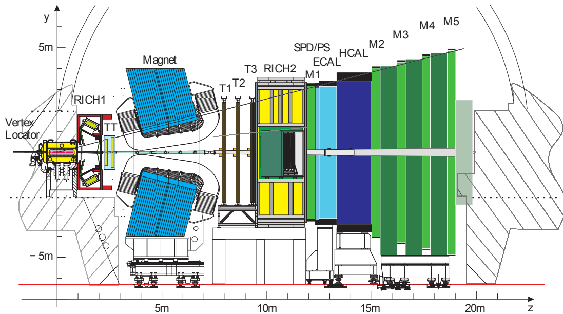
Figure 4.1.: Schematic overview of the LHCb detector in the y-z plane. The detector's subsystems are described in the text. Figure is taken from Ref. [63].
