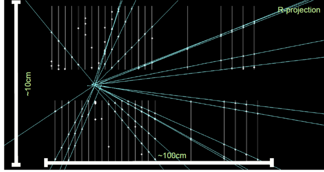
Figure 5.2.: The r - z -projection of reconstructed tracks in the VELO. As there is no magnetic field, all tracks are reconstructed as straight lines.
