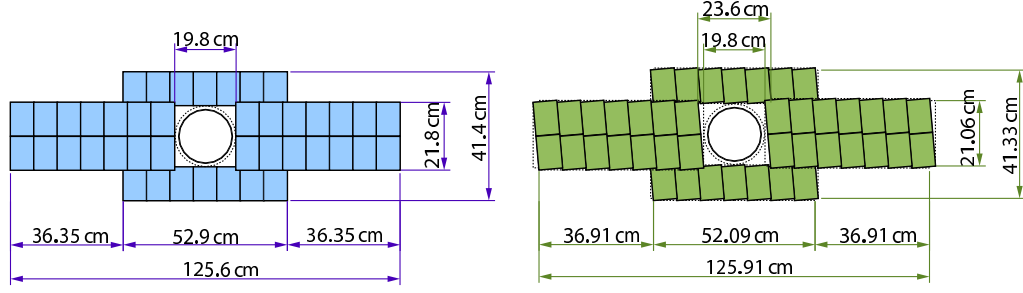
Figure 4.8.: Schematic view of x -layers (a) and stereo layers (b) in the Inner Tracker. Due to the deflection of charged particles by the magnetic field, there are more boxes in the bending plane compared to the non-bending plane. Figures taken from Ref. [74].
