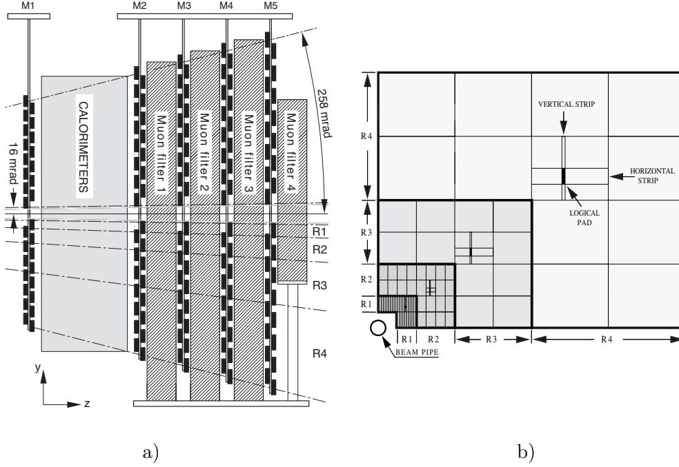
Figure 4.15.: Schematic view of the muon system. Layout of the five muons stations in side view (a). Front view of a quadrant showing the four regions of different granularity. Figures taken from Refs [63, 84].
