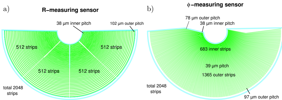
Figure 4.4.: Sketch of the VELO r - (a) and \phi - (b) sensors. Note the increasing pitch size when going towards greater radii, and the kink in the strips of the \phi -sensor. Figures are taken from Ref. [67].
