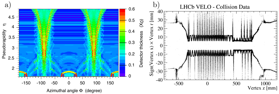
Figure 4.6.: a) Average radiation length seen by particles passing through the VELO as function of \eta and \phi . b) Reconstructed vertices of hadronic interactions in VELO material as function of z and radius \pm r (left/right of beam). Figures are taken from Refs [63, 72].
