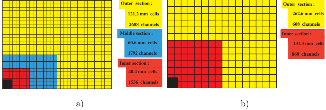
Figure 4.14.: Granularity of the calorimeter system showing one quarter of the detectors in front view. Three cell sizes are adopted for the SPD, PS and ECAL (a), the HCAL is divided into two regions. The position of the beam pipe is indicated in black. Figures are taken from Ref. [63].
