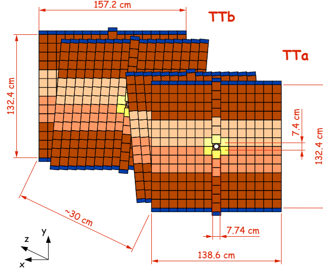
Figure 4.7.: Schematic view of the Tracker Turicensis. The x -layers are aligned straight, the stereo layers are tilted by 5^\circ . Different read-out sectors are indicated by different shadings, the electronics are marked in blue. Figure taken from Ref. [74].
