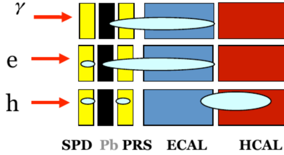
Figure 4.12.: Schematic view of the different signatures of photons, electrons and hadron in the components of the LHCb calorimeter system. Figures taken from Ref. [83].
