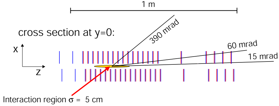
Figure 4.5.: Layout of VELO modules along the z -axis in top view. r -sensors are marked in blue, \phi -sensors in red. Figure is taken from Ref. [67].
