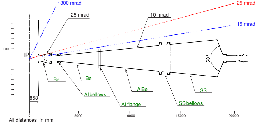
Figure 4.10.: Layout of the beam pipe in the LHCb coordinate system. The blue dotted lines indicate the borders of the main tracking system. The red dotted line marks the specific angle with which particles have to traverse a greater amount of material, related to the first section of the beam pipe. The material of the beam pipe and the connectors is given in green. Original figure is taken from Ref. [68].
