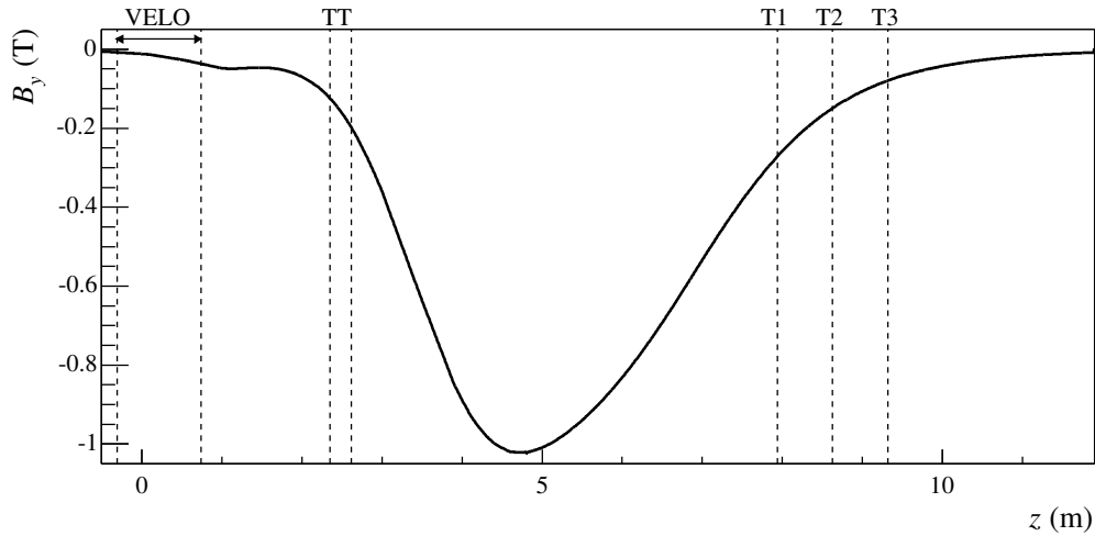
Figure 4.3.: The main component of the magnetic field strength as function of z . The position of the tracking detectors is indicated by dashed lines. Figure taken from Ref. [70].
