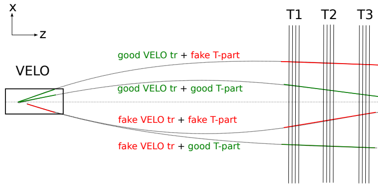
Figure 5.4.: Sketch visualising a good and fake long-tracks, consisting of different VELO and a T-station parts. Most of the fake tracks are made of good VELO track matched to a fake T-part that is build of random hits or hits induced by hadronic showers. Also combination based on fake VELO tracks are possible but less likely.
