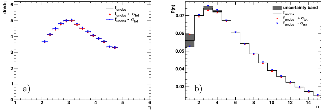
Figure 10.8.: Effect of varying f_{\text{unobs}} within its systematic uncertainty range. a) Particle density dn/d\eta , b) multiplicity distribution in the total kinematic range, showing only multiplicities from 1-15 particles.
