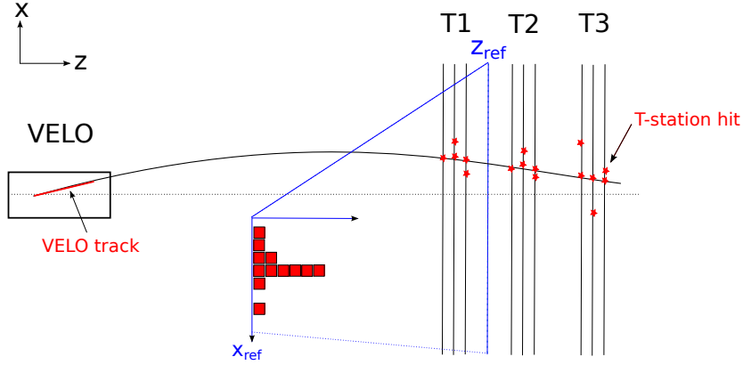
Figure 5.3.: Sketch visualising the forward tracking. A VELO track is extrapolated into the T-stations (T1-T3). Each of the found T-station hits is used to form a combined VELO-T-track. The T-hit is projected along the extrapolation onto a reference plane at z = z_{\text{ref}} . Common hits that belong to a track will cluster while unrelated hits are distributed randomly.
