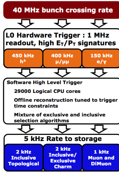
Figure 4.16.: Overview of the LHCb trigger scheme, by using the example of the 2012 configuration. Figure is taken from Ref. [58].
