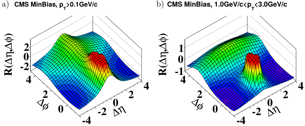
Figure 12.4.: Two-particle correlations in minimum-bias pp collisions at 7 TeV centre-of-mass energy, measured by CMS. In (a) all particles with an inclusive p_T -range of p_T > 0.1 GeV are considered, in (b) only particles in the range of 1 < p_T < 3 GeV are selected. Figures are taken from Ref. [7].
