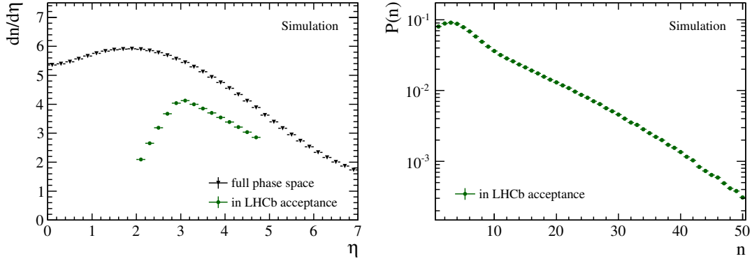
Figure 6.1.: Exemplary distributions for charged particle densities as function of pseudorapidity, dn/d\eta , and charged particle multiplicities, P(n) , in simulated pp collisions at \sqrt{s} = 7 TeV. a) The dn/d\eta distributions shows results for the entire phase space (no kinematic constraints) and for particles within the accessible kinematic range of the LHCb detector ( p > 2 GeV, p_T > 0.2 GeV, 2.0 < \eta < 4.8 ). b) Multiplicity distribution for charged particles within the full LHCb acceptance.
