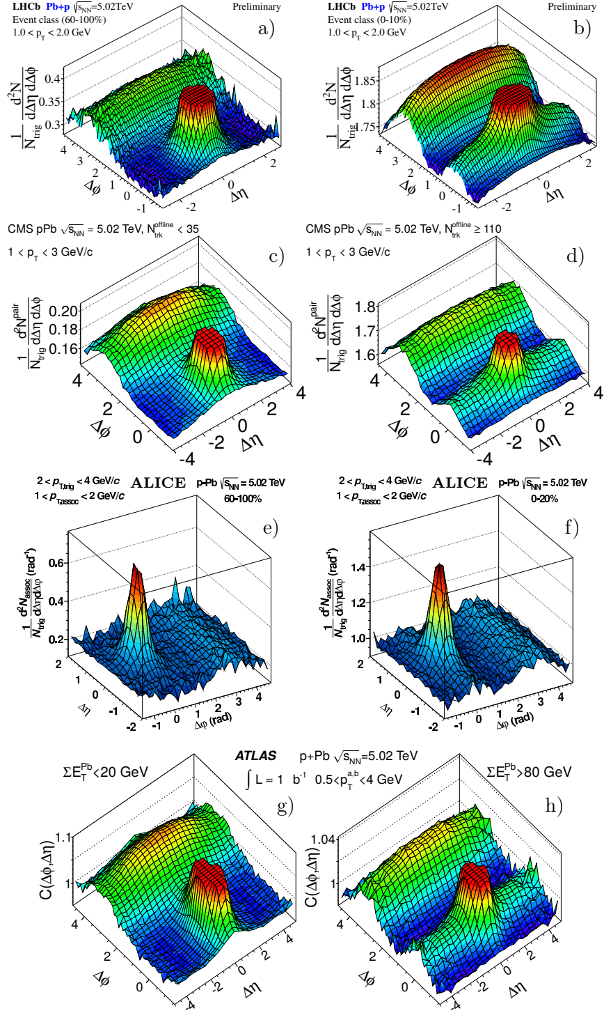
Figure 16.9.: Comparison of two-particle correlations in proton-ion collisions at \sqrt{s_{NN}} = 5.02 TeV among the four big LHC experiments. Results are presented for events with low (left) and high (right) event-activity, more details see text. LHCb results (a-b) in Pb+p configuration probing the forward region, \eta = [2.0, 4.9] ; CMS results [131] (c-d) probing the central region, |\eta| < [2.0] ; ALICE results [183] (e-f) probing the central region, |\eta| < [1.2] ; ATLAS results [182] (g-h) also probing the central region, |\eta| < [2.5] . Figures taken from respective reference.
