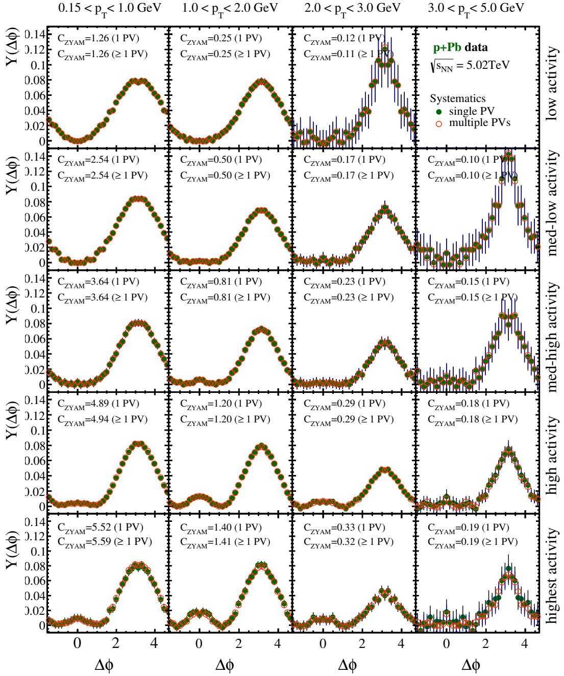
Figure 17.7.: One-dimensional correlation yield as a function of \Delta\phi for p +Pb collision at \sqrt{s_{NN}} = 5.02 TeV. Results are compared for selected events containing exactly 1 PV (nominal) and events containing \geq 1 PVs. The integration region is 2 < \Delta\eta < 2.8 , the final yield is subtracted by the constant listed in each panel using the ZYAM-method. All given errors are pure statistical.
