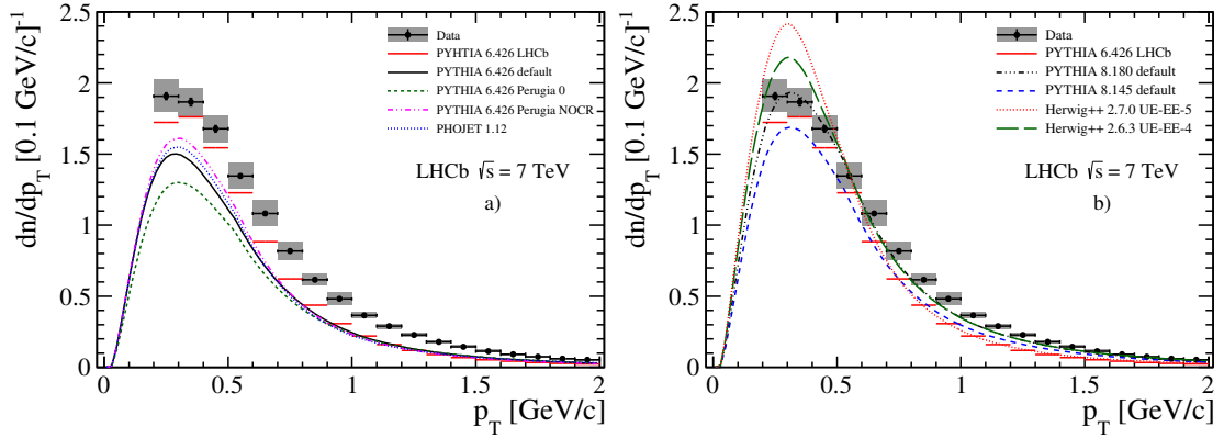
Figure 11.2.: Charged particle densities as a function of transverse momentum. The LHCb data are shown in points with statistical error bars (smaller than the marker size) and combined systematic and statistical uncertainties as the grey band. The measurement is compared to predictions of several Monte Carlo event generators.
