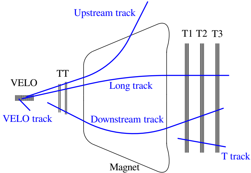
Figure 5.1.: Sketch of track types used in LHCb. Original figure taken from Ref. [97].
