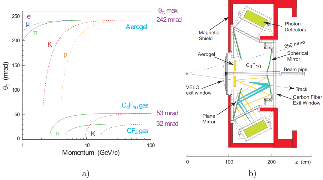
Figure 4.11.: Cherenkov angle as function of particle momentum for the RICH radiators (a). Schematic layout of RICH1 in side view (b). Figures taken from Ref. [63].
