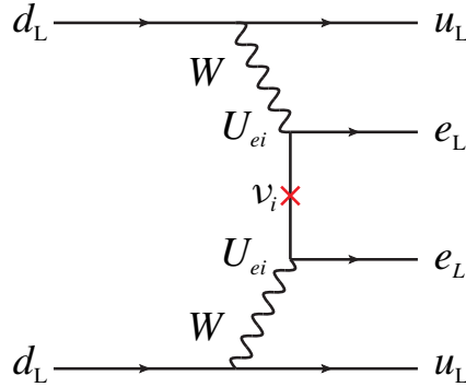
Figure 2.4: Neutrinoless double beta decay (at the constituent-quark level) mediated by neutrino exchange and charged-current interactions. The internal neutrino line implies a sum over all mass eigenstates \nu_i with mixing to the electron neutrino given by the mixing matrix elements U_{ei} .
