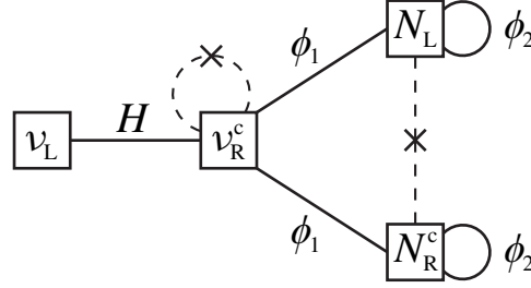
Figure 3.1: Schematic illustration of the allowed and forbidden neutrino mass terms, which yield the form of the neutrino mass matrix in the CISS. Solid lines indicate a gauge-invariant Yukawa coupling of the fields connected by that line and mediated by the scalar particle assigned to the line. The terms corresponding to dashed lines are gauge-invariant, too. However, they are not admissible in a conformal theory due to the lack of an adequate scalar degree of freedom that could induce the necessary Yukawa coupling.
