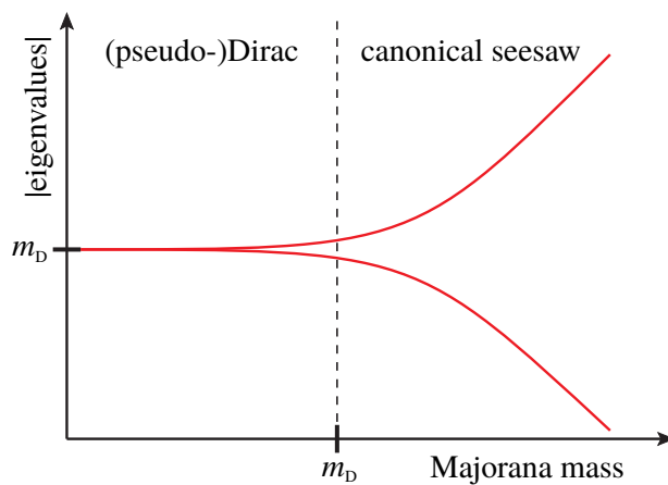
Figure 5.2: Schematic illustration of the evolution of a pair of eigenvalues with increasing Majorana mass (red lines) on a double-logarithmic plot. At a Majorana mass of about m_D the transition between the (pseudo-)Dirac and the seesaw regime takes place (dashed line).
