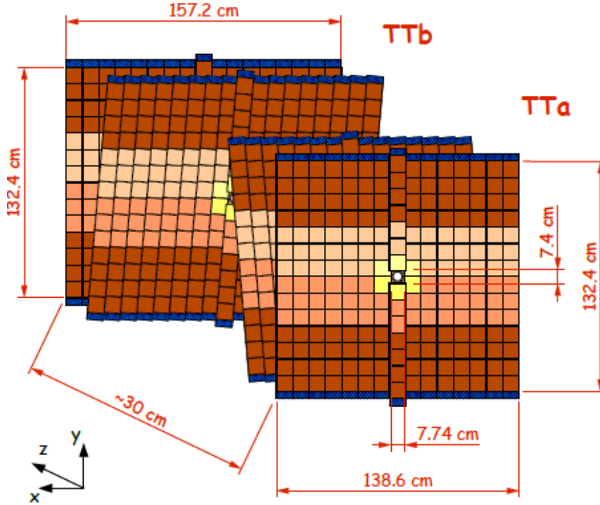
Figure 4.6.: Sketch of the geometry and length scale of the TT taken from [59].
