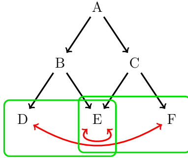
Figure 5.2: The order \leq and part of the relation \leftrightarrow on B \backslash G/H and the two minimal fat ideals.
