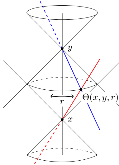
Figure 3.1: The parametrization \Theta interpreted by intersecting light cones in \mathrm{Lag}(\mathbb{R}^4) . The vertical line is the set of points \Theta(x, x, *) containing the limit set.
