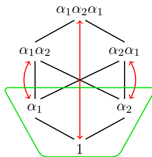
Figure 4.1: The Weyl group of SL(3, \mathbb{R}) . The black lines indicate the Bruhat order, in the sense that a line going downward from x to y means that x covers y in the Bruhat order. The red arrows show the involution induced by w_0 . The subset surrounded by the green box is the only balanced ideal.
