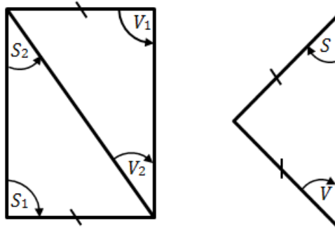
Figure 1.4.7: New coordinates on the block of type 3 (left) and on the block of type 4 (right)
