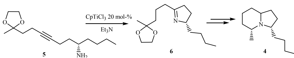
Scheme 3. The total synthesis of ( \pm )-monomorine ( 4 ) by Livinghouse et. al.
