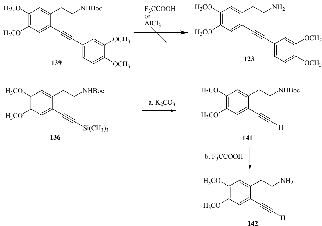
Scheme 30. Deprotection of Boc-group. Reagents and condition: a. \text{K}_2\text{CO}_3 0.1 equiv, MeOH, 25°C, 3 h, 88%; b. \text{F}_3\text{CCOOH} 6.5 equiv, \text{CH}_2\text{Cl}_2 , 25°C, 20 h, 86%.
