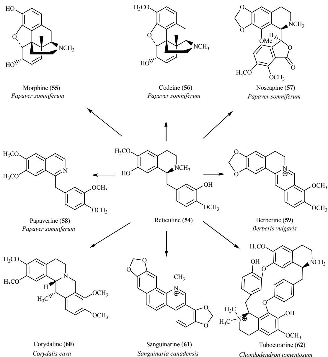
Scheme 12. Pharmaceutically useful alkaloid derivatives formed from the benzyloquinoline alkaloid ( S )-reticuline ( 54 ).
