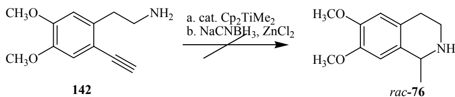
Scheme 47. Attempts to synthesize salsolidine ( 76 ) using a Ti-catalyzed hydroamination.
