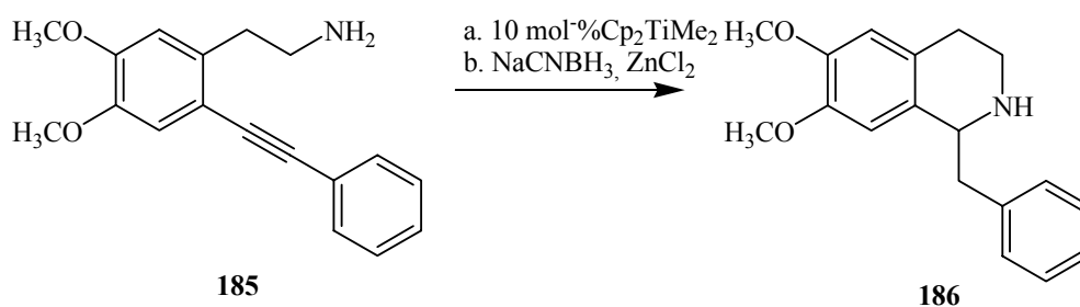
Scheme 46. Synthesis of tetrahydrobenzylisoquinoline 186 . Reagents and conditions: a. 10 mol-% \text{Cp}_2\text{TiMe}_2 , toluene, 110^\circ\text{C} , 16 h; b. \text{NaCNBH}_3 2.0 equiv, \text{ZnCl}_2 1.0 equiv, MeOH, 25^\circ\text{C} , 20 h, 82% (two steps).
