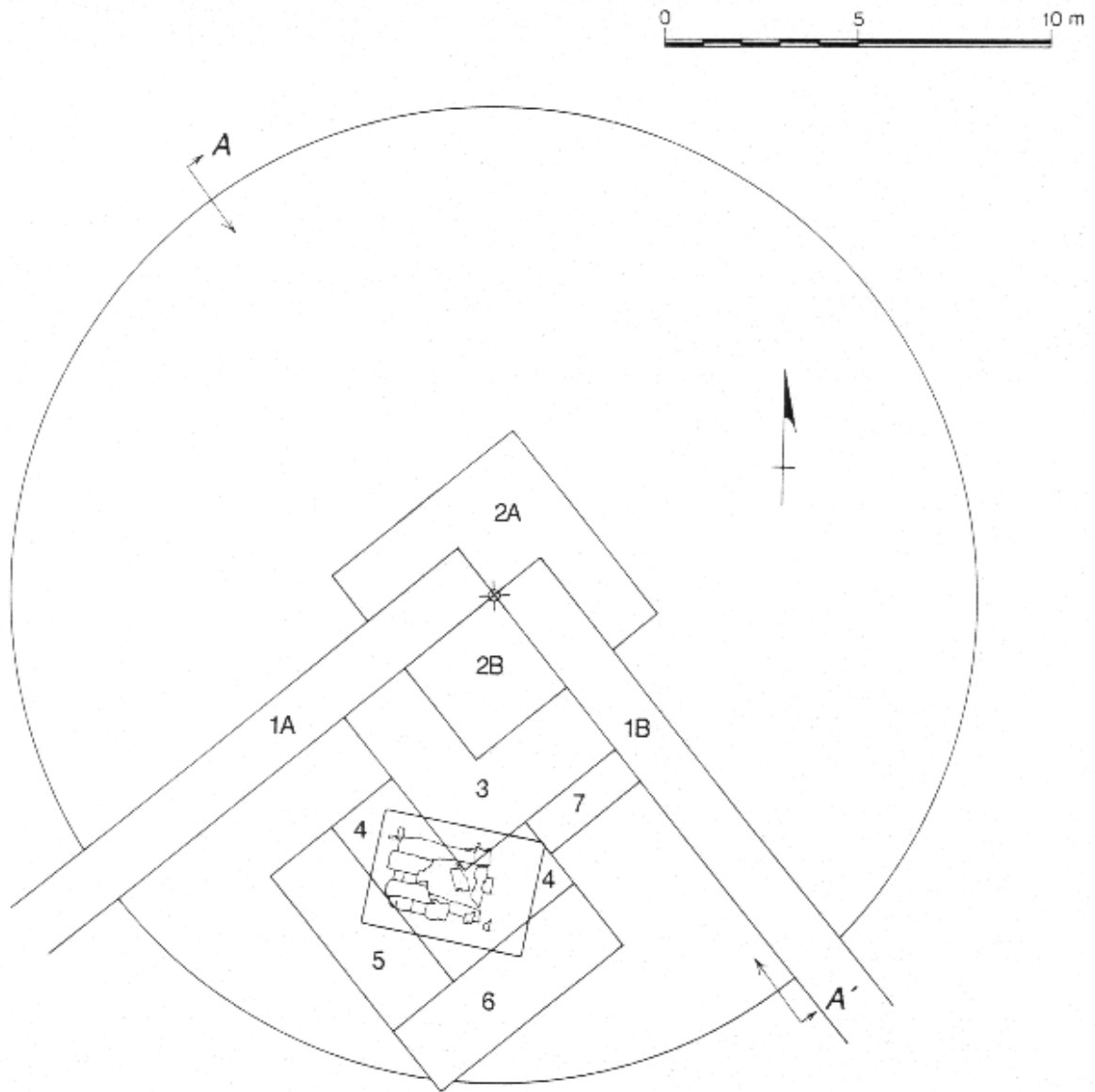
Abb.1 Tumulus G, Plan
