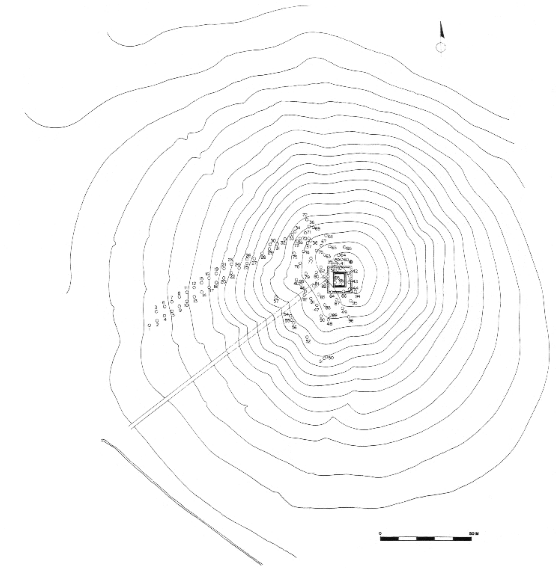
Abb.1 Tumulus MM, Plan
