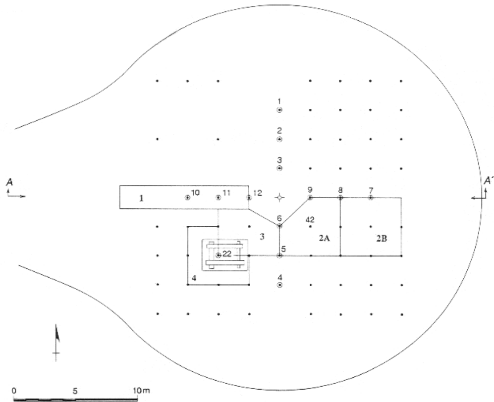
Abb.2 Tumulus N, Plan
