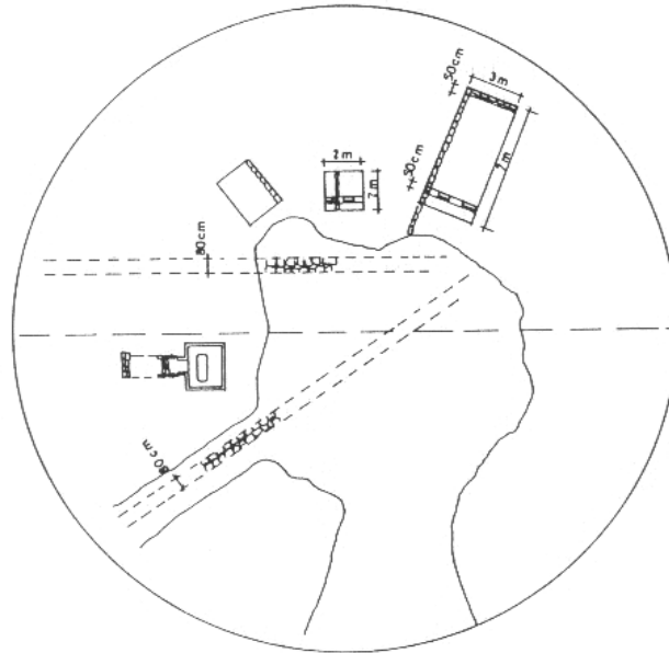
Abb.1 Tumulus Basmacitepe, Plan
