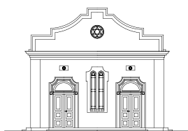
FIG. 280. Pribeník, Synagogue, South and West Façades.
