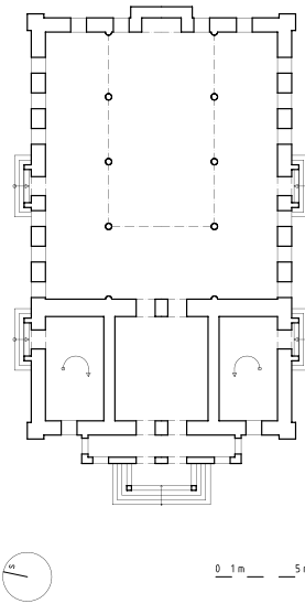
FIG. 476. Humenné, Old Synagogue, North and West Façade (Museum of Jewish Culture, Bratislava). FIG. 477. Humenné, Old Synagogue, Plan.
