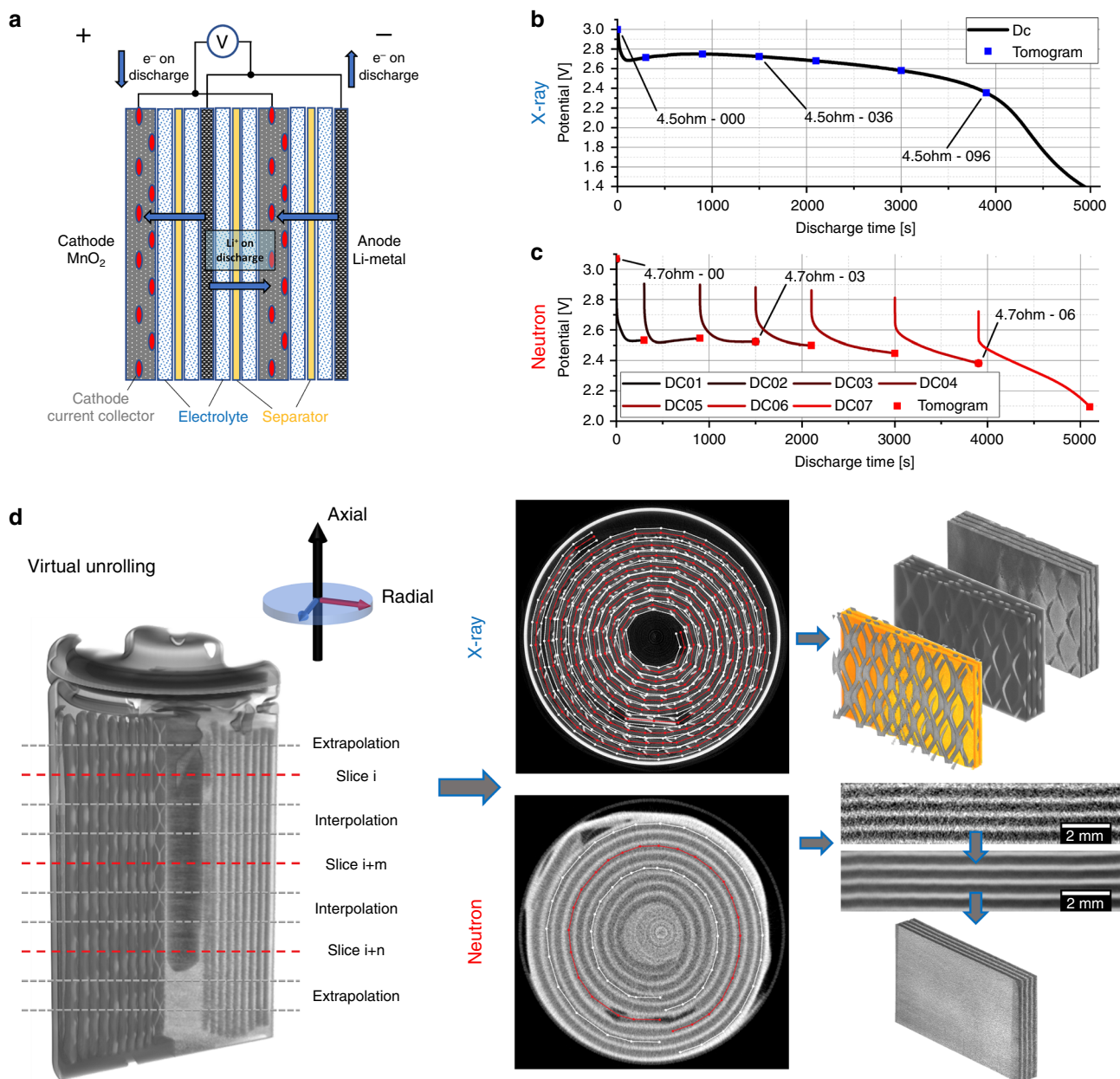
Fig. 1 Illustration of the cell operation, discharge curves and virtual unrolling technique. Image a shows an illustration of the studied Li/MnO 2 CR2 primary cell from Duracell. Graph b shows the constant resistance discharge curve for the CR2 cell over 4.5 Ω, where simultaneous fast X-ray CT was carried out. Graph c shows the constant resistance discharge curve over 4.7 Ω, where the discharge was interrupted for each neutron tomography after a certain time interval. Image d displays the reconstructed tomograms from neutron and X-ray CT along with examples of sections extracted following virtual unrolling of the reconstructions. Clearly visible in the X-ray images is the nickel current collecting mesh, which appears brighter than the Li x MnO 2 active electrode material.
