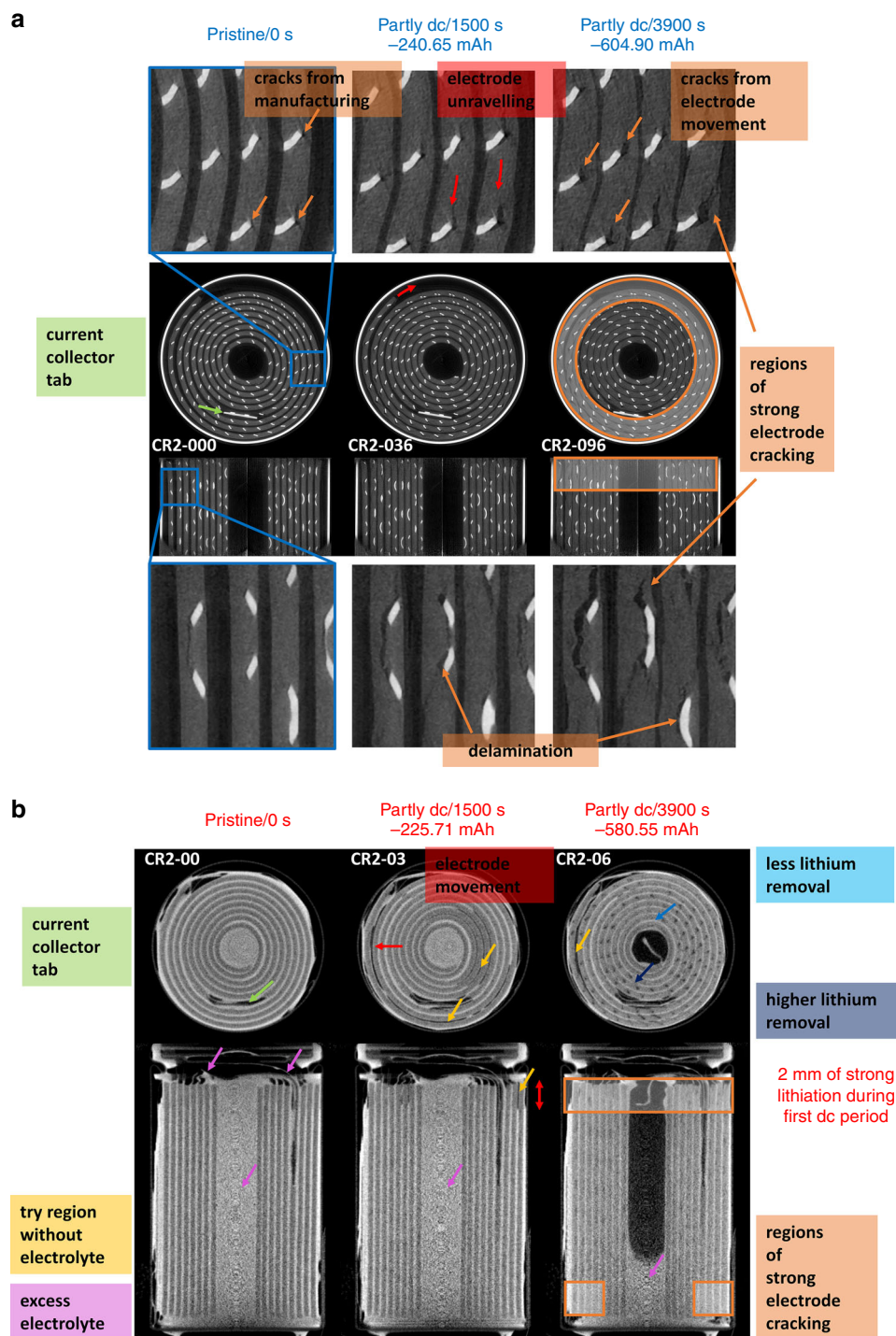
Fig. 2 3D reconstructed operando X-ray and in situ neutron tomograms. a shows horizontal and vertical orthogonal slices out of the X-ray tomograms. In total, 103 tomograms were recorded labelled from CR2-000 to CR2-102. One tomogram was recorded every 40 s with a total acquisition period of 2.8 s. Here the pristine state and two partly discharged states are presented. The images show the cracking and volume expansion of the \text{MnO}_2 electrode during cell discharging. The highly absorbing steel casing is visible as very bright ring around the wounded membrane–electrode ensemble. The contrast was optimised in order to improve the contrast within the lower attenuating components. b shows orthogonal slices of the neutron tomogram captured during the discharge over a 4.7\ \Omega resistor, where the lithium electrode and the excess of electrolyte in the middle of the cell are clearly visible. Lithium intercalation and electrolyte consumption are observed, as well as electrode cracking and electrolyte consumption. In total, eight neutron tomograms were collected with an acquisition period of about 8 h. The discharging process was interrupted for each tomogram and labelled with CR2-00 from the pristine to CR2-07, the fully discharged SoC.
