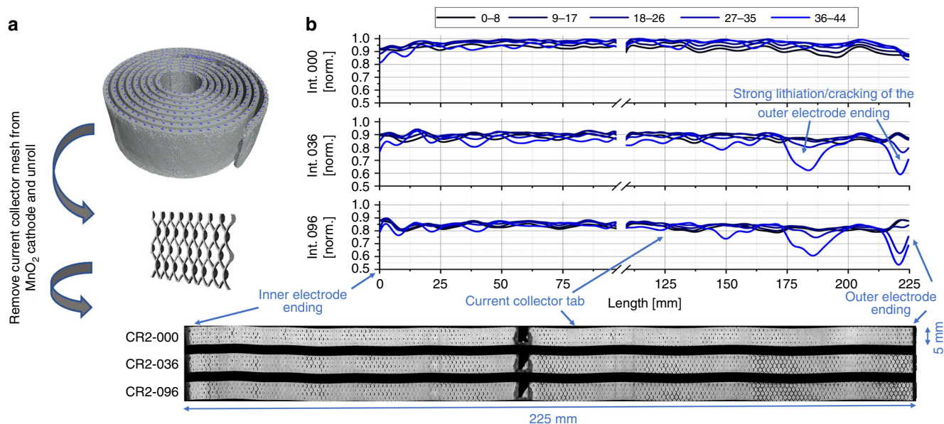
Fig. 5 Lithium distribution at various depths of the \text{Li}_x\text{MnO}_2 electrode during discharging, using unrolled X-ray tomography data of the upper part of a CR2 cell. For the analysis of the lithium distribution over the \text{MnO}_2 electrode thickness, a the current metal collector mesh is digitally removed before the electrode is unrolled. The electrode thickness is divided into five depths and the normalised grey values plotted over the electrode lengths. b represents the changed lithium distribution for the tomograms CR2-000, CR2-036 and CR2-096. The lithium content or cracking increases much more on the outer electrode side (blue) compared to the inner side and the electrode outer ending, as indicated by the reduced grey values. The lithium content is highest at the side of the current collector tab, exhibiting sinusoidal variation with increasing amplitude as the cell discharges.
