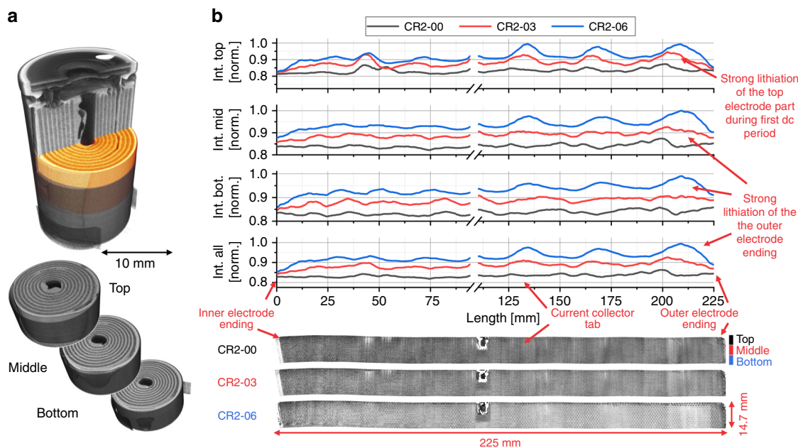
Fig. 6 Organisation of electrode unrolling (top, middle, bottom) and analysis of the lithium distribution in the \text{Li}_x\text{MnO}_2 electrode during discharging using neutron tomography data. The analysis of the lithium intercalation in the \text{Li}_x\text{MnO}_2 electrode is divided in four sections, the top, middle, bottom and overall part. a shows the pristine neutron tomogram divided in the studied parts. b displays the unrolled and over the thickness averaged electrodes of the pristine (CR2-00), partly discharged to -225.71\text{ mAh} (CR2-03) and partly discharged to -580.55\text{ mAh} (CR2-06) SoC and the related line plots. The intensity increase, due to the lithium intercalation, during discharging is clearly visible. On the top, the electrode undergoes a very strong lithiation during the first period of discharging. Over the electrode length, a sinusoidal intensity profile with increasing period is observed, with maxima at the tab side. This structure is caused by a higher lithium content on that side.
