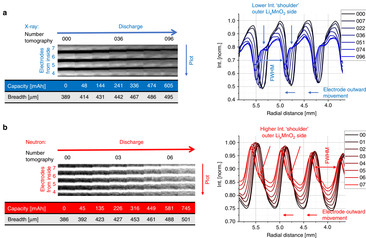
Fig. 3 Cathode thickness and intensity change during discharging. a shows cut-outs of virtual unrolled multilayer sections of the measured X-ray tomograms at different SoC from the pristine state (000) to the partly discharged state (096) to -604.90 mAh. The thickness increases of the \text{Li}_x\text{MnO}_2 electrode, during the discharge, is about 27% measured by the full-width at half-maximum (FWHM). The intensity plot shows a higher lithium intercalation in the cell outward electrode side by a lower intensity 'shoulder'. b shows a similar behaviour for the discharged cell imaged by neutrons. The electrode swelling is about 30% for a cell discharge to -745.08 mAh (07) and 26.5% to 580.55 mAh (06), which shows a similar electrode expansion as for the X-ray tomograms due to the similar discharge conditions. The plots illustrate the complementarity between X-rays and neutrons.
