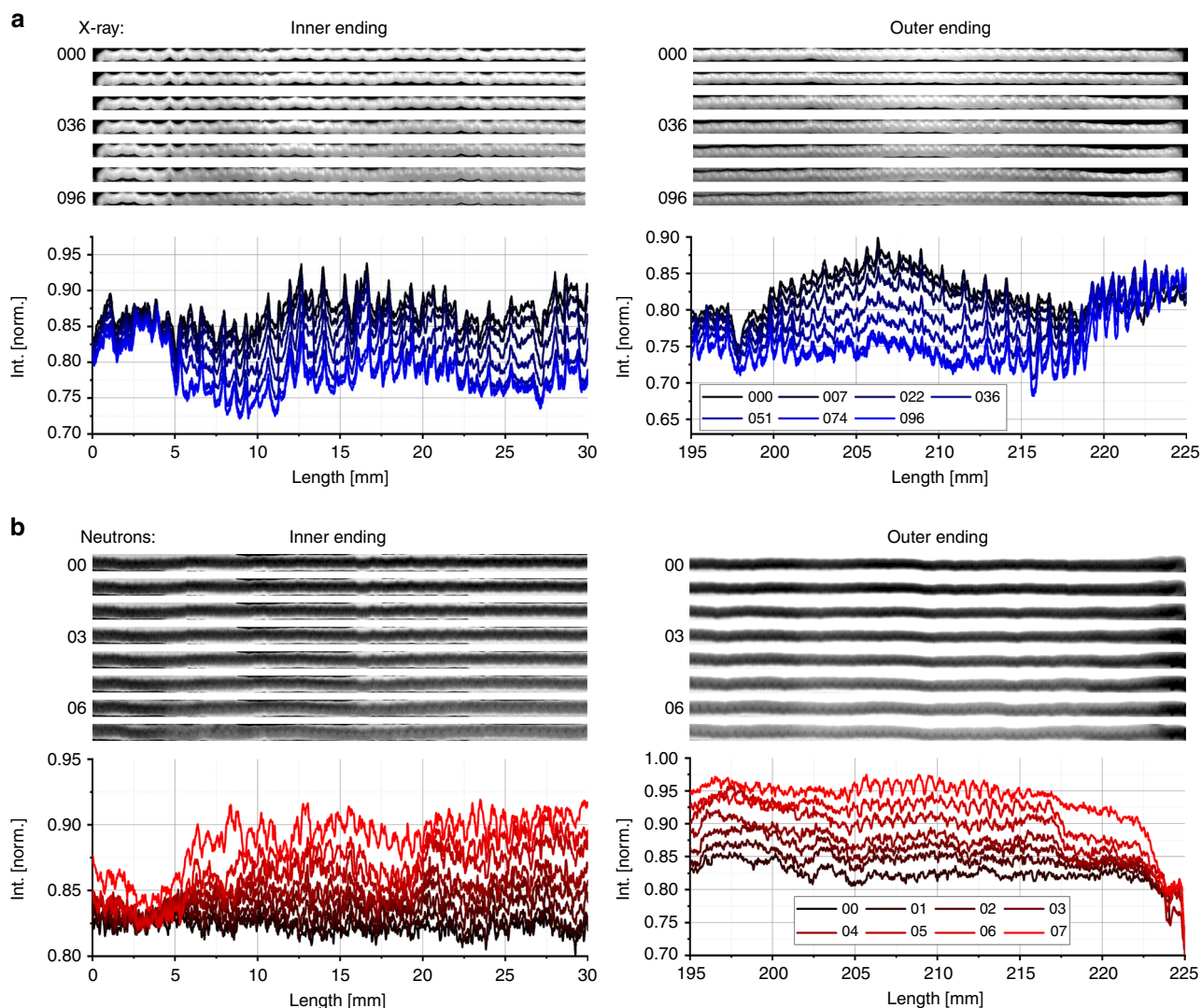
Fig. 7 Electrode endings and middle part at different SoC. The images and line plots in a , b show the attenuation of the \text{Li}_1\text{MnO}_2 electrode during cell discharging for the X-ray and neutron imaged cells, respectively. In both cases, the inner electrode parts show an almost homogeneous lithiation (not displayed here). The electrode endings do not show any lithiation activity for the X-ray scans and late start of lithiation in case of the outer electrode endings for the neutron scans.
