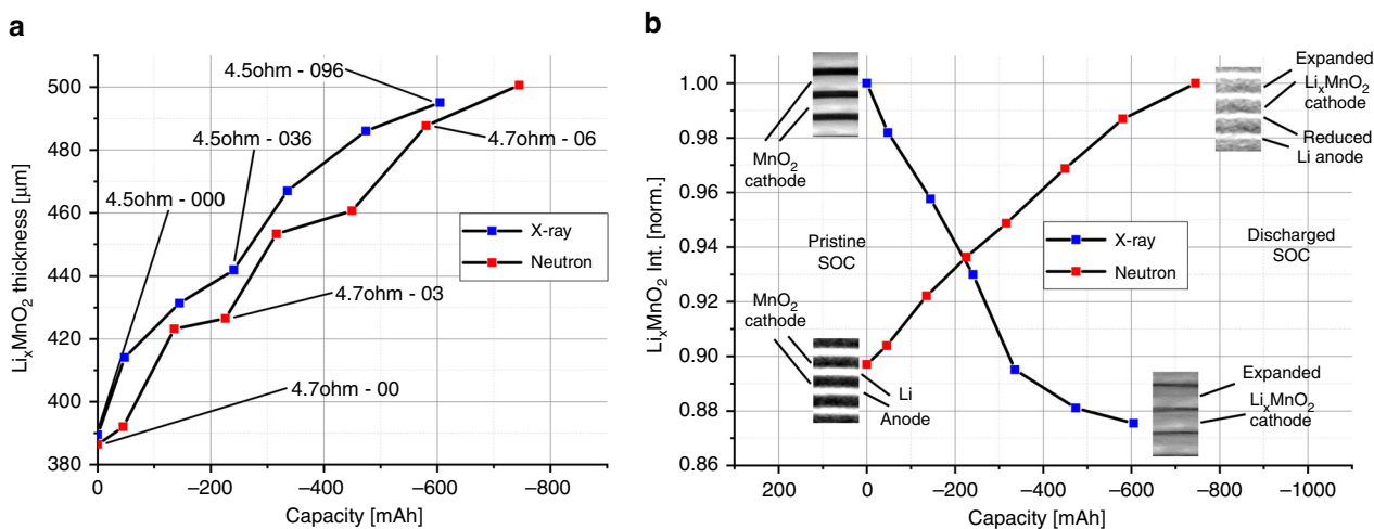
Fig. 4 Cathode thickness and intensity variation vs. capacity. Plot a shows the \text{Li}_x\text{MnO}_2 electrode thickness increase by the lithium intercalation during cell discharging by similar c-rates. For similar c-rates, the electrode thickness increases uniformly. But it seems that a slightly higher c-rate (blue) causes a higher increase in the volume expansion in comparison to lower c-rates (red). The graphs in b compare the intensity change of the \text{Li}_x\text{MnO}_2 electrode during discharging. The lithium intercalation process in the electrode causes an intensity decrease for X-rays and an increase for neutrons (for comparisons see Fig. 3).
