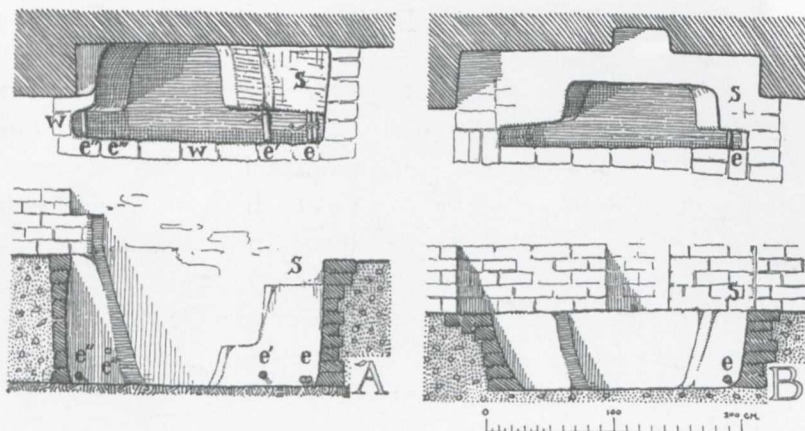
Fig. 2. Drawings of loom-pits found in the laura of Epiphanius: plan view and section through the middle. All loom-pits (also all those found outside the laura of Epiphanius) were located near walls. Pits are brick lined, from 60 to 100 cm deep, from 125 to 145 cm long, and 50 to 75 cm wide with a barrow slot alongside 200 cm in length and from 20 to 25 cm in width. The operator seat (S) is on the floor level (or very little below) at the right hand of the end of the pit (after The Monastery of Epiphanius , I, p. 69, fig. 25)
