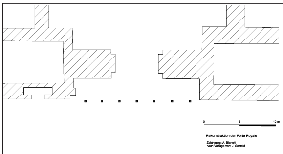
Fig. 6. Hall C: Schematic plan of the Porte Royale connecting Halls C and B as reconstructed by Jochen Schmid on the basis of the excavations by du Mesnil du Buisson 1924-1929 and the new excavations 1999-2005.
