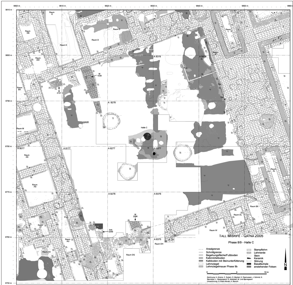
Fig. 5. Hall C: The foundations of the hall and the surrounding rooms on the basis of the excavations 1999-2005; foundations of the original planning phase (Phase 9b) are in grey and the modified foundation layout (Phase 9a) is in white.
