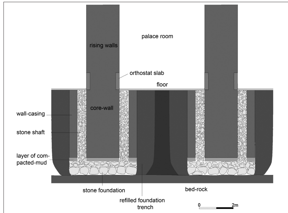
Fig. 7. The Royal Palace of Qatna: Schematic idealised section of a subterranean foundation wall of the palace with a 'couloir-type' stone alignment.
