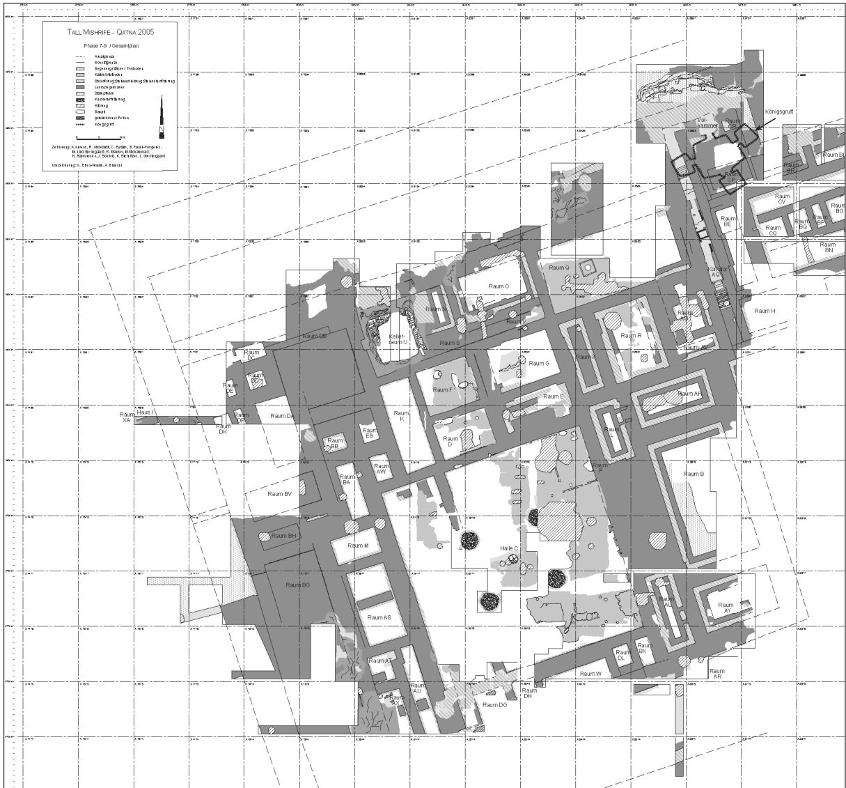
Fig. 2. The Royal Palace of Qatna: Plan of the structures excavated from 1999-2005 in Operation G by the German-Syrian team.
