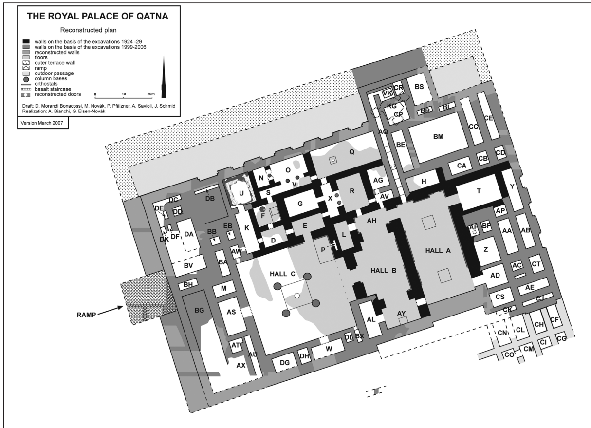
Fig. 16. The Royal Palace of Qatna: reconstructed floor plan (version of march 2007) based on the results of excavations in Operation G (after P. Pfälzner, M. Novák, J. Schmid), Operation H (after D. Morandi Bonacossi, A. Savioli) and Operation R (after M. al-Maqdissi), as well as on the plan by du Mesnil du Buisson (1935, Pl. XVI).
