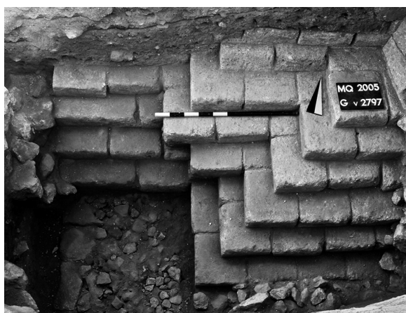
Fig. 14. Unfinished foundation wall of Phase G 9b below Hall C.
