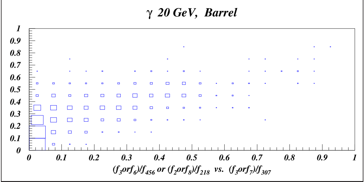
Figure 5.21: Correlation between the energy deposits in the hit cell's nearest \phi neighbour and its nearest \eta cell closest to the hit quadrant. For details see text. For cell numbering see Figure 5.13.
