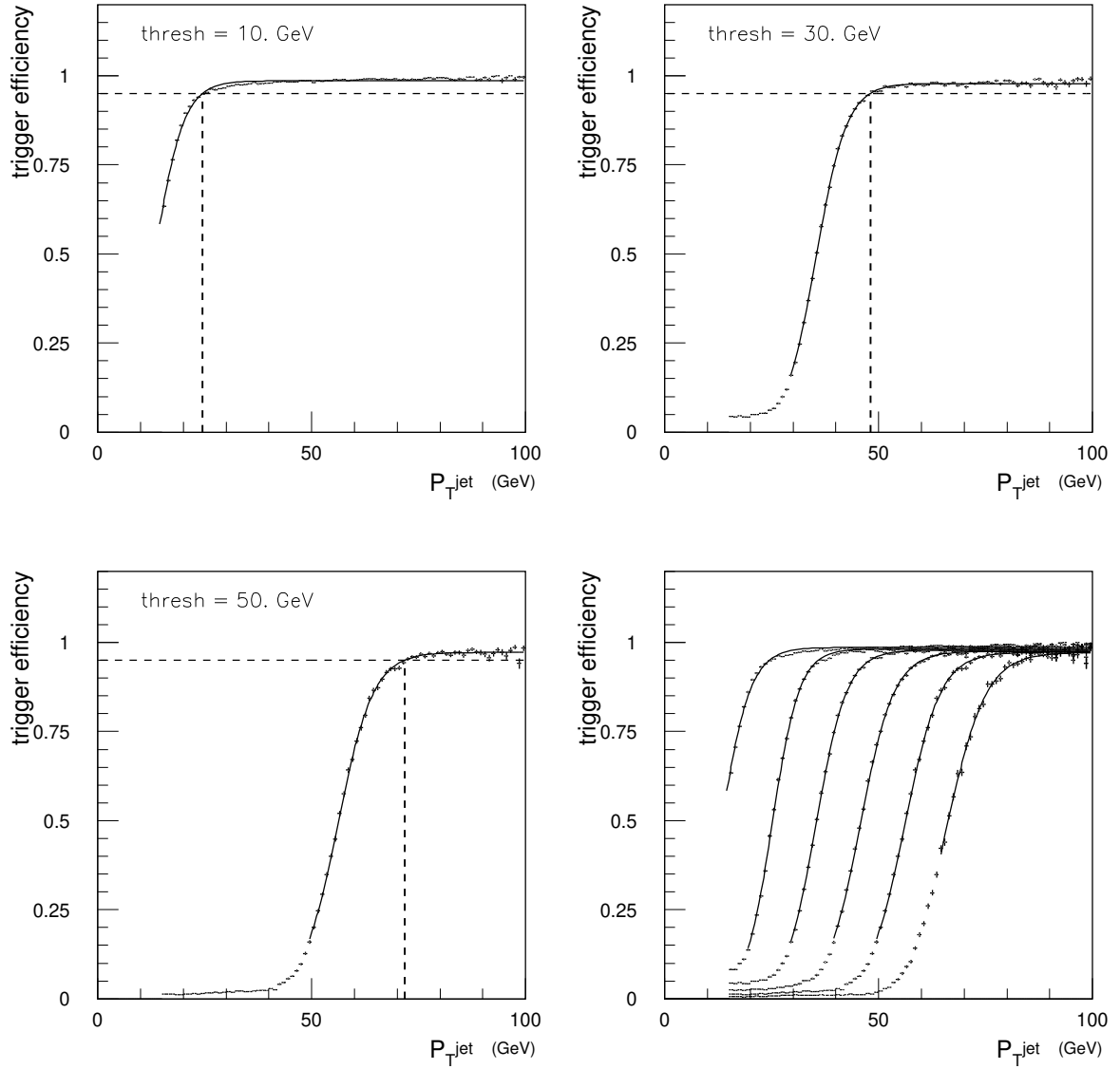
Figure 4.4: Examples of trigger efficiency curves for trigger cluster thresholds in the range 10 – 60 GeV in 10 GeV steps. The reference scale is the reconstructed jet energy of ATLFAS T using a cone algorithm with a radius of 0.7.
