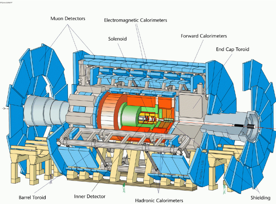
Figure 2.6: Overall layout of the ATLAS detector.
