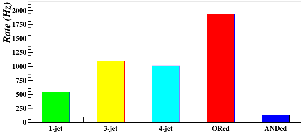
LVL1 calorimeter jet-trigger QCD background rate
