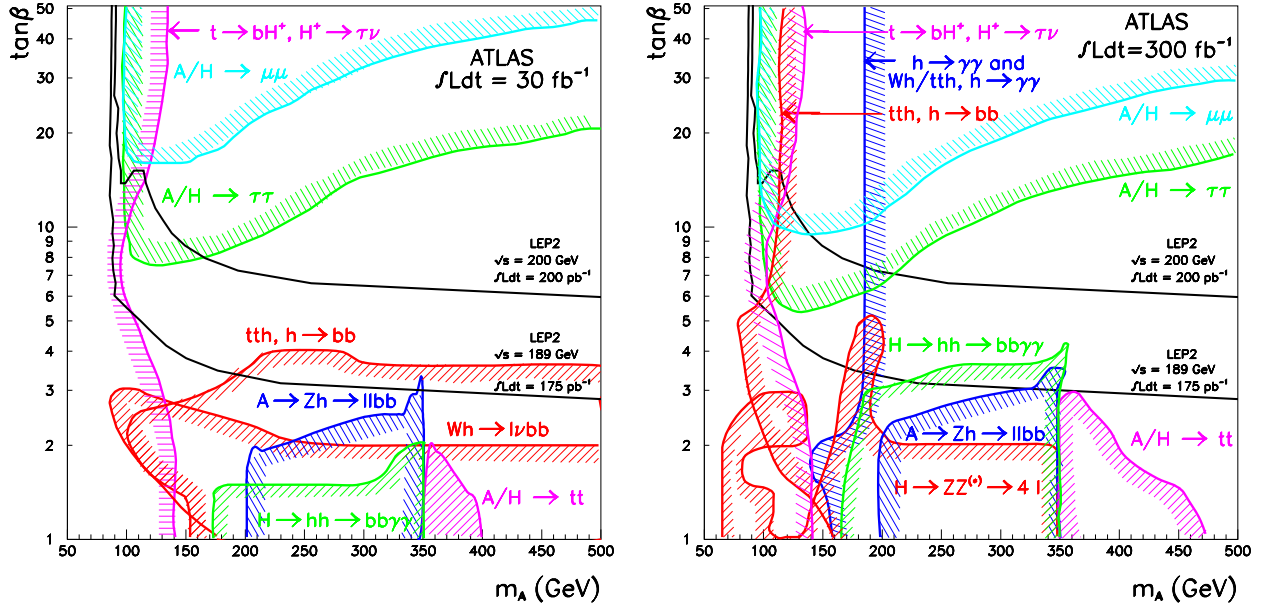
Figure 2.15: The discovery potential of the ATLAS experiment in the Higgs sector of the MSSM, in terms of the 5 \sigma discovery contours for different decay modes, in the usual (\tan\beta, m_A) parameter space for an integrated luminosity of 30 \text{ fb}^{-1} (left) and of 300 \text{ fb}^{-1} (right). The LEP2 limits corresponding to 175 \text{ pb}^{-1} and 200 \text{ pb}^{-1} integrated luminosities per experiment are also included. Taken from [46].
