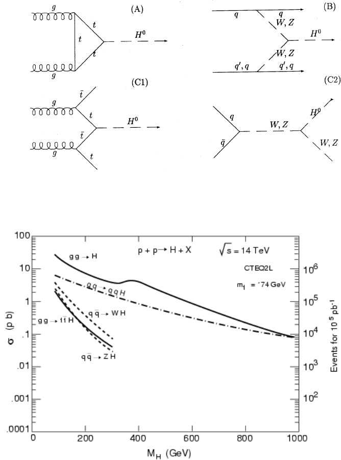
Figure 2.11: SM Higgs production cross-sections (y-axis on the left) for the different production mechanisms as a function of the Higgs boson mass. The corresponding number of events for an integrated luminosity of 100 \text{ fb}^{-1} is also indicated (y-axis on the right). Taken from [73].
