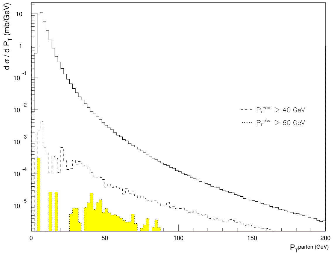
Figure 4.3: The P_T spectrum of the leading parton of the generated QCD jet events. The fraction of events accepted passing various E_T^{\text{miss}} thresholds is indicated by the dashed curves.
