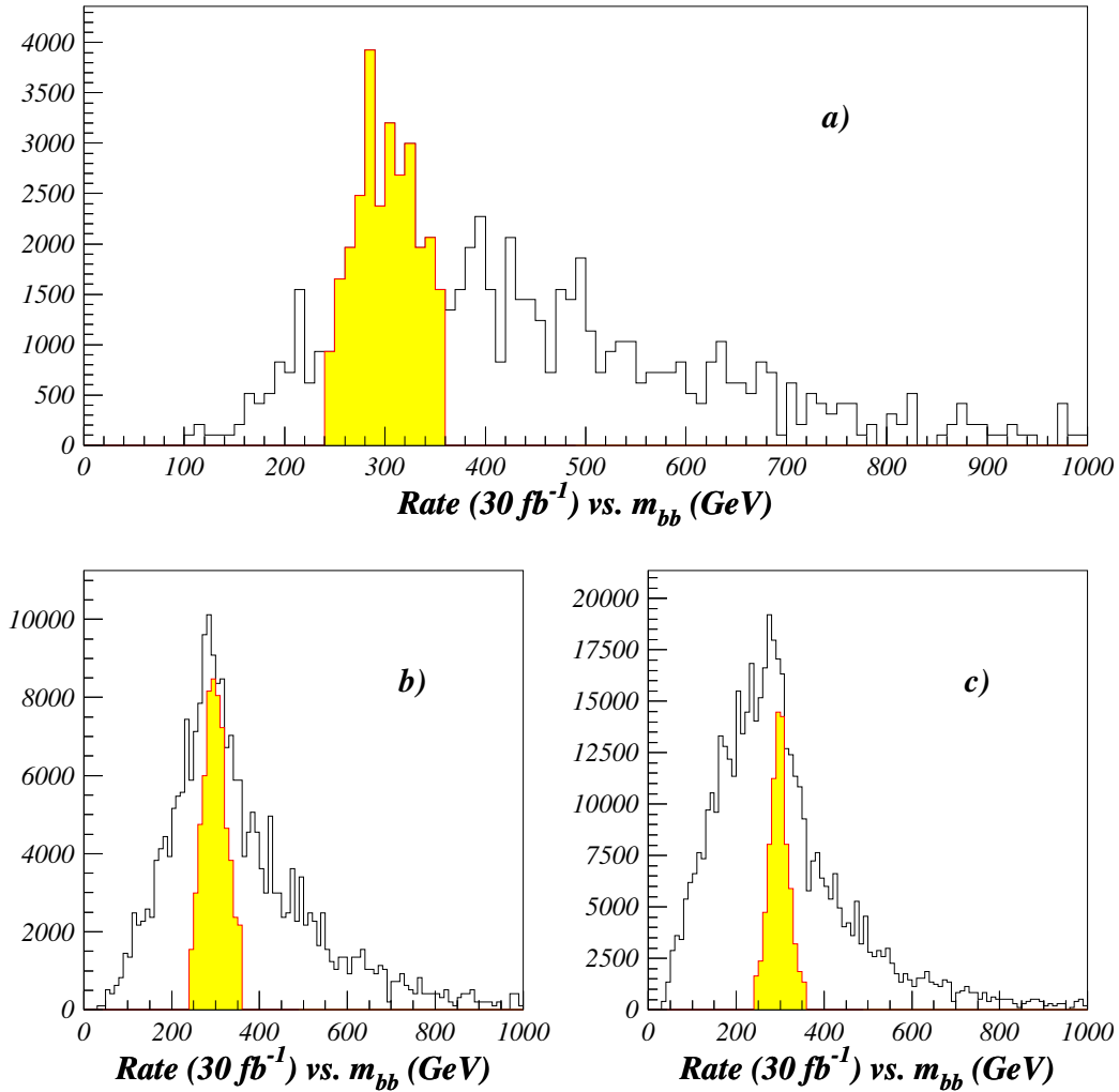
Figure 7.25: The m_{bb} distributions for m_H = 300 \text{ GeV} for an integrated luminosity of 30 \text{ fb}^{-1} . Only events with four leading jets tagged as b-jets and passing the geometrical/kinematical cuts contribute to the distributions. The invariant m_{bb} is reconstructed by using: a) only the two leading b-tagged jets (the tight cut), b) all bb combinations within the three leading ones, c) all bb combinations within the four b-tagged jets. The entries in the shaded histograms superimposed on the plots correspond to the accepted events with an entry within the applied mass window, and serve only to illustrate: 1) the position and width of the applied mass window and 2) the rate of accepted events. For an explanation of the various selection criteria see text.
