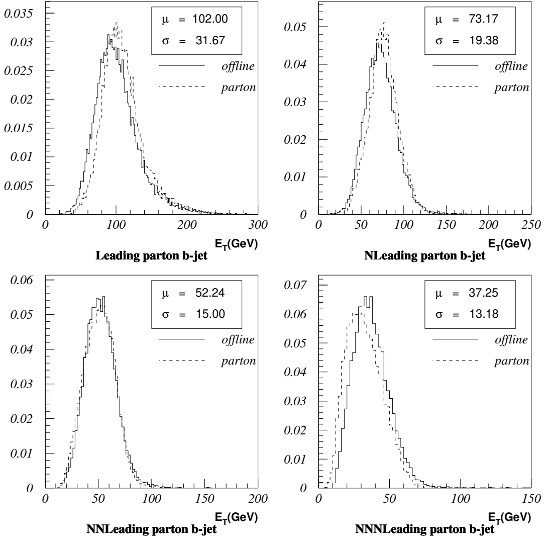
Figure 7.11: The E_T distribution of the parton b -jets and the corresponding recalibrated offline b -labeled jets, produced in the h h \rightarrow b\bar{b} b\bar{b} decay, ordered in E_T . The distributions correspond to the \tan \beta = 1.5 case (at low luminosity). In the labeling on the plots "N" stands for "Next-to".
