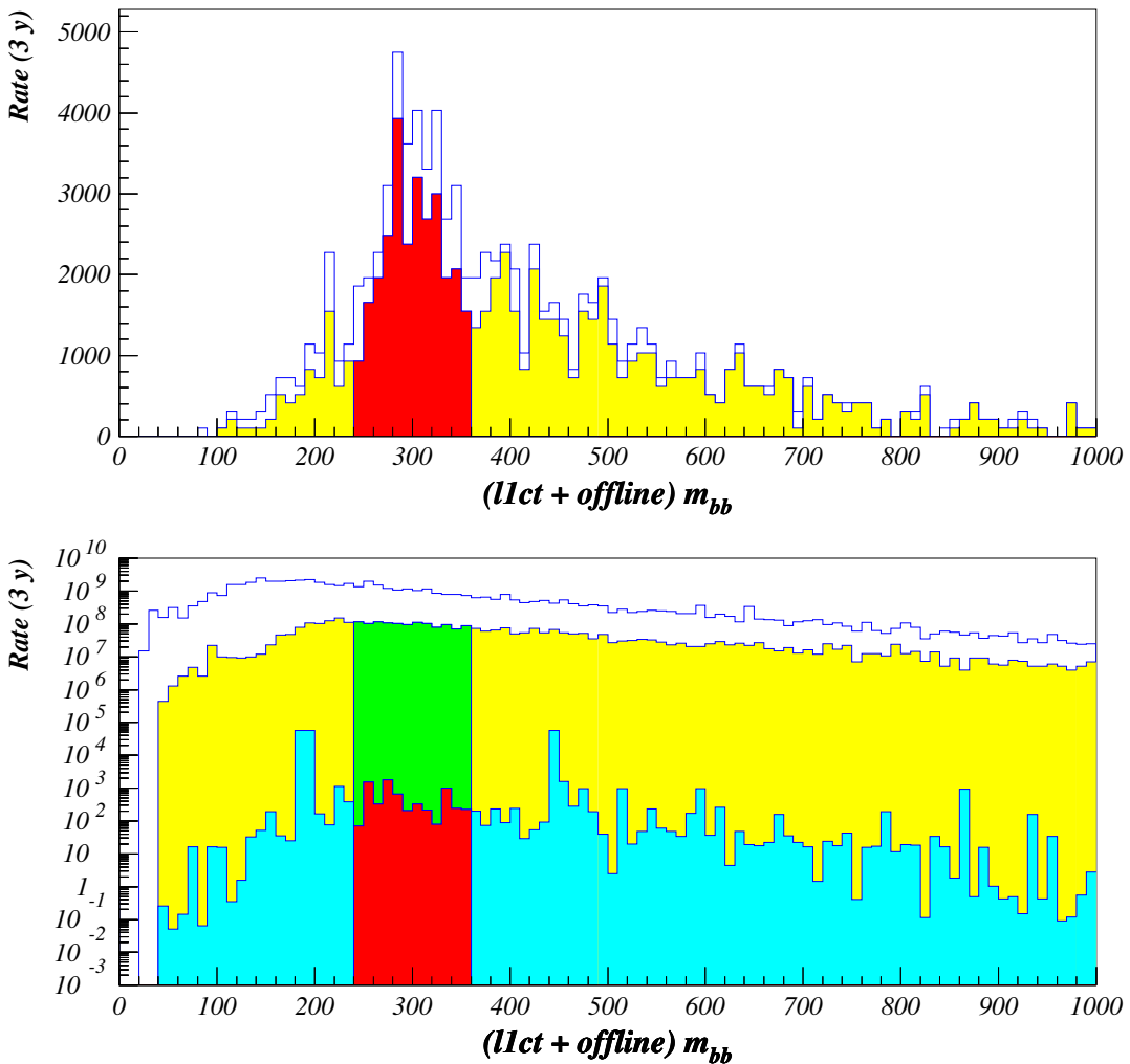
Figure 7.28: The Signal and background m_{bb} distributions for \tan \beta = 30 and m_H = 300 \text{ GeV} for an integrated luminosity of 30 \text{ fb}^{-1} for the tight selection algorithm after the LVL1 trigger. For details see text.
