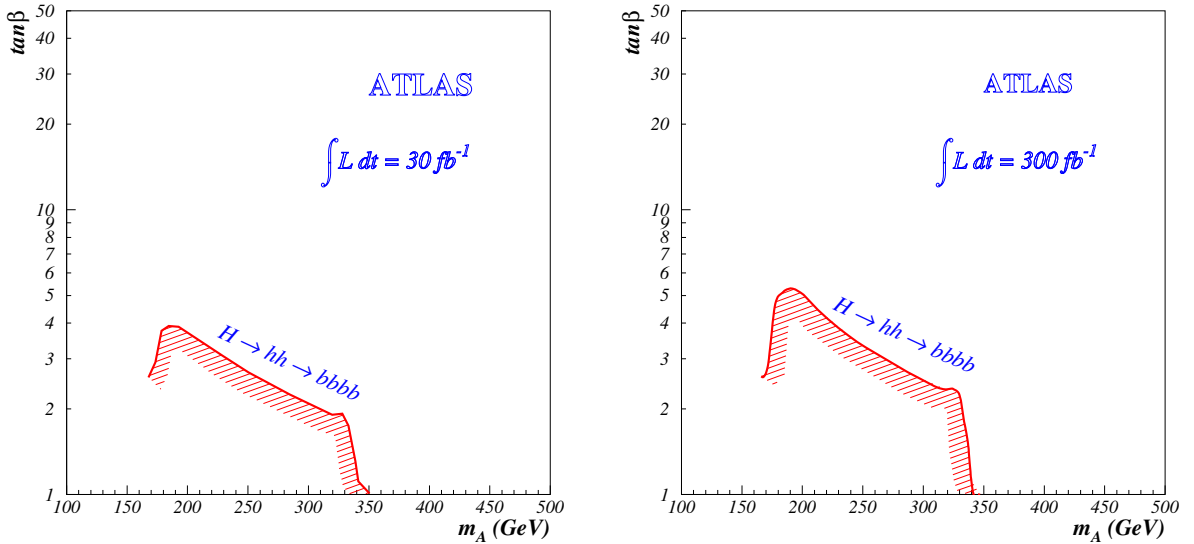
Figure 7.17: The 5\sigma discovery contours for low (left) and high (high) luminosities for the decay channel studied in this section.
