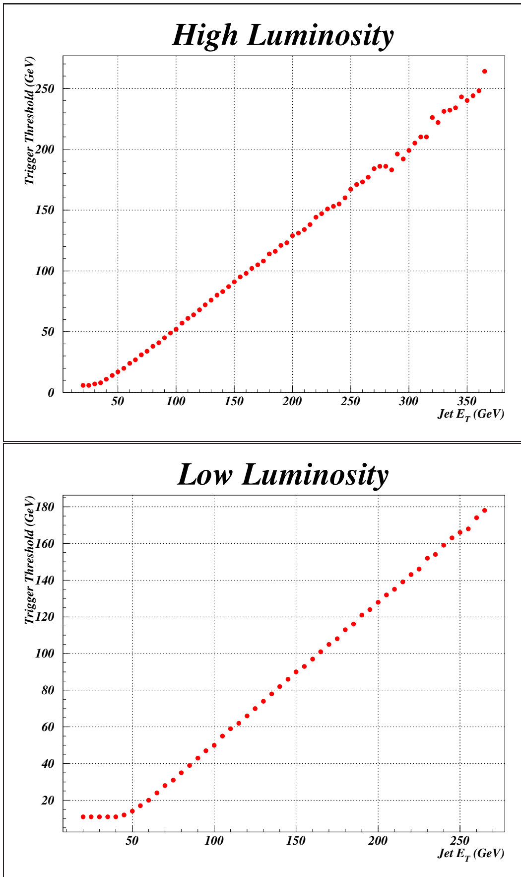
Figure 6.7: Inclusive (or single) jet trigger threshold curves as a function of the offline jets for 90% efficiency at high and low luminosities.
