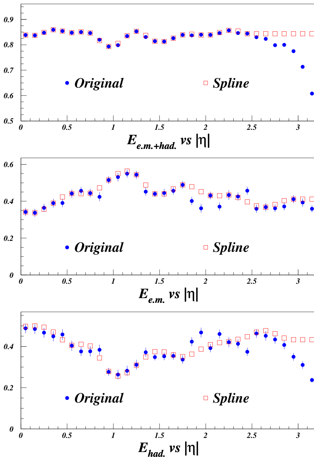
Figure 5.11: \eta scan of the response of the calorimeters to 30 GeV \pi^+ , the filled bullets labeled as original, showing different effects, like the depth of the calorimeters and the feed-through/transition region etc. . The empty boxes on the upper two plots show parametric (cubic) spline fits to describe the data points. These two functions are used to derive the response superimposed on the lower plot.
