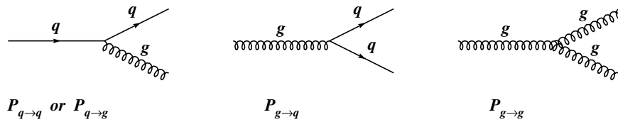
Figure 1.2: Parton splitting diagrams. The corresponding probability functions represented by each diagram is also given beneath each process.
