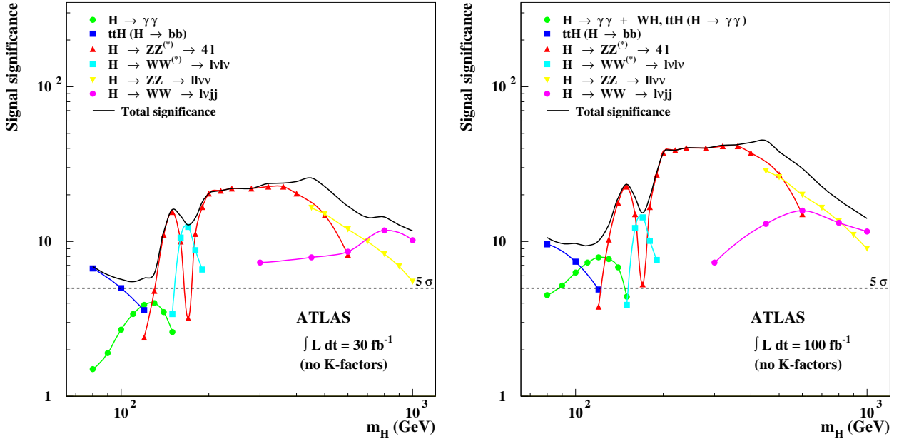
Figure 2.14: Expected observability of the Standard Model Higgs boson in ATLAS, in terms of the statistical significances for various decay channels, as a function of the Higgs mass and for an integrated luminosity of 30 fb^{-1} (left) and of 100 fb^{-1} (right). The statistical significance for the combination of all the decay channels are also superimposed on both plots. Taken from [46].
