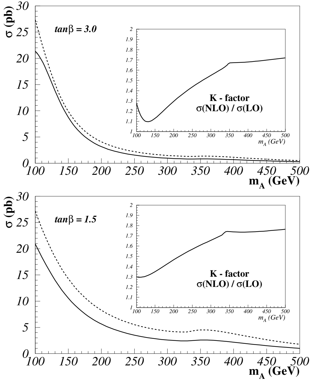
Figure 7.9: The gg \rightarrow H production cross-sections of the neutral CP-even heavy Higgs, H , at one- (full curve) and two-loop (dashed curve) for \tan\beta values discussed in the text. The corresponding K-factor, defined as the ratio of the two- to one-loop cross-section, is also superimposed in each case. The Monte-Carlo program HIGLU [59, 60] have been used to obtain these plots.
