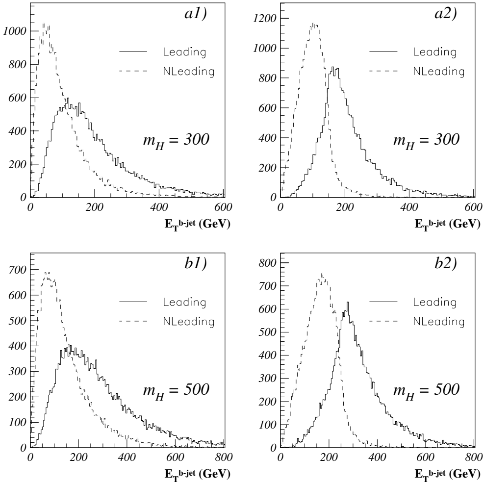
Figure 7.20: The E_T distribution of the partonic b -jets produced in the bbH \rightarrow bbbb process. The a plots are for the m_H = 300 GeV and the b plots for the m_H = 500 GeV case. The E_T distributions of the associated b -jets is suffixed with the digit 1 and that of the H decay product b -jets is suffixed with the digit 2. In each case the leading (full-line) and the next-to-leading (dashed-line) jet distributions are shown.
