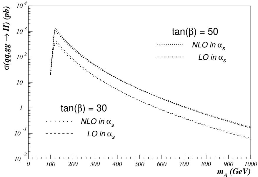
Figure 7.18: MSSM neutral CP-even heavy Higgs associated production cross-section, \sigma(gg, q\bar{q} \rightarrow b\bar{b} H) for \tan\beta = 30, 50 as obtained from HQQ program [60].
