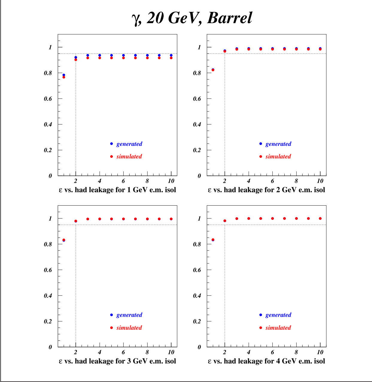
Figure 5.27: Efficiency plots for a 20 GeV photon in the barrel for the full (●) and the fast (●) simulations. The 95% efficiency points are shown with dotted lines.
