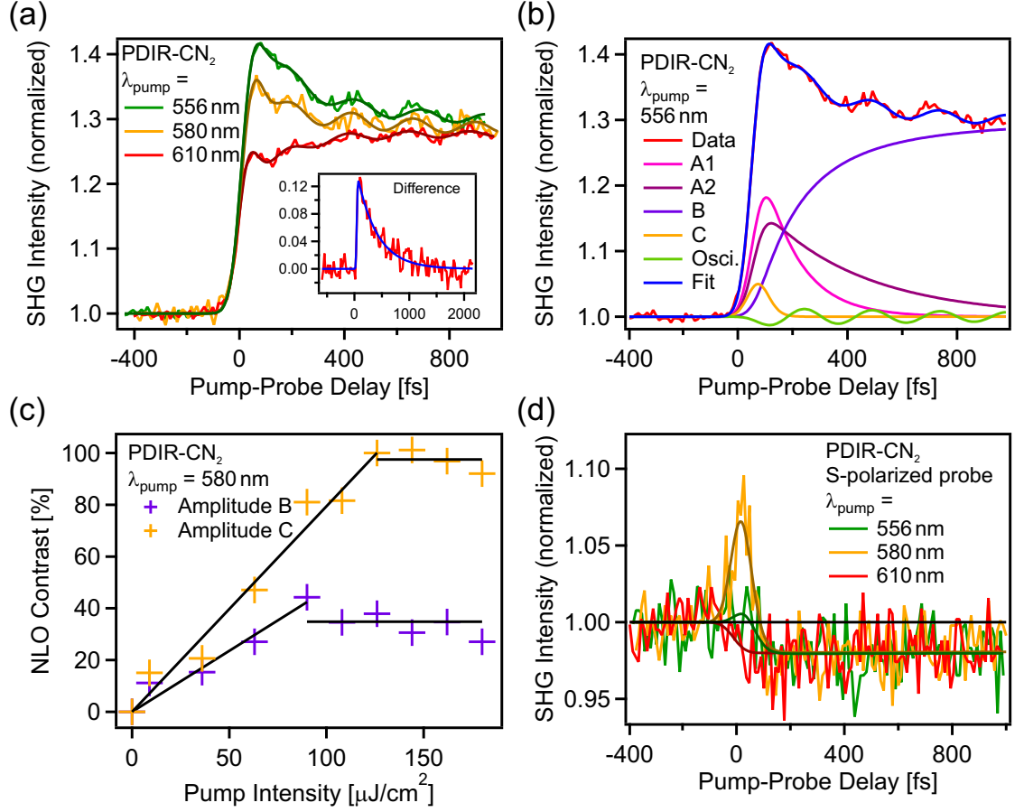
Figure 4.13: (a) Dependence of the TR-SHG trace on the pump wavelength. Insert: Difference between the TR-SHG response for a pump wavelength of 556 nm and 610 nm. (b) TR-SHG trace for 556 nm overlaid with an expanded fit model (see text). (c) Pump intensity dependence of the amplitudes of feature B and C. (d) Dependence of the TR-SHG trace on the pump wavelength for s-polarized probe light.
