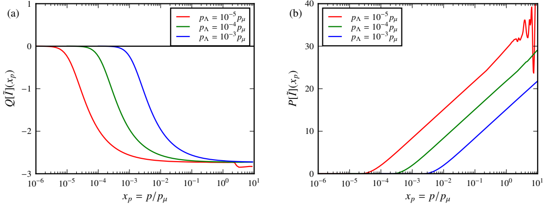
Figure 5.3: The particle flux Q[\tilde{I}](x_p) and the energy flux P[\tilde{I}](x_p) calculated from the rescaled scattering integral \tilde{I}(x_p) are shown as functions of the rescaled momentum x_p in panel (a) and (b) respectively. The evaluation has been done at the analytically predicted scaling exponents, i.e. at \kappa = 7/3 for Q[\tilde{I}](x_p) and \kappa = 3 for P[\tilde{I}](x_p) .
