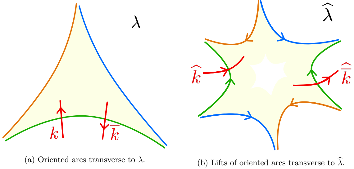
Figure 3.7.: For an oriented arc k transverse to the lamination \lambda that intersects a leaf, drawn in green here, there exists a unique lift \widehat{k} transverse to \widehat{\lambda} such that the intersection \widehat{k} \cap \widehat{\lambda} is positive. If \overline{k} is the same arc with opposite orientation, then its lift \widehat{\overline{k}} intersects the other lift of the leaf.
