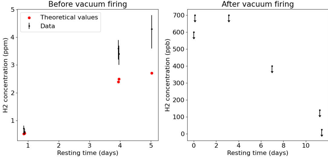
Figure 5.2.: Comparison of hydrogen outgassing of a pipette before (left) and after (right) vacuum firing. The theoretical outgassing values for a pipette without vacuum firing are plotted with red dots. After vacuum firing, no hydrogen is detected in outgassing after more than 10 days. The lower detection threshold of the last point is due to a smaller sample dilution.
