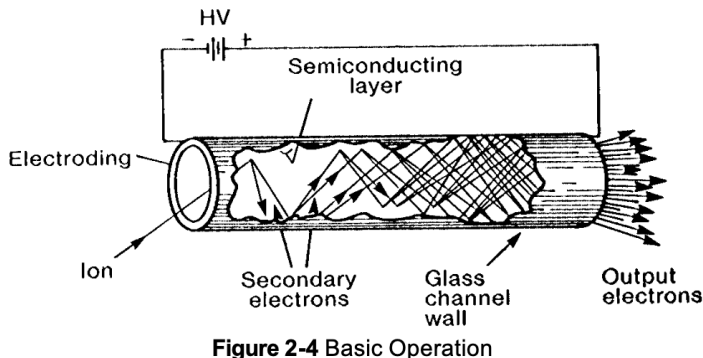
Figure 2-4 Basic Operation
