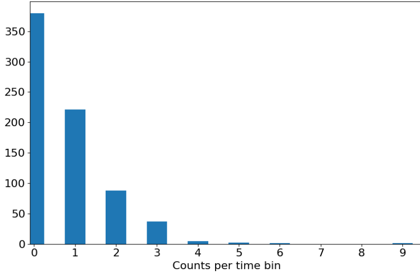
Figure 3.22.: Example of the distribution of counts per time bin for the krypton trace.
