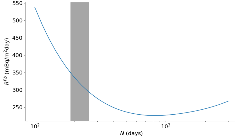
Figure 6.21.: Evolution of R^{\text{Pb}} as a function of N . The best possible constrain comes for measuring a sample after 880 days and it is 225 mBq/M m day. The grey shaded area shows the time span of when the samples were measured for this work.
