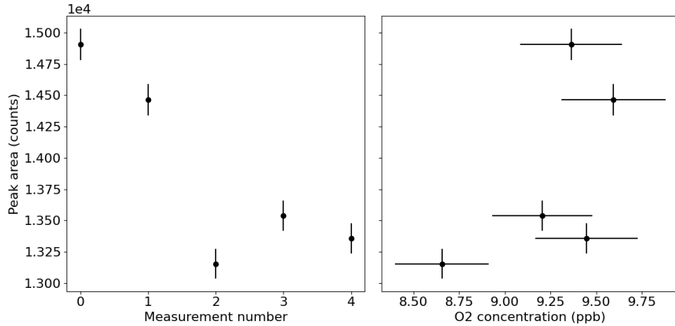
Figure 4.7.: Left: oxygen response during measurements performed in one day after spiking the column with \sim 1\text{ppm} of oxygen. The response does not correlate with the measurement number. Right: same data respect to oxygen amount in the sample volume, where now a trend can be seen.
