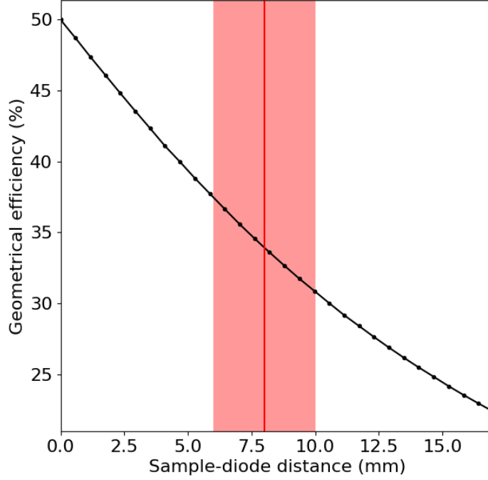
Figure 6.8.: Geometrical efficiency as a function of the distance between the sample and the PIN diode ( d ). The distance used distance in this work and its uncertainty is marked in red ( d = 8 \pm 2 mm).
