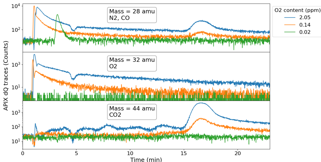
Figure 4.5.: Chromatography spectrum with Shincarbon. The green trace is taken at different flow conditions, which changes the elution time for nitrogen.
