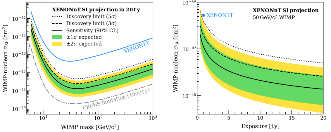
Figure 2.8.: Left: Projection of XENONnT sensitivity for spin-independent WIMP-SM nucleus cross section. Right: Sensitivity vs exposure for a WIMP with mass 50 \text{GeV}/c^2 . Figure taken from [48].
