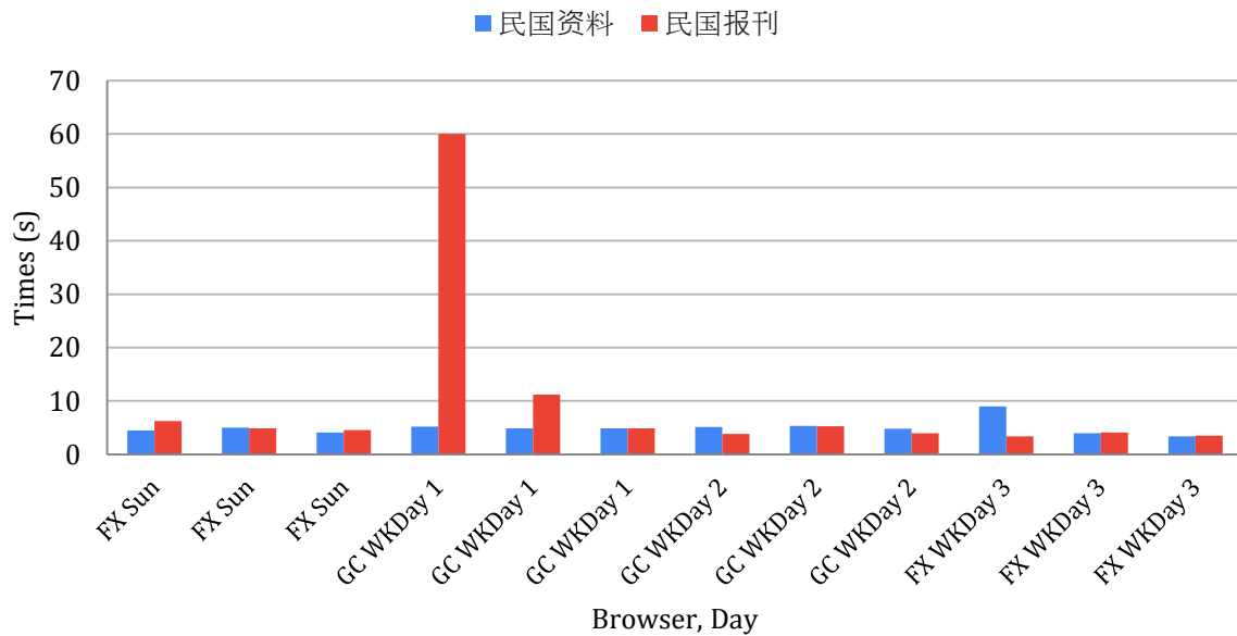
Fig. 10 Time for re-triggered searches
