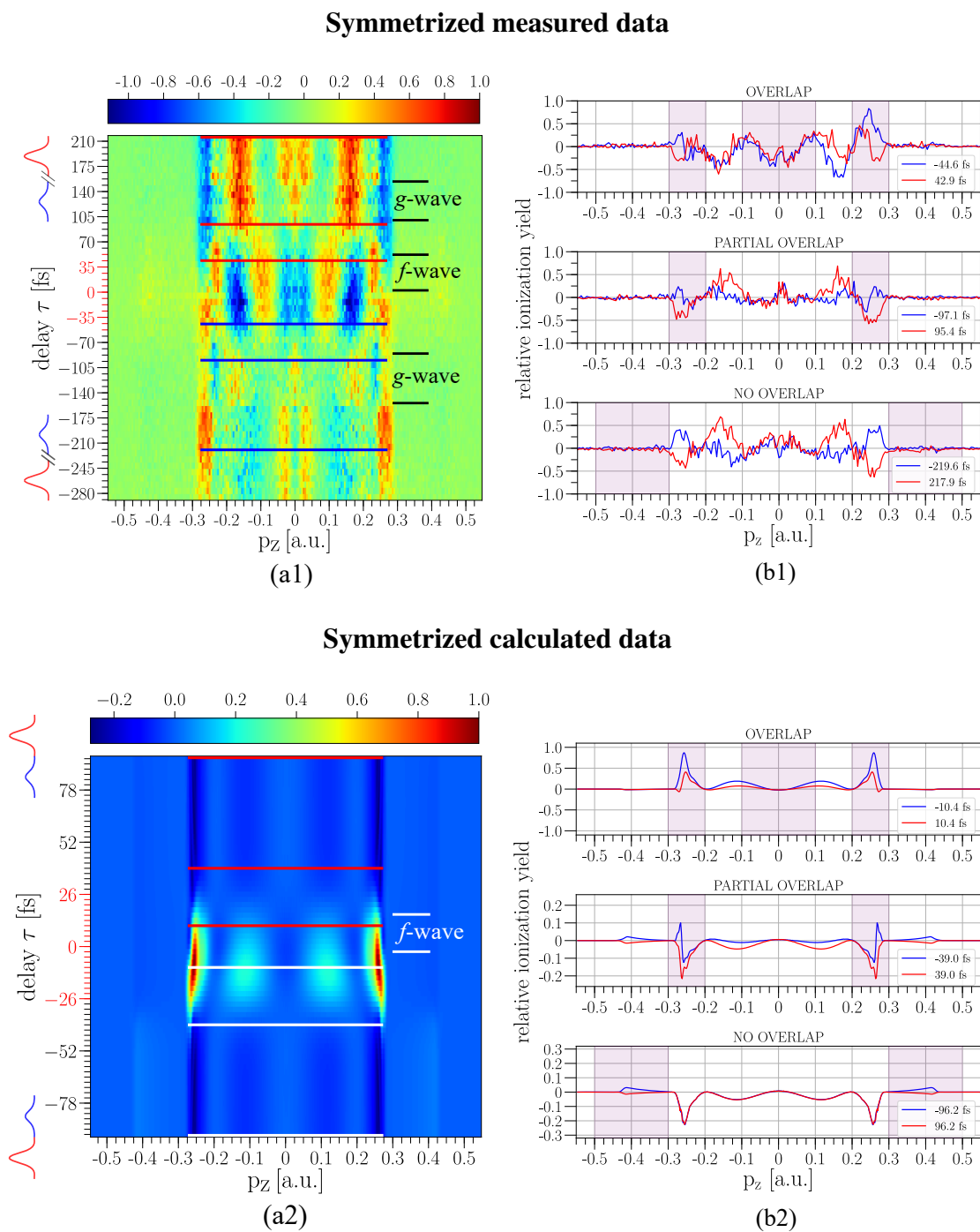
Figure 4.5.: (a1, a2) Symmetrized delay traces of longitudinal momentum spectra. Red ticks mark the span of the FWHM of the pulse overlap delay range. (b1, b2) Comparison between processed longitudinal momentum spectra at positive and negative delays within the overlap, partial overlap, and no overlap delay ranges between the two-color pulses. Purple-shaded areas mark features that appear both in experiment and theory. Red and white horizontal lines in (a1) and (a2) mark the delays of (b1) and (b2), respectively.
