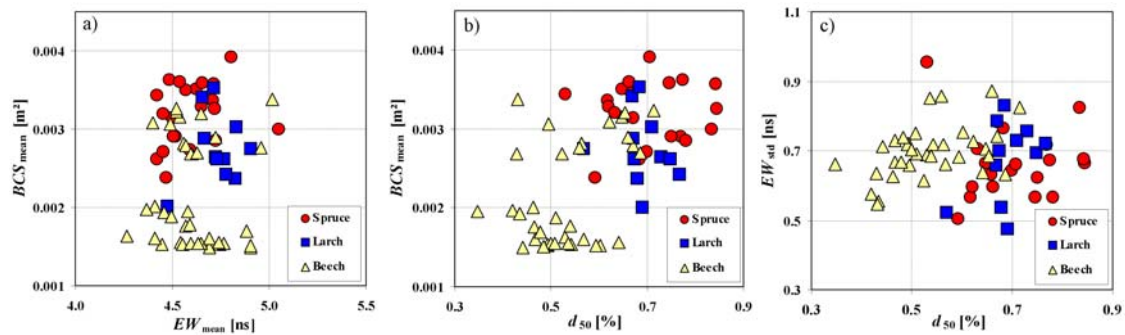
Figure 2: Mean values of point cloud attributes per field measured crown areas for different tree species. a) backscatter cross section ( BCS_{\text{mean}} ) vs. echo width ( EW_{\text{mean}} ), b) ( BCS_{\text{mean}} ) vs. canopy density ( d_{50} ) and c) standard deviation of echo widths ( EW_{\text{std}} ) vs. d_{50} .
