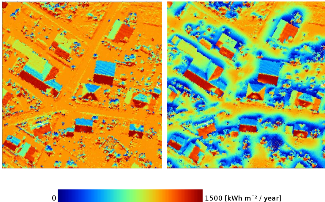
Fig. 4: Results of point cloud based solar radiation modeling. Left: incoming solar radiation without considering shadows of nearby objects. Right: consideration of shadows caused by objects by calculating the horizon of each point within the original 3D point cloud.
