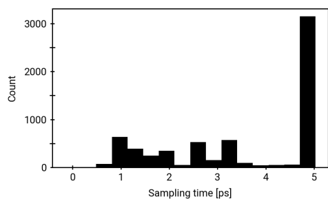
(c) Histogram of the achieved simulation lengths of the umbrella window simulations.
