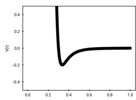
Figure 2.7: A Lennard-Jones potential.
