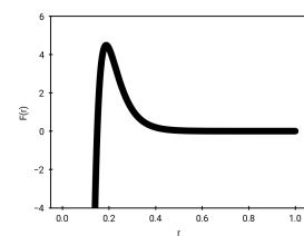
Figure 4.12: The derivative of the Morse potential, i.e., the force as a function of the bond distance r .
