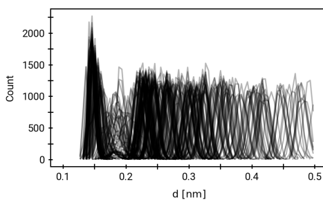
(d) Histograms of the coverage of the umbrella windows over the reaction coordinate of TS1.
