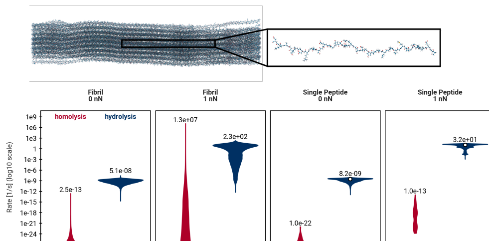
Figure 4.23: Reaction rates (log 10 -scale) for homolysis and hydrolysis in the collagen fibril system (left) and the single chain (right), with the systems visualized above the plot. The 1 nN case for the fibril system represents the shear pulling setup. The value of the highest rate for each setup is shown above the respective distribution. The white points in the hydrolysis rate distributions of the single peptide denote the experimental reference value from AFM experiments [20] for the respective force. Rates lower than 10^{-25} 1/s are not shown.
