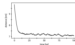
Figure 3.4: The distance between the pull groups for the external force as a function of time for the equilibration of the triple helix under 1 nN.
