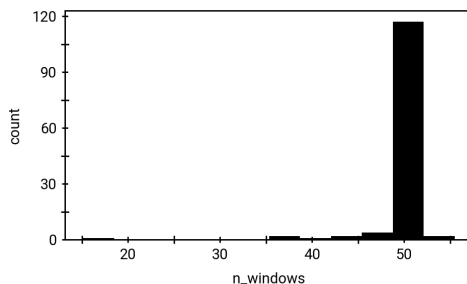
(b) Histogram of the number of umbrella sampling windows per hydroxide attack trajectory.
