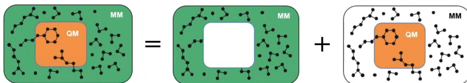
Figure 2.11: Electrostatic embedding scheme for QM/MM. Figure by Dmitry Morozov [80].
