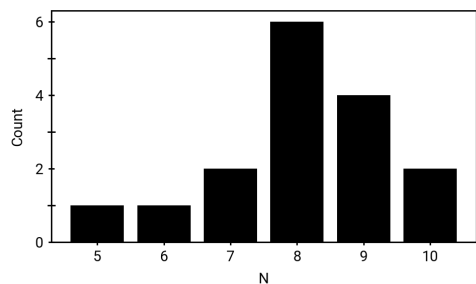
(a) Histogram of the number of successful simulations of the hydroxide attacks on the peptide bond out of 10 starting frames.
