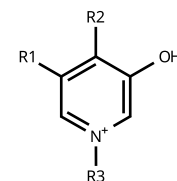
Figure 4.27: Center of a pyridinoline crosslink.
