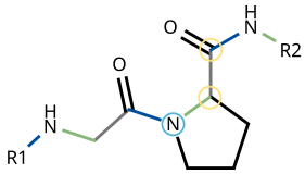
Figure 4.20: A Glycine-Proline peptide highlighting the three bond types of the protein backbone. Blue: amide C – N (the peptide bond with atom types C-N); Green: N – C (with atom types N-CT); Gray: C – C (with atom types CT-C).
