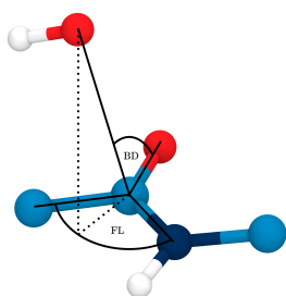
Figure 3.7: Schema of the Bürgi-Dunitz and Flippin-Lodge angles.
