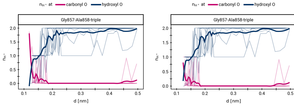
(a) Protonation states before filtering. (b) Protonation states after filtering.
