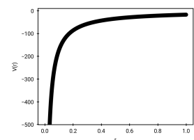
Figure 2.8: A Coulomb potential.
