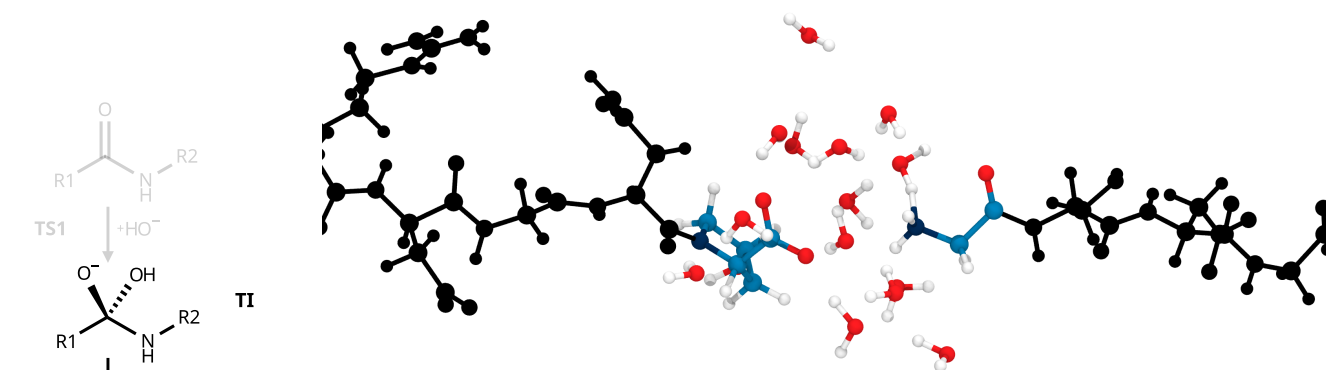
Figure 3.19: The QM subsystem (in color) and the MM subsystem (in black) of a single chain system during the rupture of the peptide bond (C–N).
