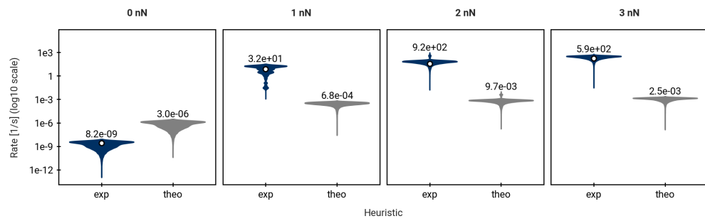
Figure 5.5: Hydrolysis reaction rates (log 10 -scale) for a single chain under force increasing from 0 to 3 nN using the experimental (exp) model compared to the physical model based on single-point energies. Rates lower than 10^{-13} 1/s are not shown.
