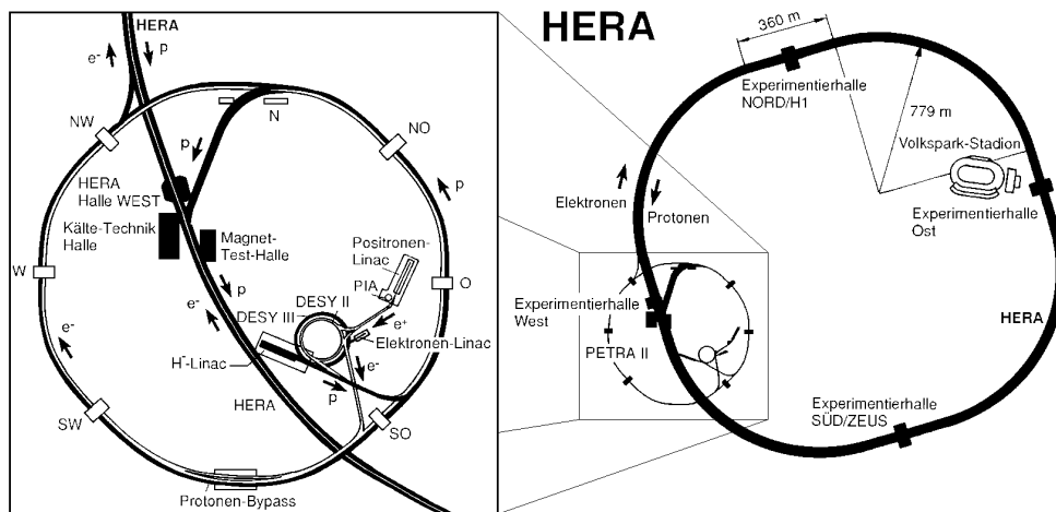
Figure 2.1: Schematic overview of the HERA accelerator complex
