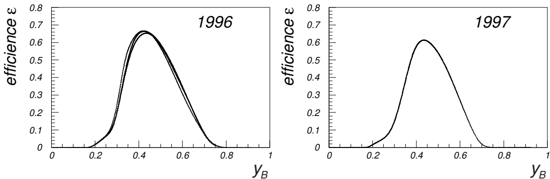
Figure 4.1: Run dependent efficiencies of the electron tagger as a function of y_B for the years 1996 and for the minimum bias data taking period of 1997.
