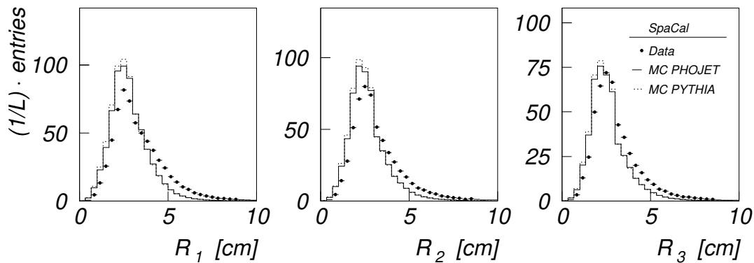
Figure 5.8: SpaCal : Comparison of the radii of the three most energetic clusters in data (points) and the MC models PHOJET (full line) and PYTHIA (dotted line).
