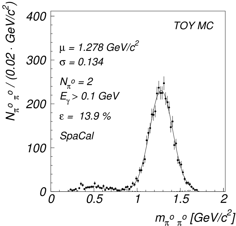
Figure 8.10: TOY MC : Two- \pi^0 spectrum as seen in the SpaCal. Only the tensor meson f_2(1270) was generated by the TOY MC with the p_\perp distribution presented in [BER00].
