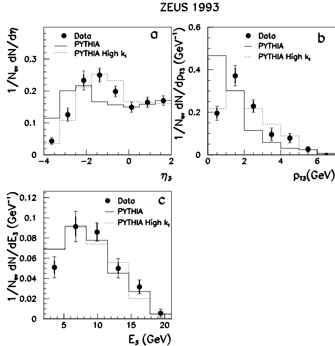
Figure 1.10: (a) Pseudo-rapidity of the third jet corrected back to hadron level. (b) Corrected p_{\perp} distribution (c) Corrected energy distribution. In (b) and (c) the cut \eta < -1 is applied. The solid line represents the prediction of PYTHIA assuming a Gaussian distribution of the initial k_{\perp} while the dotted line shows the prediction of PYTHIA according to a power like initial k_{\perp} distribution with k_0 = 0.66 GeV/c.
