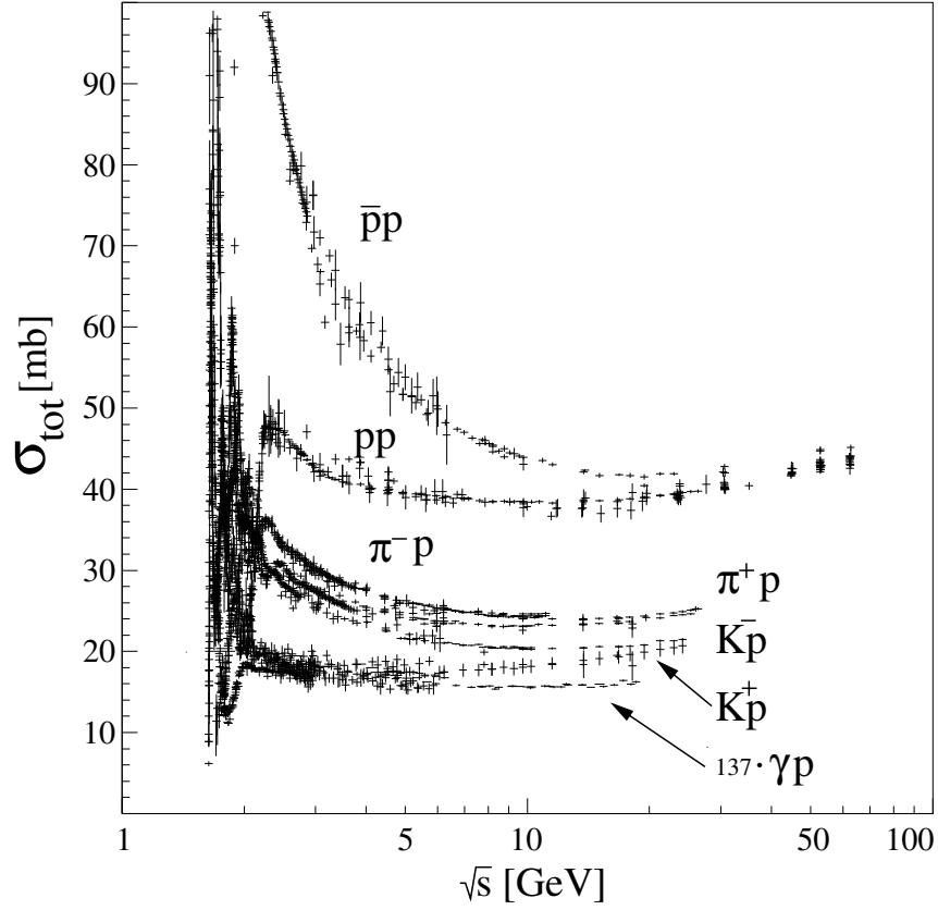
Figure 1.3: Total cross section for various particle reactions as a function of the CM energy. The photon-proton cross sections have been multiplied by a factor of \frac{1}{\alpha_{em}} .
