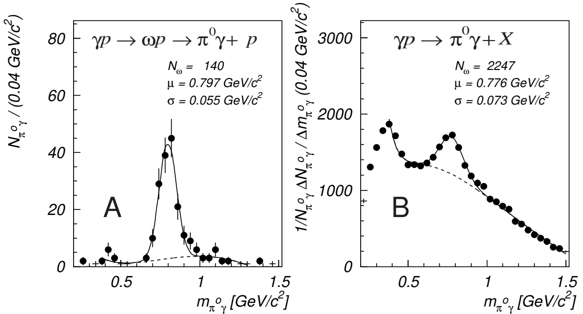
Figure 8.1: SpaCal : A. \pi^0\gamma mass spectrum which comes from elastic events, B. inclusive \pi^0\gamma mass spectrum.
