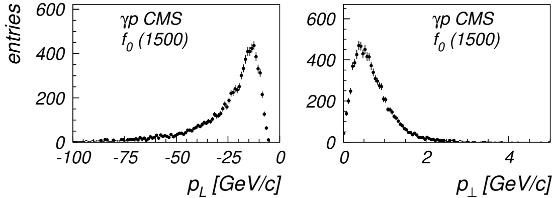
Figure 8.2: Longitudinal (left side) and transverse (right side) momenta of the f_0(1500) meson in \gamma p CMS, used in the TOY MC.
