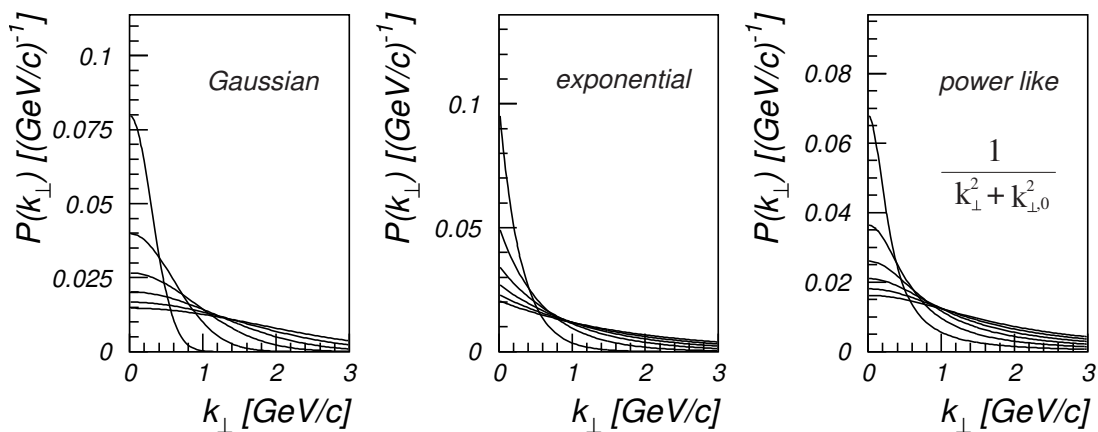
Figure 1.8: Three assumptions on the primordial k_{\perp} distributions of the photon remnant: a Gaussian, an exponential and a power law distribution. The width of the distributions increases from 0.3 GeV/c to 1.8 GeV/c in steps of 0.3 GeV/c.
