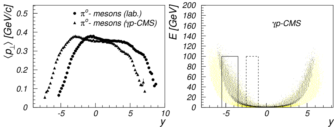
Figure 1.12: Kinematical range accessible for \pi^0 and \eta mesons at HERA in the \gamma p CMS. The gray points refer to the \pi^0 s and the black points to the \eta s. The kinematical range within the boxes is studied by this analysis.
