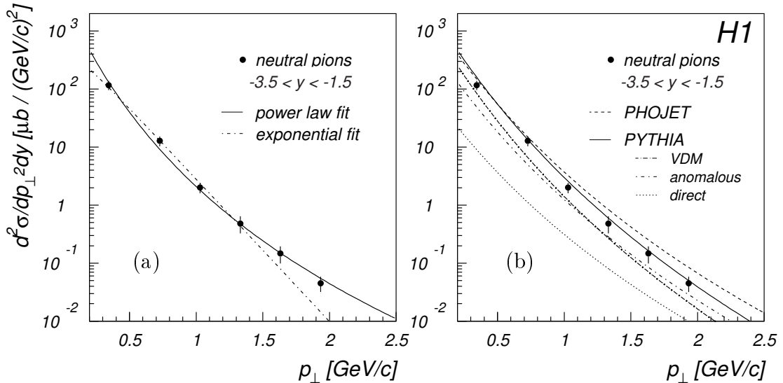
Figure 6.13: (a) Inclusive \pi^0 photoproduction cross section as a function of p_\perp (circles), for the rapidity region -3.5 < y < -1.5 . The dash-dotted curve is a fit of an exponential to the data in the range 0.3 < p_\perp < 1.6 GeV/c; the full curve is the result of a power law fit (see text). (b) Same cross section as in (a) but this time compared to predictions of PHOJET and PYTHIA. In addition, the decomposition (PYTHIA) into VDM, anomalous, and direct contributions is shown.
