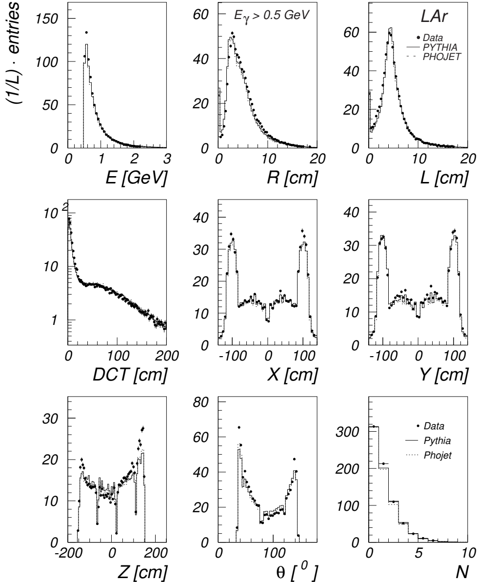
Figure 5.17: LAr: Comparison of data (points) with reweighted MC PYTHIA 5.722 (full line) and reweighted MC Phojet 1.04 (dotted line). E = Cluster energies, R = Radial cluster extension, L = Longitudinal cluster extension, DCT = Distance of Cluster center of gravity from next Track (DTNV bank), X, Y, Z = Cluster coordinates, \theta = Polar-angle, N = Number of cluster cells. Used bank: AE0R.
