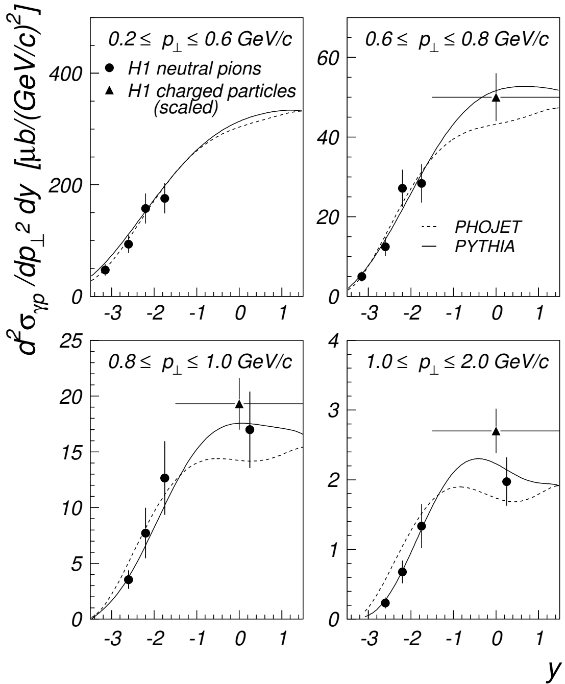
Figure 6.11: Inclusive \pi^0 photoproduction cross section as a function of laboratory rapidity y in intervals of transverse momentum p_{\perp} (full circles), for Q^2 \leq 0.01 \text{ GeV}^2 and 0.35 < y_B < 0.65 . The triangles are the corresponding cross section values for charged pions, derived from [ABT94] by subtracting a fraction of 17.5% to account for the “non-pion” contribution, and then dividing by the isospin factor 2 (see text). The curves are the predictions of the PHOJET (dashed) and PYTHIA (full) event generators for neutral pions.
