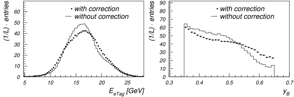
Figure 5.4: Left side: Energy of the electron tagger for the minimum bias run 1997 before and after the energy correction. Right side: reweighted y_B distribution (see section 4.3) before and after the energy correction. y_B = 1 - E'_e/E_e with E_e = electron beam energy, E'_e = energy of scattered electron.
