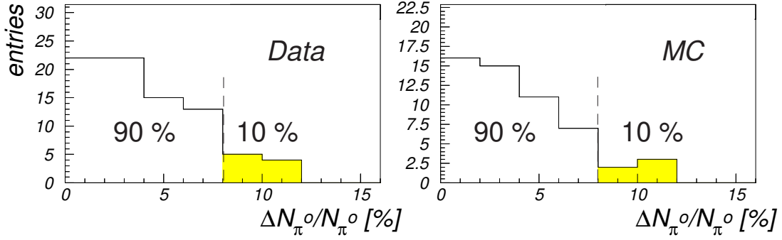
Figure 6.2: The distribution of \Delta N_{\pi^0, \text{fit}}/N_{\pi^0} for all bins in which the \pi^0 cross section is measured. The dashed line marks the final error on N_{\pi^0} .
