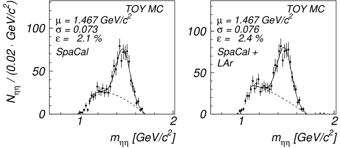
Figure 8.5: TOY MC : Two- \eta spectra as seen in the SpaCal (left side) and as seen in the SpaCal and LAr calorimeters together (right side). Only the f_0(1500) meson, scattered into the backward region of the H1 calorimeter, was generated by the TOY MC . The reconstruction efficiencies \epsilon for the f_0(1500) reconstruction are shown in the plots.
