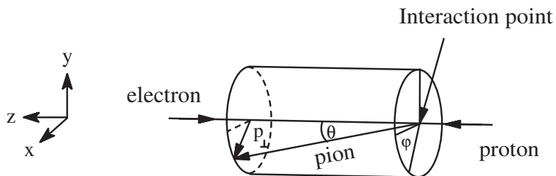
Figure 1.2: Variables of the hadronic final state.
