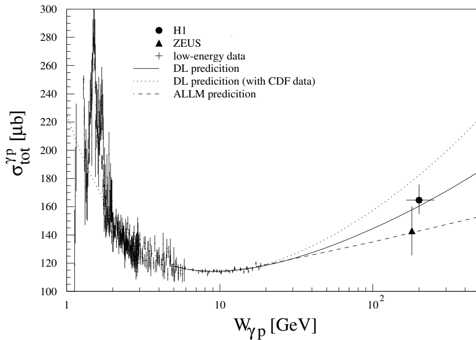
Figure 1.4: Total \gamma p cross section as measured at HERA.
