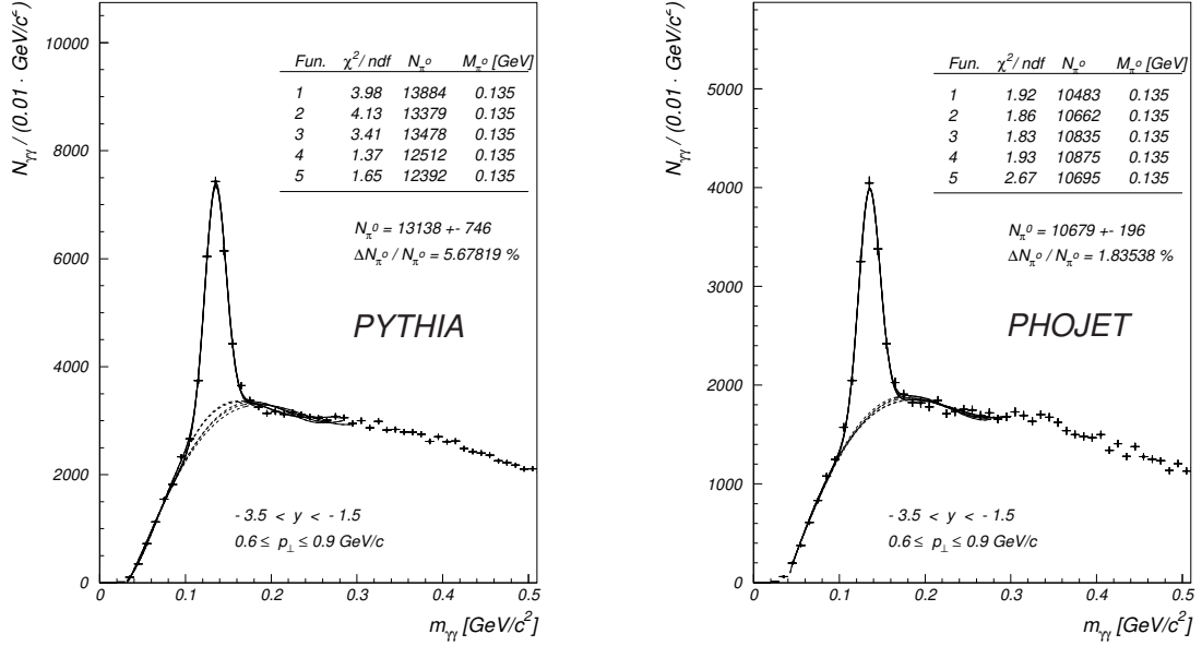
Figure 6.1: MC PYTHIA: m_{\gamma\gamma} spectra (SpaCal) in intervals of the \pi^0 transverse momentum fitted by different functions ( -3.5 < y < -1.5 ). Table 6.1 gives the fit function referring to the number given in the plots above.
