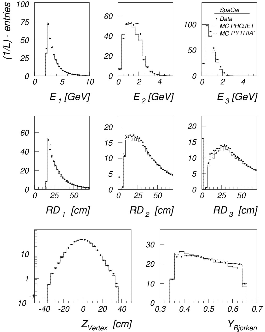
Figure 5.9: Spacal: Comparison of data selected by subtrigger 50 and the reweighted MC models PHOJET (full line) and PYTHIA (dotted line). E_1 - E_3 = Energy of the first three most energetic clusters, RD_1 - RD_3 the corresponding radial distance of the cluster center from the beam line. The z -vertex and the y_B distribution.
