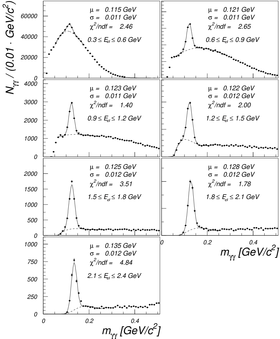
Figure 5.1: SpaCal : m_{\gamma\gamma} distributions in intervals of the cluster energy (data). The mass peak is fitted with a Gaussian, the background with a polynomial of fourth order.
