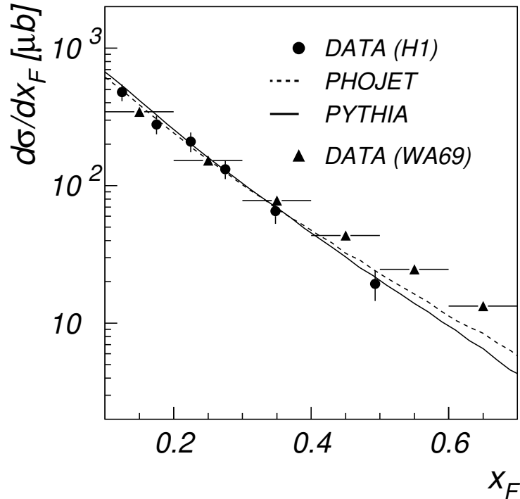
Figure 6.16: Inclusive \pi^0 photoproduction cross section as a function of Feynman x . The curves are the predictions of the PHOJET (dashed) and PYTHIA (full) models. The H1 data, at \sqrt{s_{\gamma p}} \approx 208 GeV, as well as the MC model predictions, are obtained in the rapidity range -3.5 < y < -1.5 . The data of the Omega Photon Collaboration (WA69), at \sqrt{s_{\gamma p}} \approx 12.3 GeV, were derived as described in appendix C.
