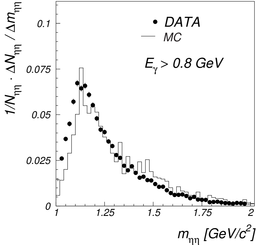
Figure 8.7: Comparison of the \eta\eta spectrum based on the data selected with subtrigger 50 with the spectrum predicted by PYTHIA with enhanced f_0(1500) (TOY MC) production.
