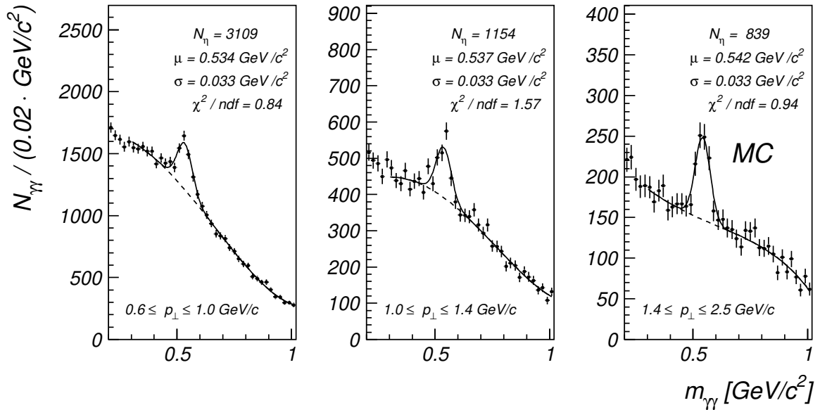
Figure 7.3: The same distributions as shown in figure 7.2 for the simulated events generated by the MC models PYTHIA and PHOJET (see text).
