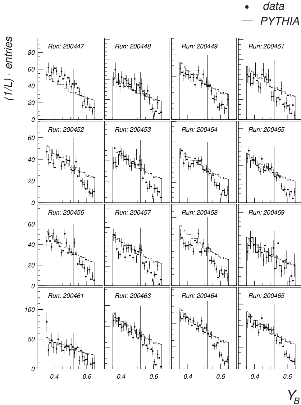
Figure 5.3: Comparison of the y_B distribution in data and the MC PYTHIA. For y_B > 0.52 the electron tagger did not reach its full acceptance.
