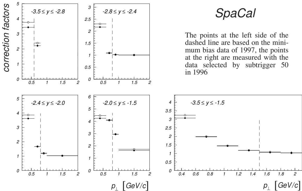
Figure 6.8: Correction factors for the number of events lost due to the cut on the most energetic cluster in the SpaCal and on the radial distance of its center of gravity from the beam line.
