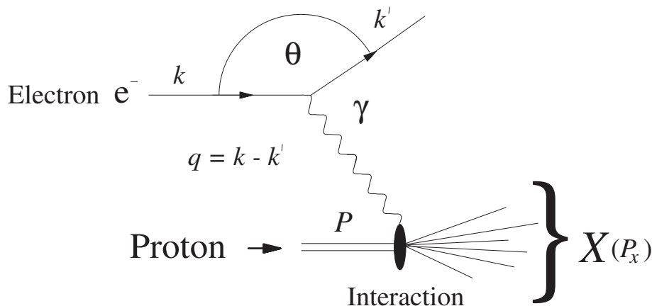
Figure 1.1: Electron-Proton scattering via photon exchange. k , k' , P and P_x denote the four-momenta used to construct Lorentz-invariant quantities.
