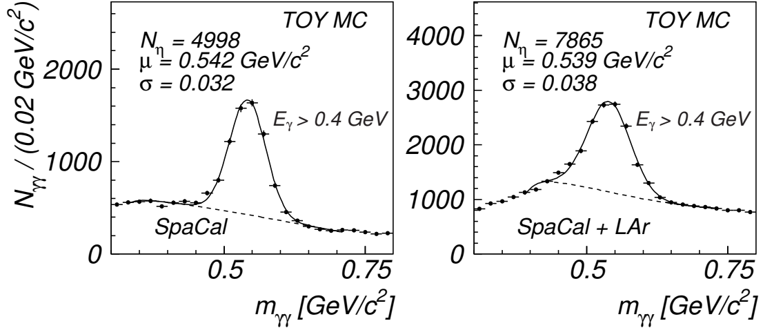
Figure 8.4: TOY MC: The two-photon distribution of the decay f_0(1500) \rightarrow \eta\eta \rightarrow \gamma\gamma\gamma\gamma as reconstructed in the SpaCal (left side) and as reconstructed in both, the SpaCal and LAr calorimeters (right side).
