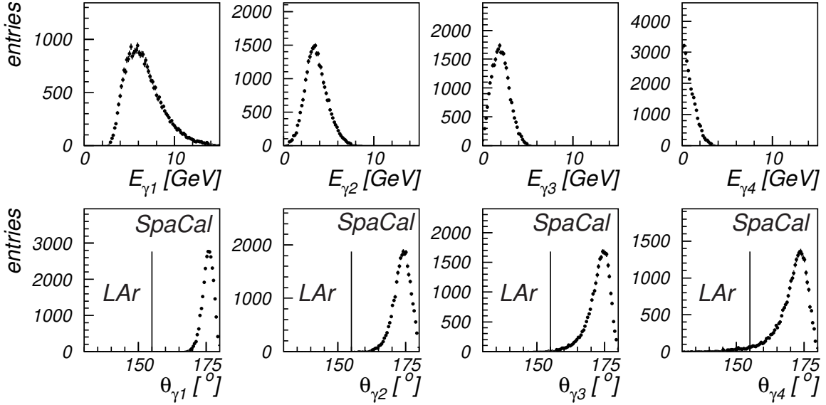
Figure 8.9: TOY MC: Energy and polar angle distributions of the four decay photons of the exclusively produced f_2(1270) as seen in the lab system. The line indicates the polar angular acceptance regions of the SpaCal and LAr calorimeter, respectively.
