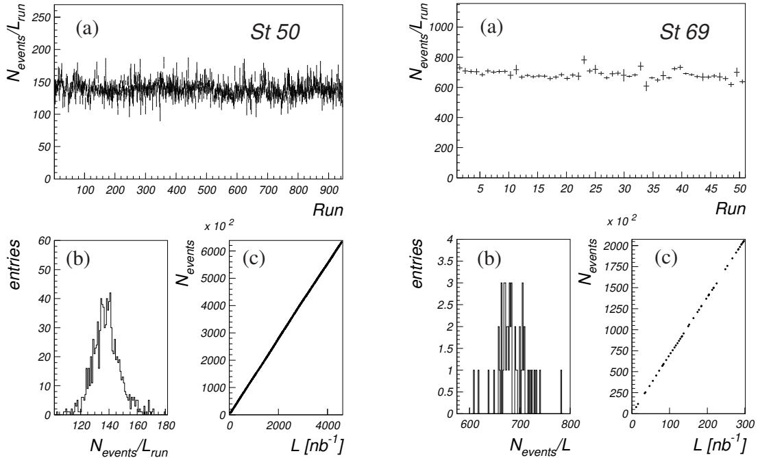
Figure 4.3: The number of events in the plots a,b and c fulfil the selection cuts listed in table 4.1 for subtrigger 50 and 69 respectively. (a) Number of events over the run luminosity as a function of the run number. (b) Number of events per run luminosity. (c) Number of selected events as a function of the integrated luminosity.
