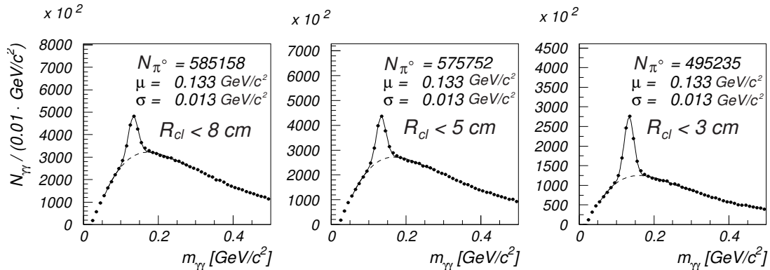
Figure 5.11: SpaCal : m_{\gamma\gamma} distributions for different cuts on the cluster radius ( E_{cl} > 0.3 \text{ GeV} ).
