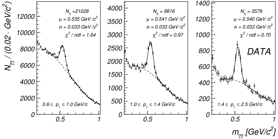
Figure 7.2: Data: m_{\gamma\gamma} spectra of the SpaCal in the mass range of the \eta meson for different intervals of the \eta transverse momentum and for the \eta rapidity range: -3.5 < y < -1.5 .
