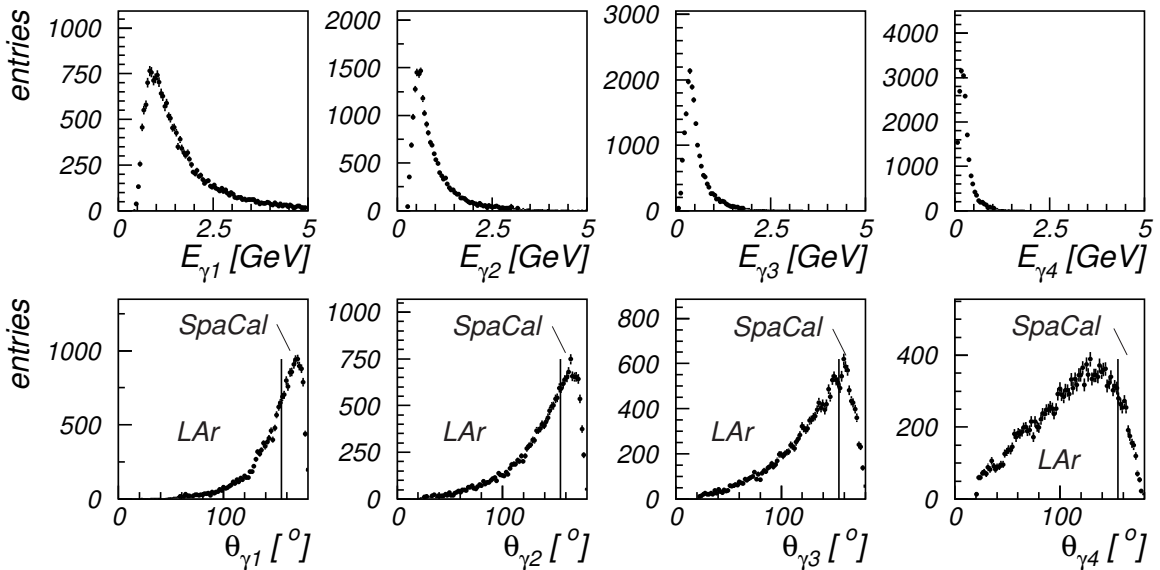
Figure 8.3: TOY MC: Energy and polar angle distributions of the four decay photons of the f_0(1500) as seen in the lab system. The line indicates the polar angular acceptance regions of the SpaCal and LAr calorimeter, respectively.
