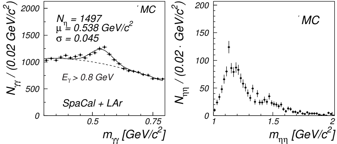
Figure 8.6: TOY MC + PYTHIA : The two-photon distribution of events generated by PYTHIA with one additional f_0(1500) added which was produced by the TOY MC in the backward region of H1. (left side). The \eta spectrum based on the selection of the two-photon combinations in the mass window around the \eta mass (right side).
