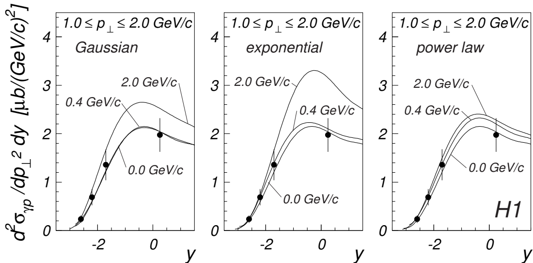
Figure 6.14: The \pi^0 cross section as a function of the \pi^0 rapidity y for the p_\perp range indicated in the figure. The curves are predictions of PYTHIA, labelled with the corresponding k_{\perp,0} values, as described in the text.
