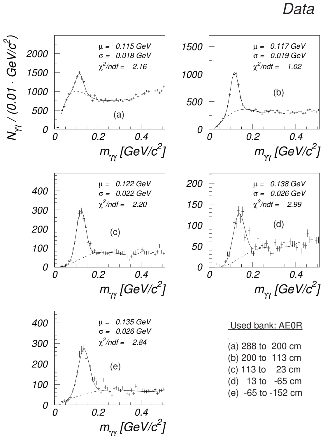
Figure 5.15: m_{\gamma\gamma} distributions reconstructed from photons where both are recorded in the same LAr wheel (Data). The bank AE0R is used.
