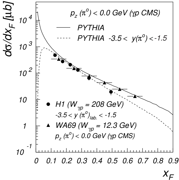
Figure 6.17: The same data points as shown in figure 6.16 but this time also compared to the x_F distribution of PYTHIA for all \pi^0 s scattered into the backward hemisphere in the \gamma p CMS system ( p_{z, CMS} < 0.0 \text{ GeV} ).
