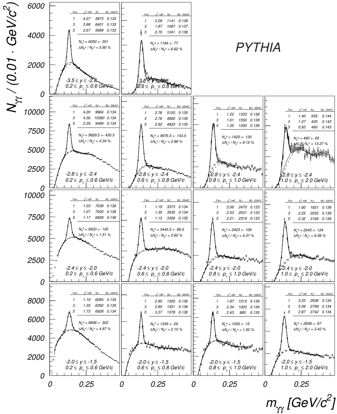
Figure 6.10: MC PYTHIA: m_{\gamma\gamma} spectra (SpaCal) in intervals of the \pi^0 transverse momentum and in intervals of the \pi^0 rapidity fitted by different functions. Table 6.1 gives the fit function referring to the number given in the plots.
