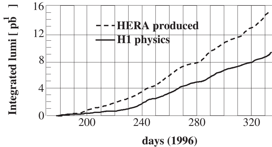
Figure 2.2: Integrated luminosity versus the days of the year 1996. Dashed line: integrated luminosity produced by the HERA machine. Solid line: integrated luminosity collected by the H1 experiment.
