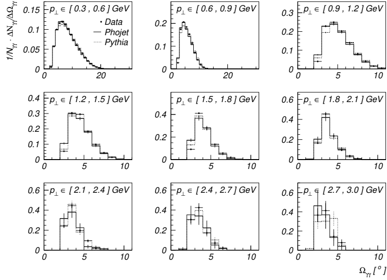
Figure 6.6: Opening angle \Omega_{\gamma\gamma} of all possible two-cluster combinations in the mass band of the \pi^0 ( 0.1 < m_{\gamma\gamma} < 0.17 \text{ GeV}/c^2 ) in intervals of the transverse momentum of the cluster pairs (SpaCal).
