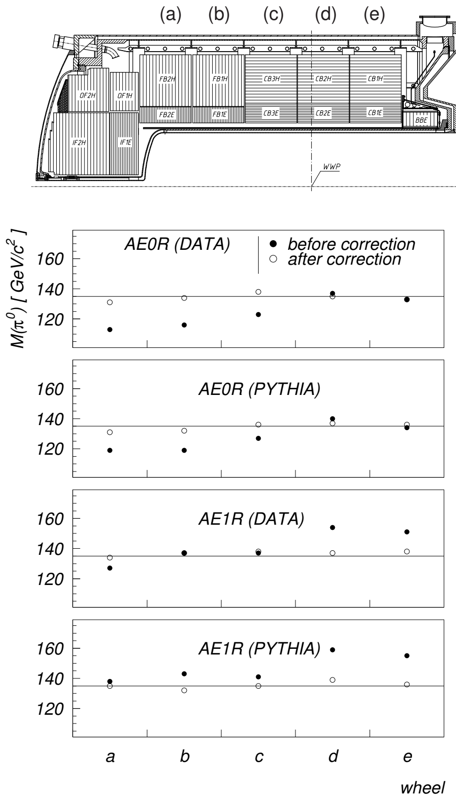
Figure 5.16: Comparison between data and MC model PYTHIA with respect to the \pi^0 mass reconstructed from photons flying into the same LAr wheel. The full points are the values of the \pi^0 mass before the mass correction and the open points are the values of the \pi^0 mass after the mass correction.
