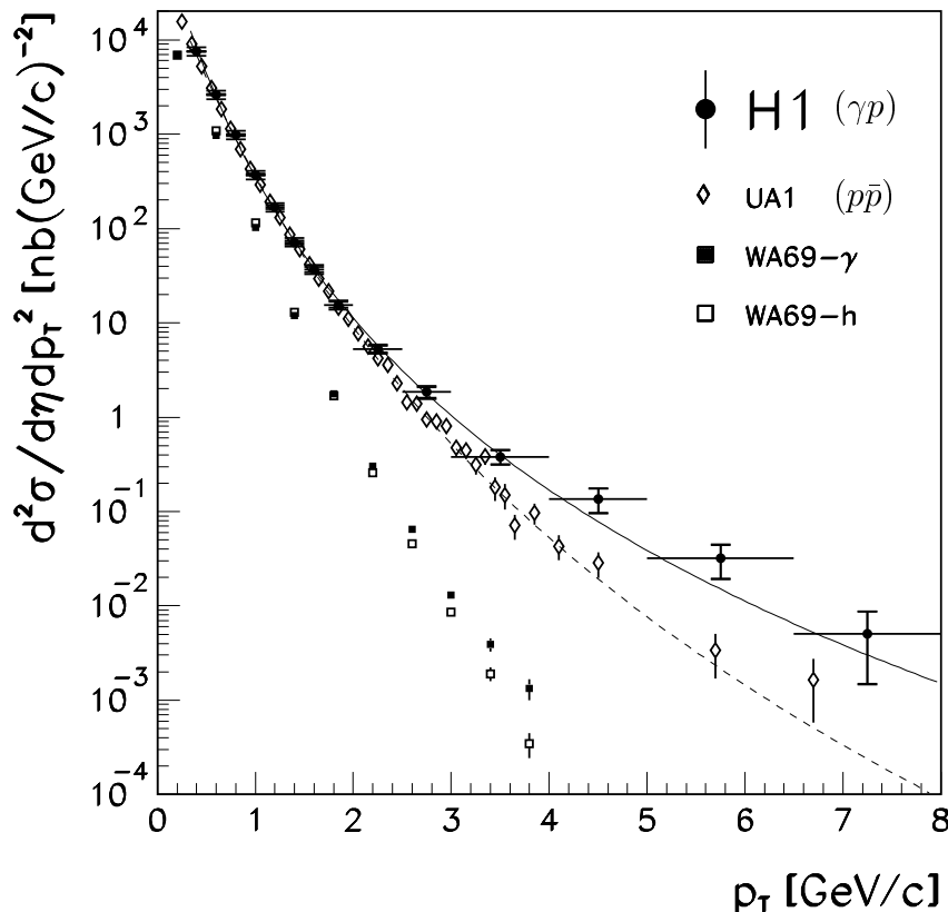
Figure 1.9: The inclusive double differential charged particle cross section d^2\sigma/d\eta dp_{\perp}^2 as a function of the particles transverse momenta p_{\perp} , measured by the H1 Collaboration (full points) in the pseudo-rapidity range |\eta| < 1.5 . The solid (dashed) line is the result of a power law fit (equation 1.29) to the H1 (UA1) data (see text).
