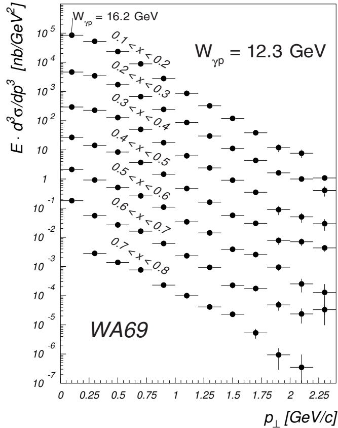
Figure C.1: Invariant neutral pion cross section as measured by the Omega Photon collaboration (see text) at W_{\gamma p} = 12.3 GeV.
