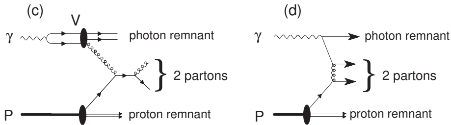
Figure 1.6: Examples for resolved \gamma p processes in leading order QCD. c.) VDM d.) anomalous.
