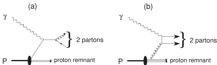
Figure 1.5: Direct \gamma p processes in leading order QCD: a.) QCD-“Compton”-process, b.) photon-gluon fusion.
