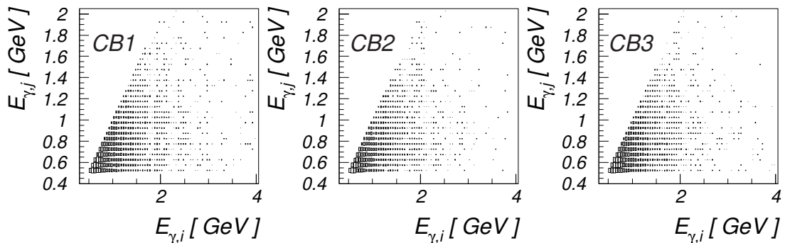
Figure 5.14: Energy of the photons of the LAr calorimeter used for the m_{\gamma\gamma} spectra (data), reconstructed in the central barrels one, two and three, abbreviated with CB1, CB2 and CB3 (compare figure 3.3).
