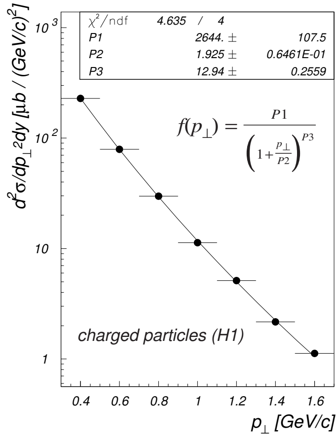
Figure B.1: Charged particle cross section as a function of p_{\perp} for p_{\perp} < 2 \text{ GeV}/c with a smooth interpolation used to account for different momentum ranges in the charged particle and \pi^0 analysis respectively.
