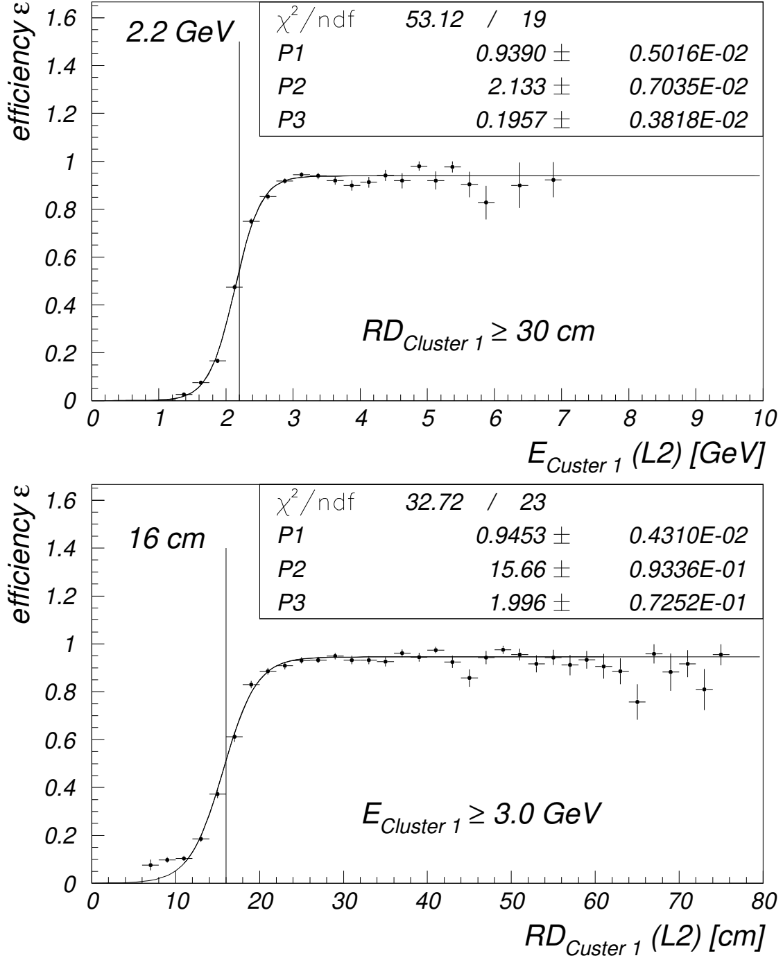
Figure 4.2: Efficiency of subtrigger 50 as a function of the energy of the hottest cluster (upper plot) and as a function of the distance of the hottest cluster from the beam line (lower plot).
