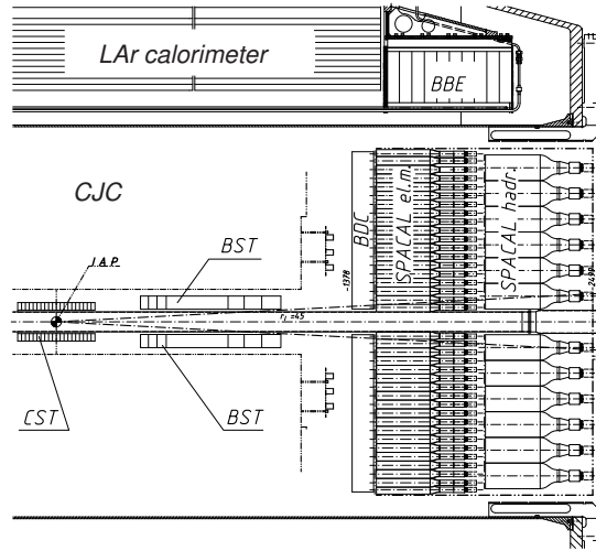
Figure 3.2: A side view of the backward region of the H1 detector.
