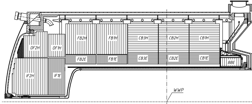
Figure 3.3: A side view of the Liquid Argon calorimeter.
