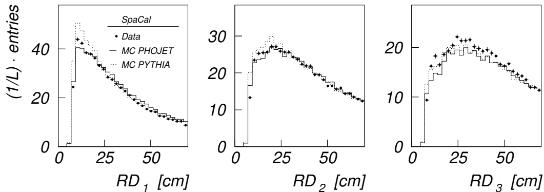
Figure 5.7: SpaCal : Comparison of the radial distribution of the three most energetic clusters in data (points) and the MC models PHOJET (full line) and PYTHIA (dotted line).
