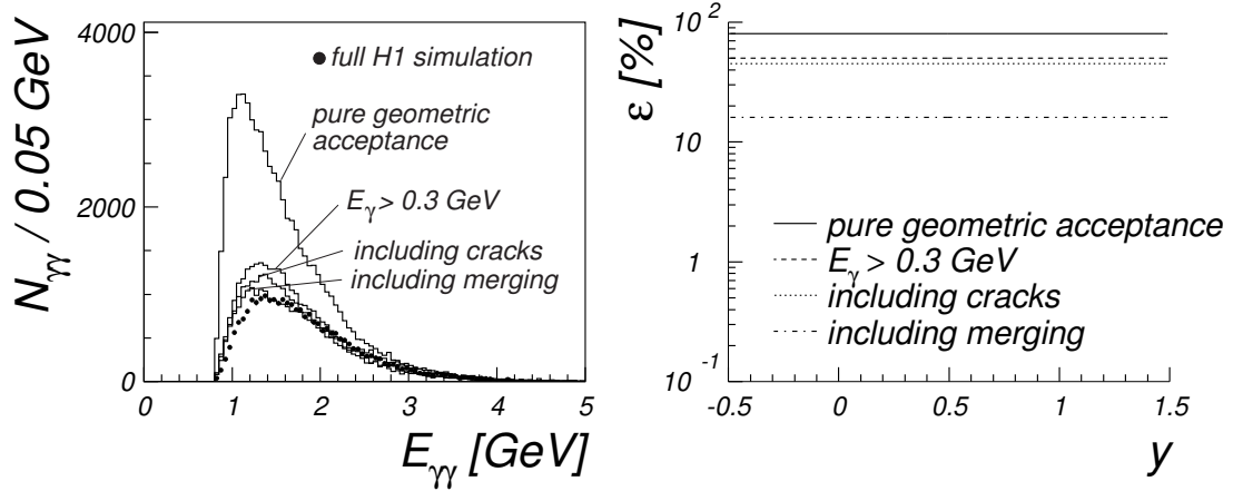
Figure 6.4: Left side: Comparison of the energy of all two-photon combinations between the TOY (see text) and the full detector simulation. The values of the z -coordinate of the LAr calorimeter were restricted to the range -150 < z < 200 \text{ cm} . Right side: The \pi^0 reconstruction efficiency (LAr) for the conditions listed in the legend of the plot.
