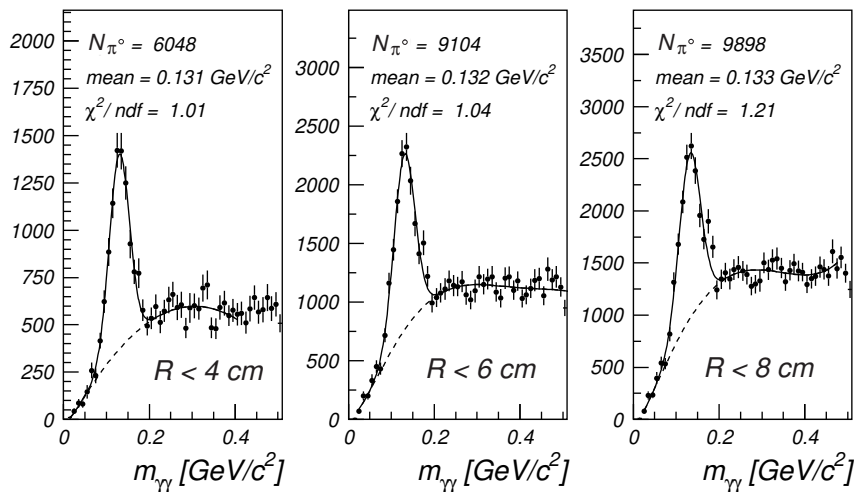
Figure 5.19: LAr: m_{\gamma\gamma} distributions with different cuts on the cluster radius R .
