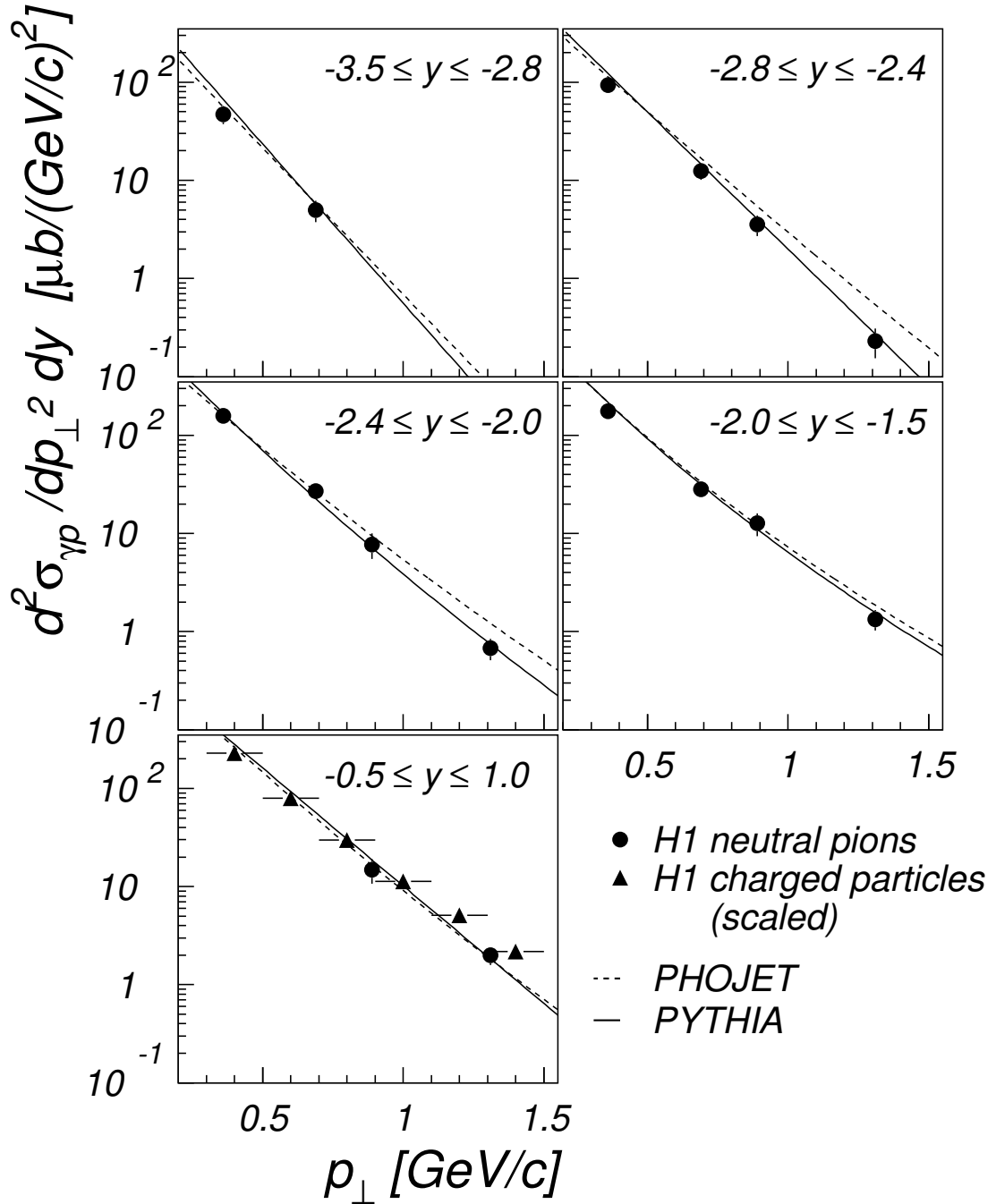
Figure 6.12: Inclusive \pi^0 photoproduction cross section as a function of transverse momentum p_{\perp} in intervals of laboratory rapidity y (full circles). The triangles are the corresponding cross section values for charged pions in the pseudorapidity range |\eta| \leq 1.5 , derived from [ABT94] by subtracting a fraction of 17.5% to account for the “non-pion” contribution, and then dividing by the isospin factor 2 (see text). The curves are the predictions of the PHOJET (dashed) and PYTHIA (full) event generators for neutral pions.
