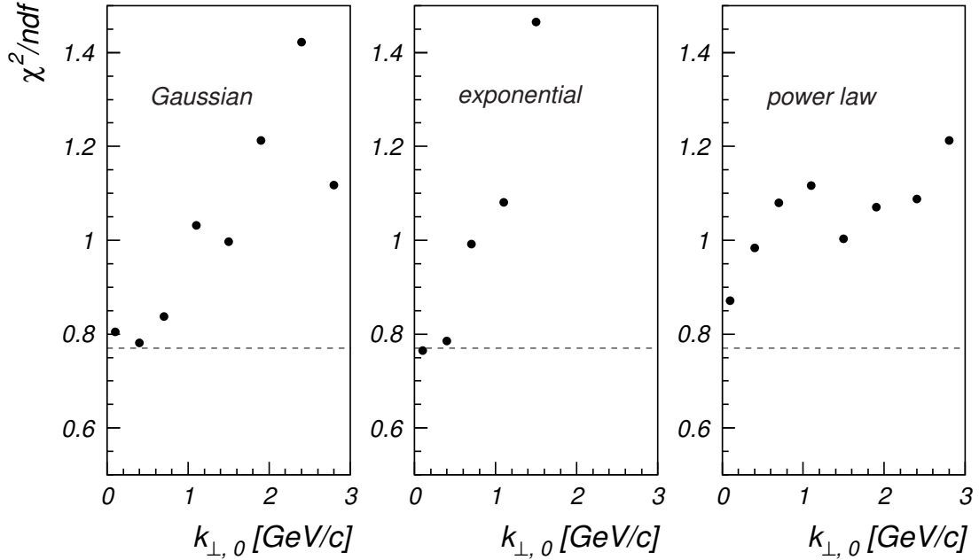
Figure 6.15: \chi^2/ndf as a function of the “primordial” intrinsic k_{\perp} assuming a Gaussian, exponential and power law k_{\perp} distribution. The \chi^2 was obtained taking into account all data points from the double differential cross sections shown in Fig. 6.11 and 6.12 .
