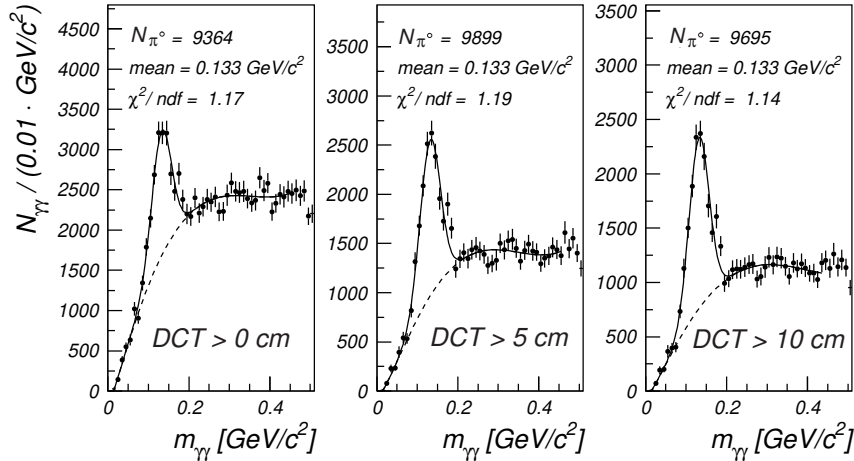
Figure 5.18: LAr: m_{\gamma\gamma} distributions with different cuts on the distance between the cluster center to the closest track.
