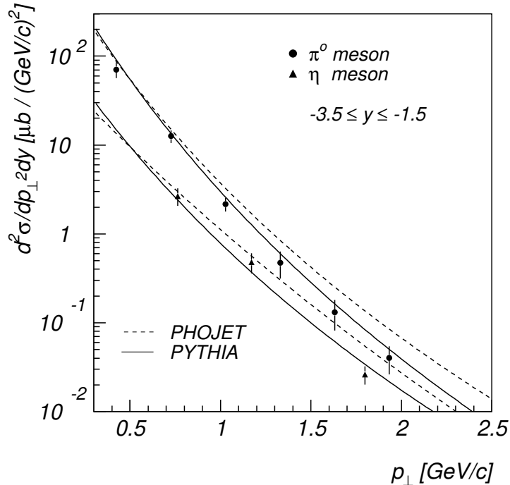
Figure 7.4: Comparison of the inclusive \pi^0 and \eta photoproduction cross sections as a function of p_\perp , for the rapidity region -3.5 < y < -1.5 , for Q^2 \leq 0.01 \text{ GeV}^2 and 0.35 < y_B < 0.65 . The curves are predictions of the PHOJET (dashed) and PYTHIA (full) models.
