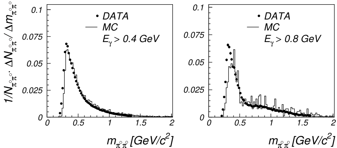
Figure 8.8: Comparison of the \pi^0\pi^0 mass spectrum based on the data selected with sub-trigger 50 with the spectrum predicted by PYTHIA with enhanced f_2(1270) (TOY MC) production for two different cuts on the minimal photon energy.
