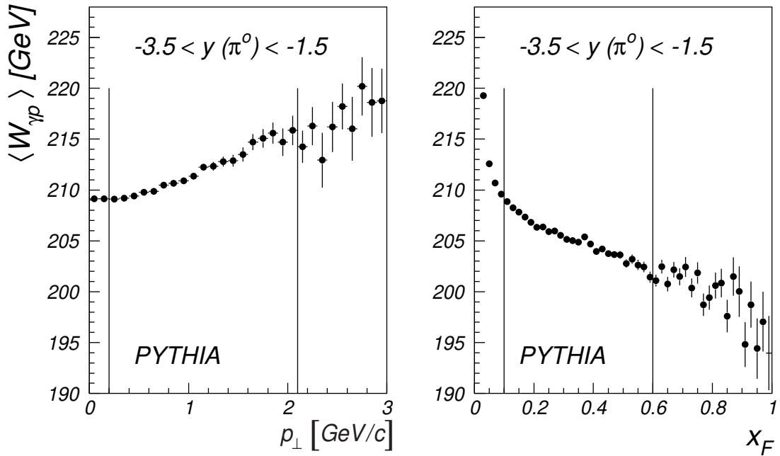
Figure 6.18: PYTHIA : \langle W_{\gamma p} \rangle as a function of the \pi^0 transverse momentum and as a function of x_F . The region within the two vertical lines of each plot mark the range covered by this measurement.
