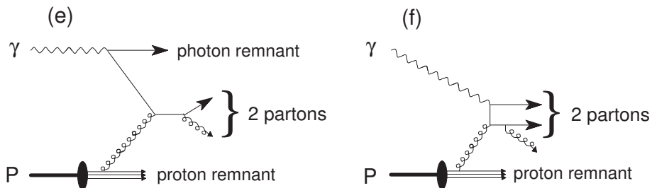
Figure 1.7: Examples for resolved/direct \gamma p process at higher order.
