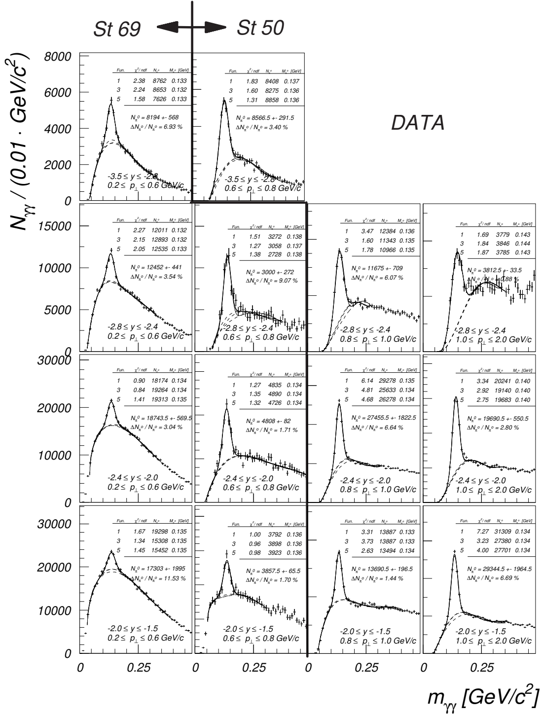
Figure 6.9: m_{\gamma\gamma} spectra ( SpaCal ) in intervals of the \pi^0 transverse momentum and the \pi^0 rapidity fitted by different functions. Table 6.1 gives the fit function referring to the number given in the plots. On the left of the marked line: mass spectra based on the minimum bias run of 1997 (St 69). On the right of the emphasised line: mass spectra based on data, selected by subtrigger 50 (St 50) in 1996.
