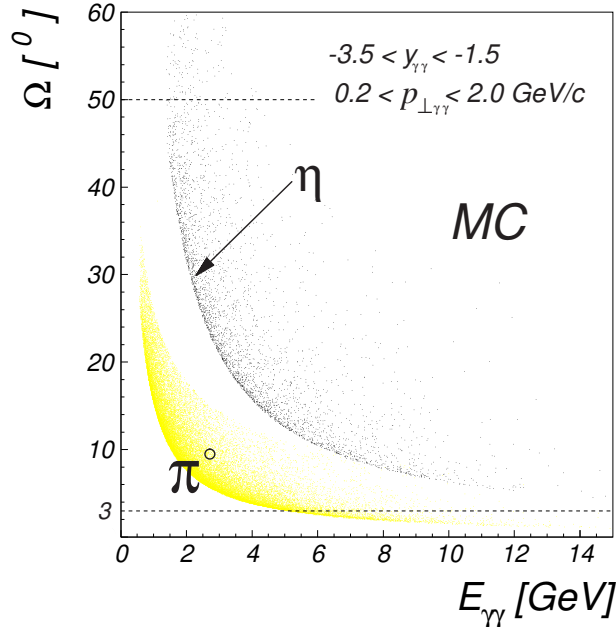
Figure 7.1: PYTHIA : Opening angles of the \pi^0 and \eta decay photons as a function of the energy of the corresponding mother particles. The black lines mark the acceptance region of the SpaCal for the opening angles between photons which were produced perpendicular to the beam axis at the decay of the meson. Only \pi^0 and \eta mesons within the kinematical range -3.5 < y_{\gamma\gamma} < -1.5 and 0.2 < p_{\perp\gamma\gamma} < 2.0 GeV/c were selected.
