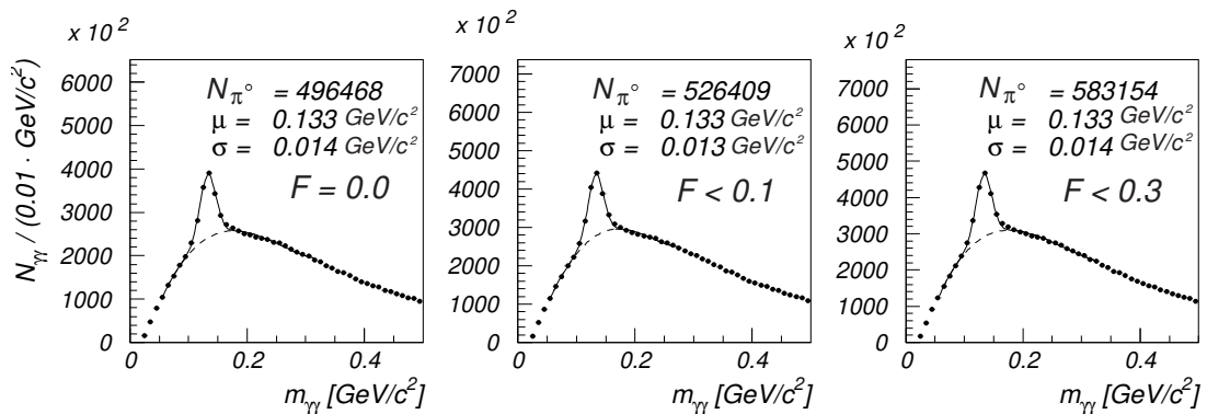
Figure 5.12: SpaCal : m_{\gamma\gamma} distributions with different cuts on the hadronic cluster energy fraction F .
