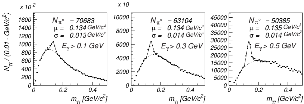
Figure 5.10: SpaCal : m_{\gamma\gamma} distributions with different cuts on the electromagnetic cluster energy E_{cl} .
