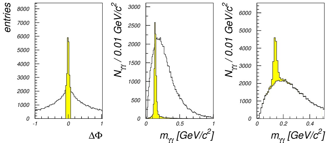
Figure 6.5: Left side: the difference f_{gen.} - f_{det.} for the \pi^0 s found in the SpaCal. Middle: two-photon mass spectra with photon candidates having a strong correlation to generated photons (grey coloured) and two-photon mass spectrum were no correlated photon on generator level could be found. Right side: the sum of the mass spectra shown in the middle plot.
