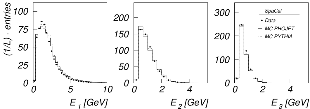
Figure 5.6: SpaCal : Comparison of the energy of the three most energetic clusters in data (points) and the MC models PHOJET (full line) and PYTHIA (dotted line).
