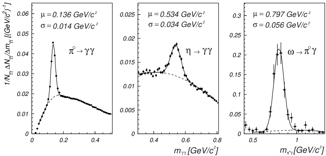
Figure 5.2: The inclusive \pi^0 , \eta and the exclusive \omega signals as seen in the SpaCal after applying the energy scale correction with the help of the \pi^0 mass.
