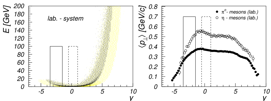
Figure 1.11: Kinematical range accessible for \pi^0 and \eta mesons at HERA. Left side: The \pi^0 and \eta energies versus their laboratory rapidities. The gray points refer to the \pi^0 and the black points to the \eta mesons. Both, the \eta and \pi^0 -meson reach energies up to 820 GeV (= beam energy of incoming protons) in the forward direction. Right side: The mean transverse momenta of the \pi^0 (full points) and \eta mesons (circles) as a function of their lab. rapidities. The kinematical range within the boxes is investigated by this analysis.
