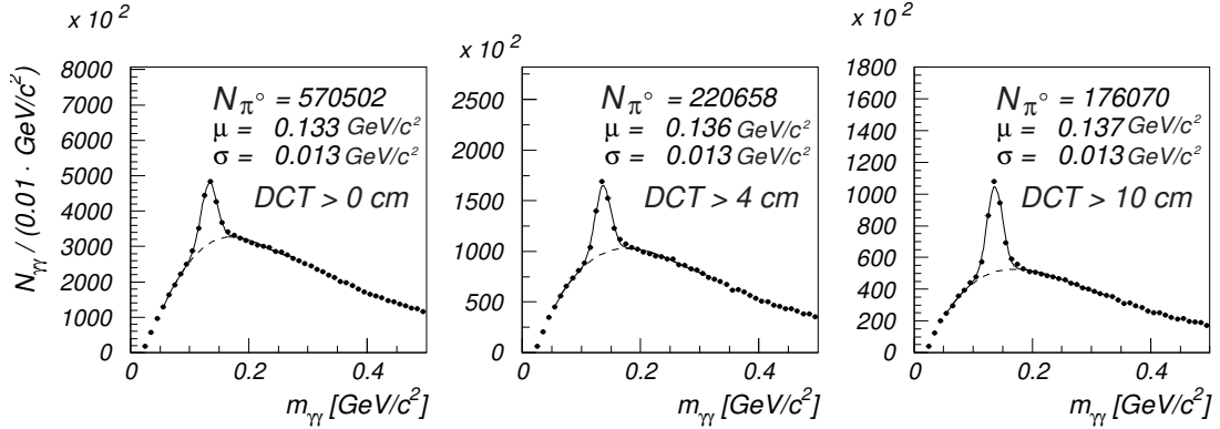
Figure 5.13: SpaCal : m_{\gamma\gamma} distributions for different cuts on the distance of the cluster center to the closest BDC track ( DCT = \text{Distance of Cluster center to closest Track} ).
