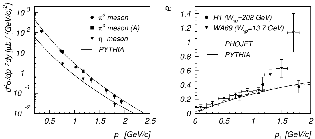
Figure 7.5: Left side: the same cross sections as shown in figure 7.4. The squares (A) show the \pi^0 cross section measured in the same bins in which the \eta cross section is measured. Right side: Ratio R of the \eta/\pi^0 photoproduction cross sections as a function of the transverse momenta of the mesons in the interval -3.5 < y < -1.5 . R = \frac{d^2\sigma}{dp_{\perp}^2 dy}(\eta) / \frac{d^2\sigma}{dp_{\perp}^2 dy}(\pi^0) .
