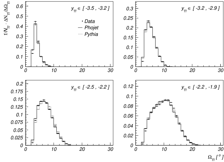
Figure 6.7: Opening angle \Omega_{\gamma\gamma} of all possible two-cluster combinations in the mass band of the \pi^0 ( 0.1 < m_{\gamma\gamma} < 0.17 \text{ GeV}/c^2 ) in intervals of the rapidity of the cluster pairs (SpaCal).
