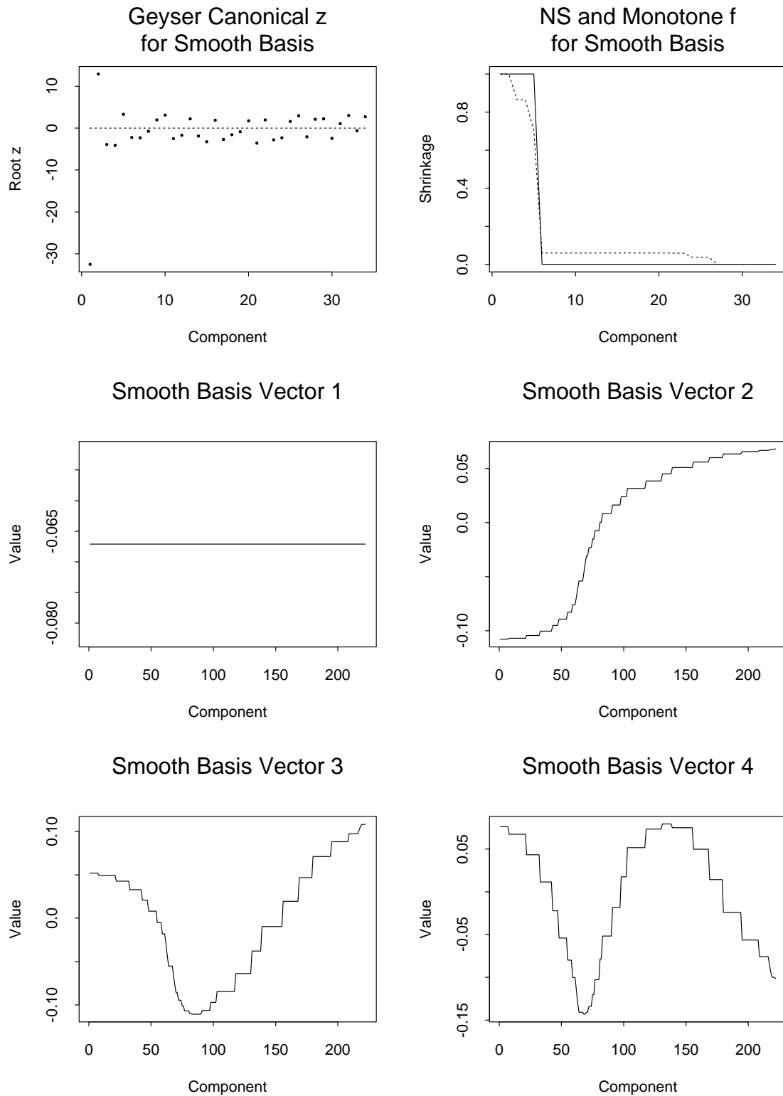
FIG 5. The second and third rows exhibit the first four vectors in the smooth basis U_S for the geysers data. The top row displays the canonical response z = U_S' y and, on the right, the shrinkage vectors \hat{f}_{NS} (solid line) and \hat{f}_M (dashed line) for the smooth basis.
