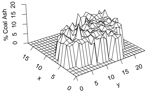
Least Squares Fit to Coal Ash Data
