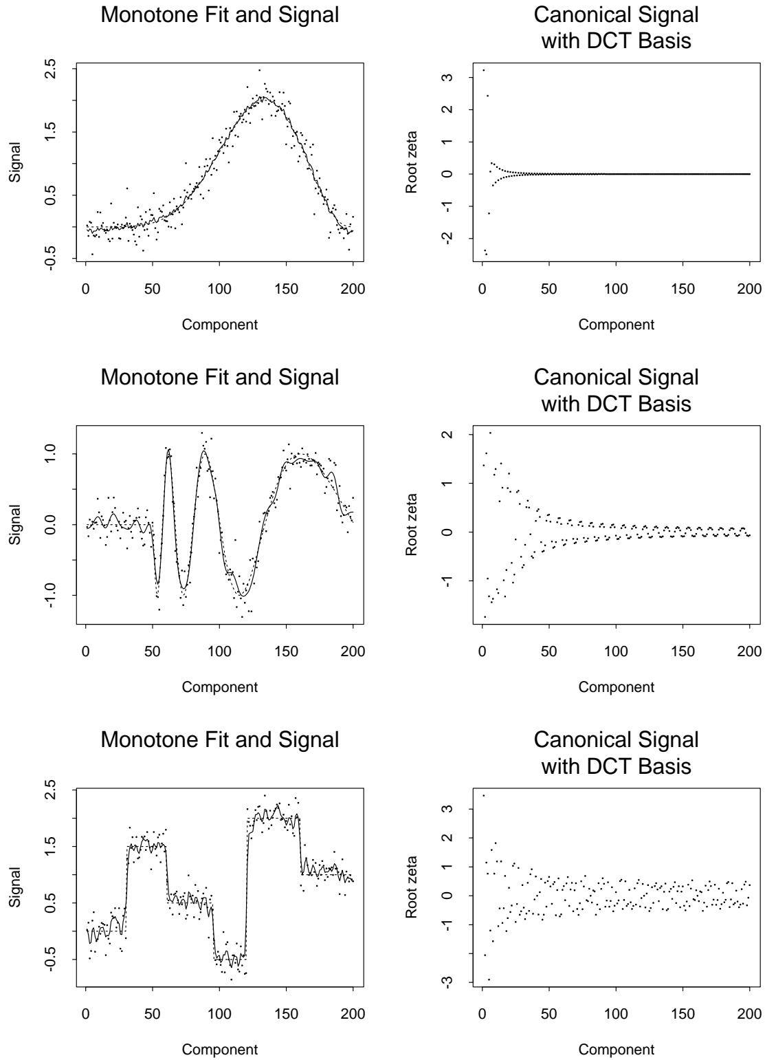
FIG 10. For three trend vectors \eta (dashed line), the left column displays a trend plus noise sample y of size 200 and its monotone REACT fit (solid line) using the discrete cosine basis U_{DC} . The canonical mean vectors \xi = U_{DC}^T \eta in the right column show that this basis is less economical for the second and third trends.
