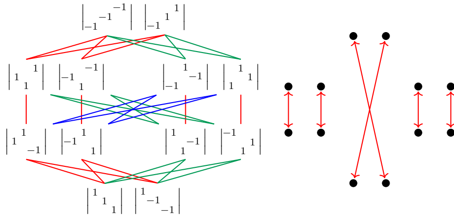
Figure 2.3: The Bruhat order on R \backslash \widetilde{W} and the involution given by w_0 . Different colors are used purely for better visibility.
