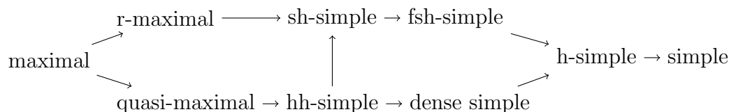
Figure 4.1: Most common simplicity properties and their relations among each other. An arrow P \rightarrow Q indicates that property P implies property Q but not vice versa.
