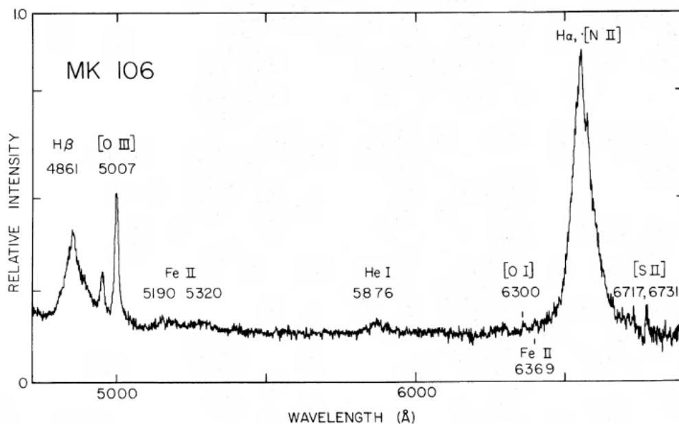
Figure 1.3 Early depiction of optical BELs of the Seyfert 1 galaxy Mrk 106. Especially H \alpha and H \beta are prominent although superposed by NELs (indicated by the square brackets). The figure was taken from Osterbrock (1977) .
