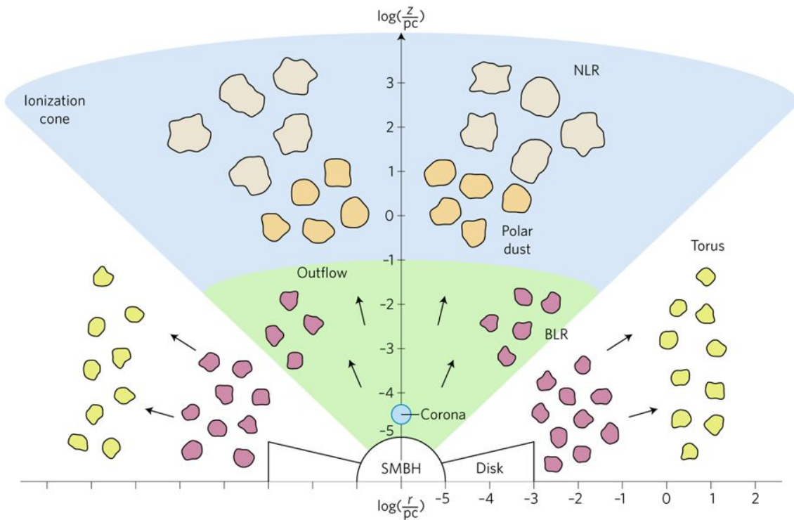
Figure 1.2 State-of-the-art view of the structure of AGN from the immediate vicinity of the SMBH to host galaxy scales. Graphic is taken from Ramos Almeida & Ricci (2017) .
