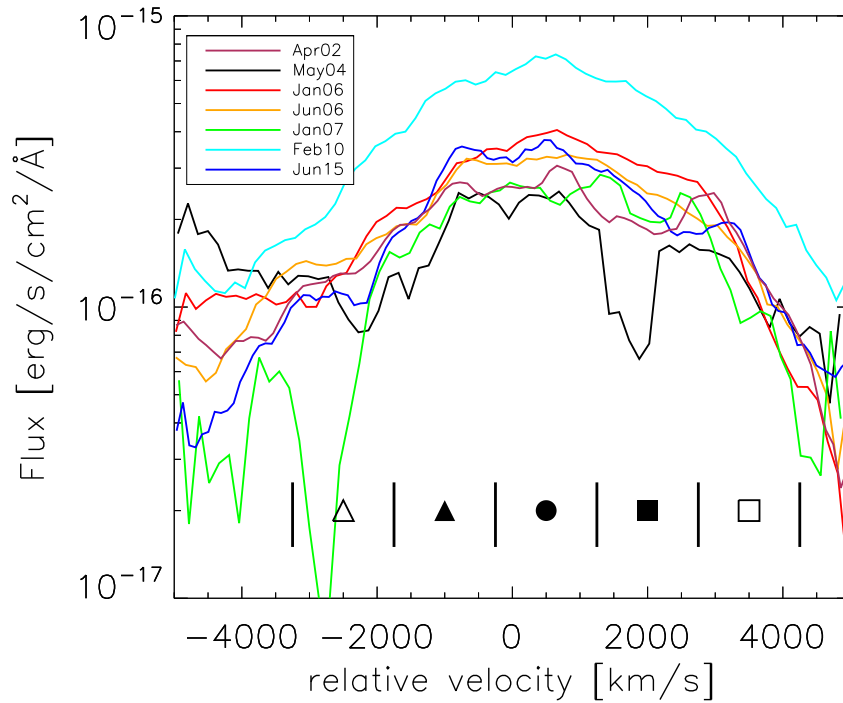
Figure 4.4 Same as Fig. 4.2 for the Bry BEL.
