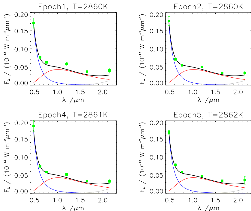
Figure 3.9 Observed fluxes and fit according to our model (compare Eq. 3.1) and an additional blackbody due to the increased flux in the K band. The third epoch is not shown as the flux in the H and K band is not available in this case. The green squares show the fluxes with the host extinction correction, the blue line the AD model, the red line the blackbody of the dust model with the higher temperature ( 2857_{-68}^{+65} K), the gray line the blackbody of the dust model with the lower temperature ( 576_{-23}^{+54} K), and the black line the combined fit. The hotter temperature for each epoch is given at the top of the corresponding plot.
