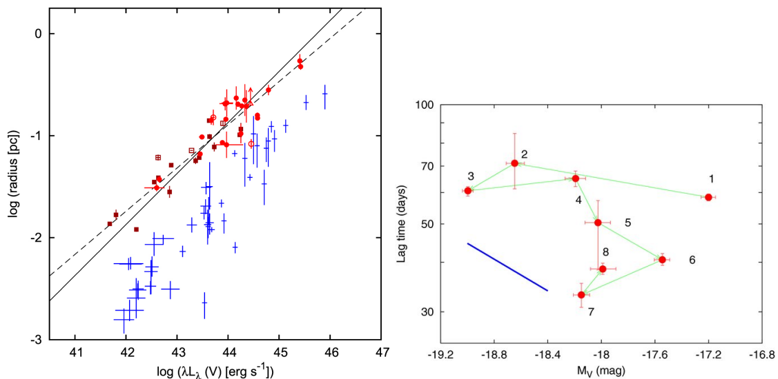
Figure 1.4 In the left figure (taken from Minezaki et al. 2019) the radius luminosity relation for the BLR (blue crosses) from Bentz et al. (2013) using Balmer emission lines and the dust torus (red symbols) from Koshida et al. (2014) and Minezaki et al. (2019) are shown. The solid line represents a fit to the dust radii with a slope fixed at 0.5 while the dashed line represents a fit with free slope. In the right figure (taken from Koshida et al. 2009) the evolution of the radius luminosity relation of NGC 4151 over six years is shown. The solid line indicates the expected \tau \propto L^{0.5} relation, which is not in agreement with the data.
