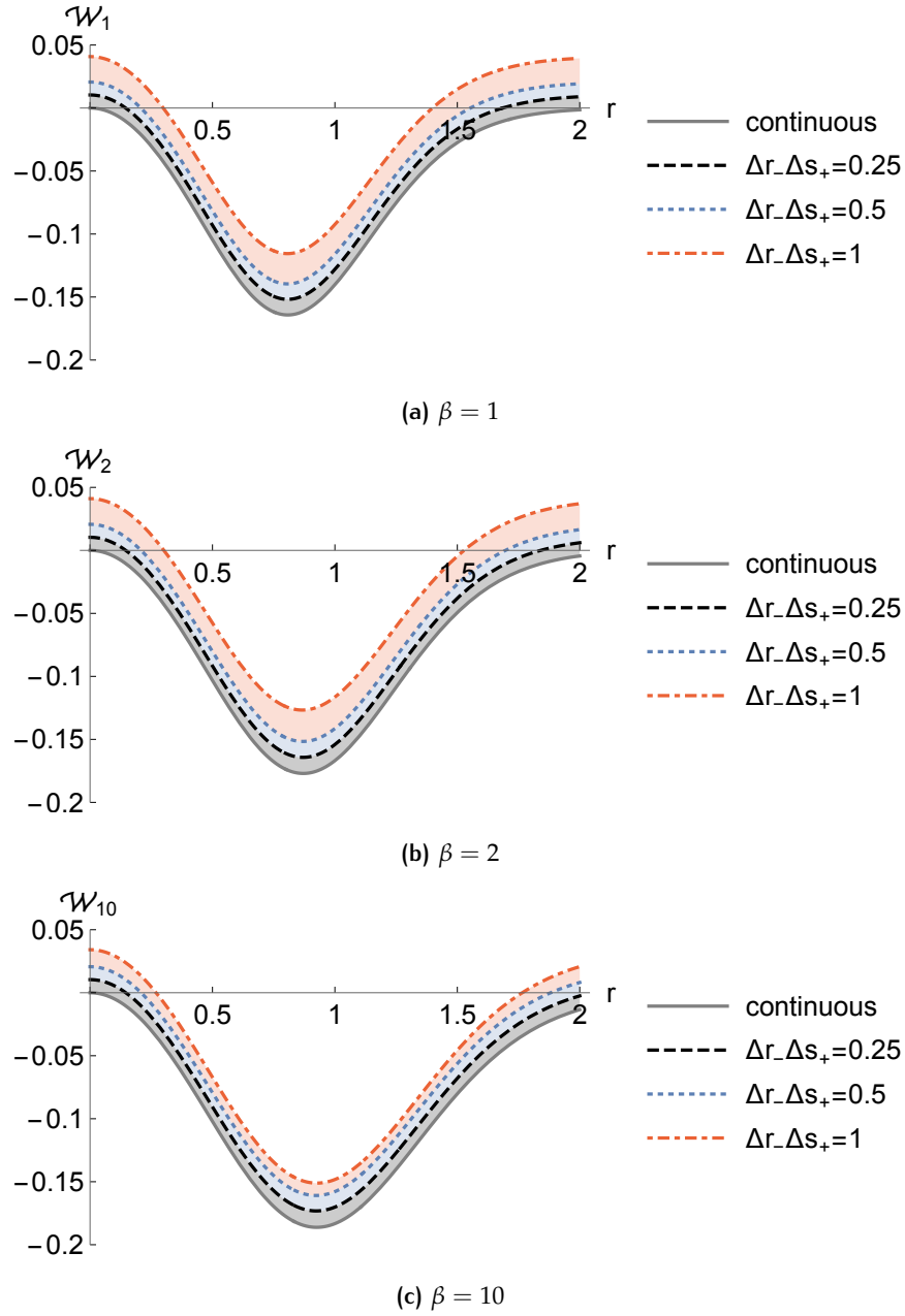
Figure 13.2: Continuous vs. discretized Rényi-Wehrl entropic criteria (cf. (13.27)) for the dephased Schrödinger cat state (12.26) with s = z = 0 as a function of r for various bin sizes \Delta r \Delta s_+ . Entanglement is witnessed for negative \mathcal{W}_\beta , which is defined as the difference of the two sides in (13.27). We show the Wehrl criteria in (a), while (b) and (c) depict higher-order Rényi-Wehrl entropies with \beta = 2 and \beta = 10 , respectively. For discretized data, detecting entanglement becomes harder for small r \lesssim 0.25 and large r \gtrsim 1.5 .
