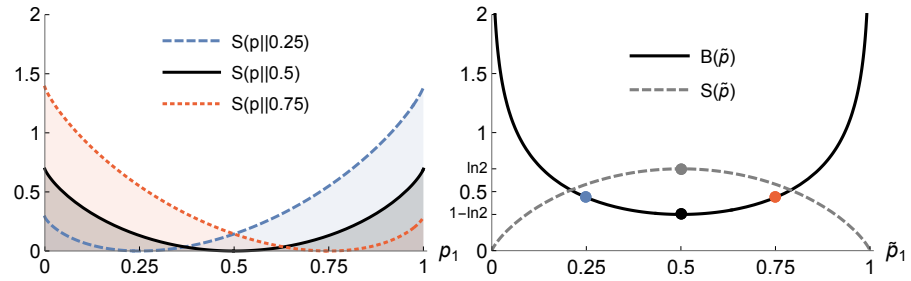
(a) Three relative entropies S(p||\tilde{p}) (b) B -functional B(\tilde{p}) and entropy S(\tilde{p})
