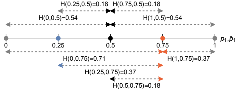
(c) Exemplary Hellinger distances for the two models \tilde{p}_1 = 0.5, 0.75
