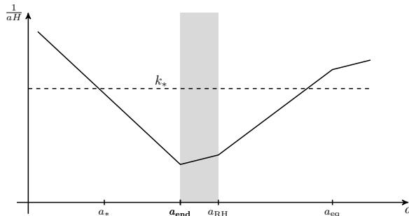
Figure 4.1: Evolution of the comoving Hubble radius (solid line) and a perturbation (dashed line) with corresponding comoving wavenumber k_* = a_* H_* . The gray area indicates the era of reheating. The scale factor a_{\text{end}} denotes the end of inflation, a_{\text{RH}} denotes the start of radiation domination and a_{\text{eq}} denotes matter-radiation equality.
