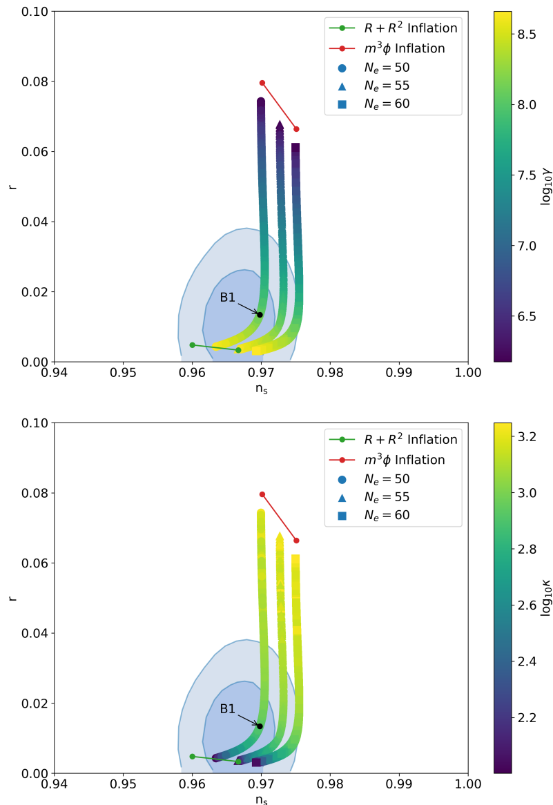
Figure 6.1: Predictions for the scalar spectral index n_s and the tensor-to-scalar ratio r with varying numbers of e-folds N_e are displayed. All shown points are taken according to the parameter ranges in (6.35) while satisfying the A_s -constraint (5.43). The color gradient shows \gamma in the upper and \kappa in the lower plot. The blue regions indicate the Planck TT,TE,EE+lowE+lensing+BK18+BAO 68% and 95% CL regions from [131, 235]. We also included the predictions of the Starobinsky model (green) and linear inflation (red), where the circles represent the predictions for N_e = 50 (left) and N_e = 60 (right) e-folds respectively. This exemplifies that our results interpolate between these two results as in Fig. 5.4. The effect of corrections to r due to the C^2 term as discussed in [183–185] are included in Fig. 6.2.
