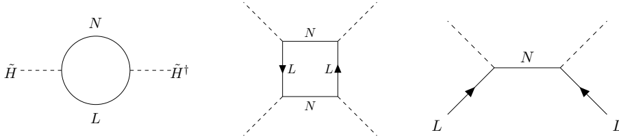
Figure 5.5: Neutrino contributions to the Higgs mass term (left) and Higgs quartic coupling (middle). The Feynman diagram in right panel generates light active neutrino masses through the type-I seesaw mechanism.
