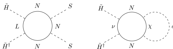
Figure 5.7: Neutrino contribution to the Higgs portal coupling \lambda_{HS} (left) and dark matter two-loop contribution (right) to the Higgs mass.
