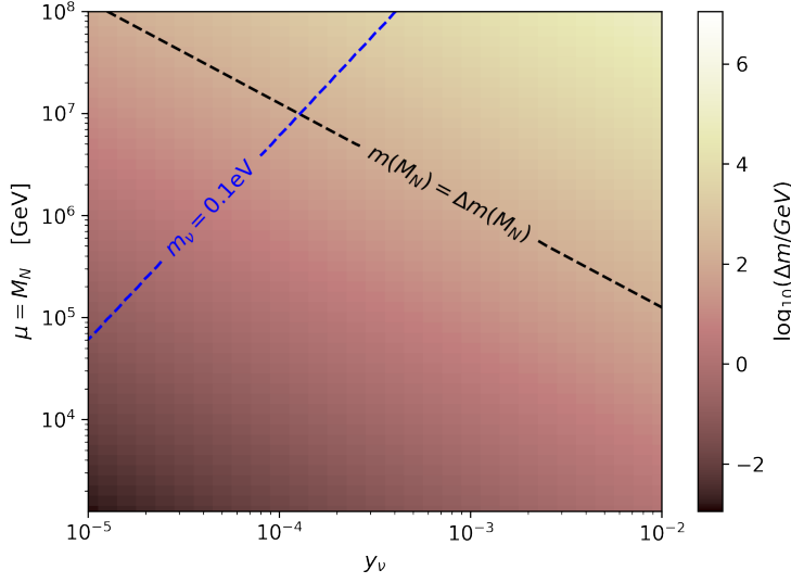
Figure 5.6: The threshold correction to the Higgs mass parameter (5.47) due to the Majorana mass M_N of right-handed neutrinos. Along the black dashed line the matching condition is satisfied, where the threshold correction at the matching scale \mu = M_N equals the running Higgs mass parameter of the SM m(m_N) at the matching scale. The blue line indicates the light neutrino mass scale obtained by the seesaw mechanism (5.50). Both conditions are satisfied at the intersection of the two lines at y_\nu \simeq 10^{-3.9} and M_N \simeq 10^7 GeV.
