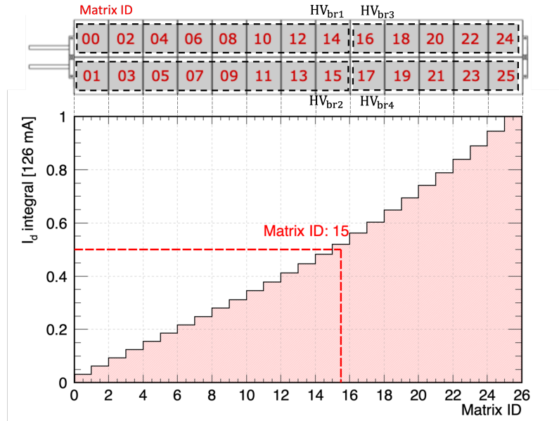
Figure 8.3: Integral of I_d along Matrices. The integral for each bin is the current sum of all the Matrices with IDs not larger than the bin value. Each Tile Detector Module is biased by four HV branches: branch 1 for Matrices 0 to 15 with even IDs, branch 2 for Matrices 0 to 15 with odd IDs, branch 3 for Matrices 16 to 25 with even IDs, and branch 4 for Matrices 16 to 25 with odd IDs.
