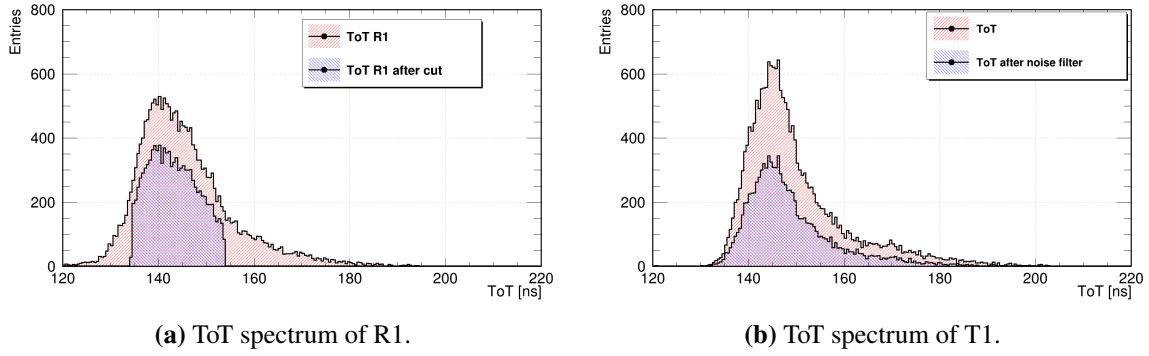
Figure 7.11: Comparison of ToT in channel (a) R1 and (b) T1 before and after the ToT filter implementation. (a) The sharp edge in the distribution after filter is due to the cut in R1 and the missing events within the range [\mu_{\text{ToT}} - 1.5 \cdot \sigma_{\text{ToT}}, \mu_{\text{ToT}} + 3.5 \cdot \sigma_{\text{ToT}}] were filtered out by the ToT filter in channel R2. (b) No direct cut was implemented on T1 and T2 to preserve all the timing jitter contribution from different E_{\text{dep}} .
