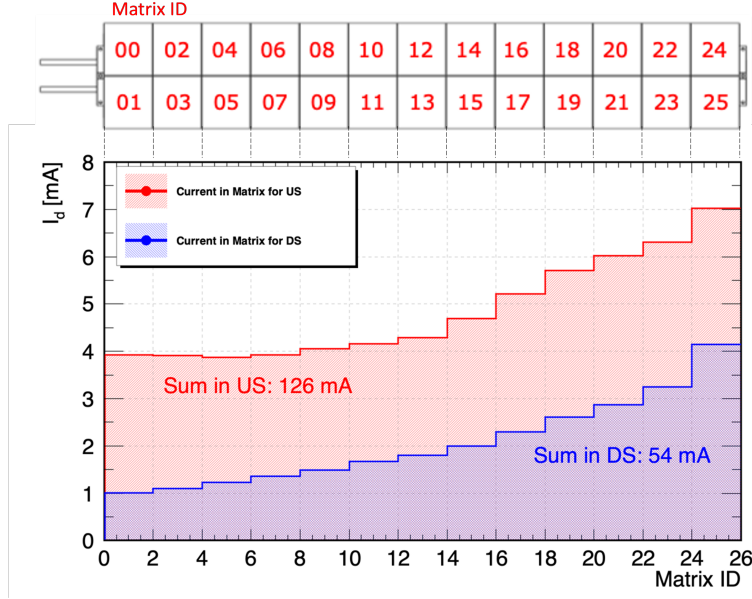
Figure 8.2: I_d in different Tile Detector Matrices. Matrices with larger IDs are closer to the center of the experiment, and the two pipes close to Matrices 0 and 1 are cooling pipes. Matrices mounted on the same z position, e.g. Matrix 0 and 1, have the same I_d , which is due to the symmetry of dose along \phi .
