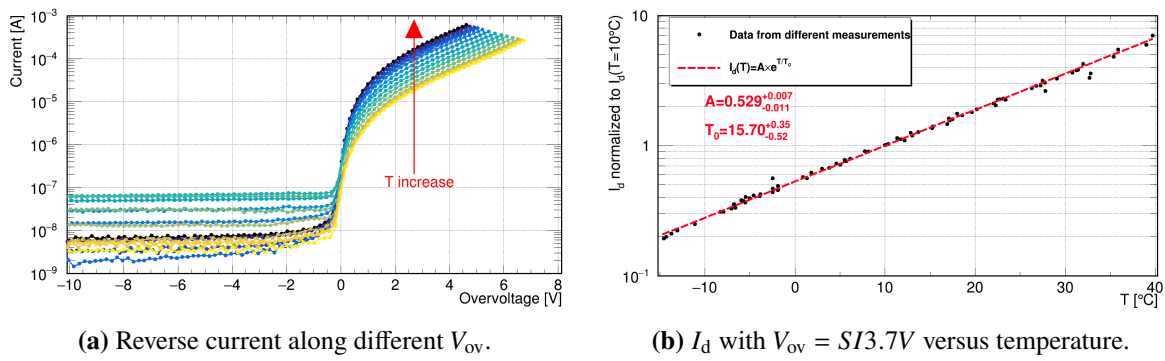
Figure 6.19: (a) IV curve and (b) I_d with a constant V_{ov} at different temperatures. (b) Fitting results reveal that I_d decreases by a factor of e when the temperature drops by 15.7^\circ C .
