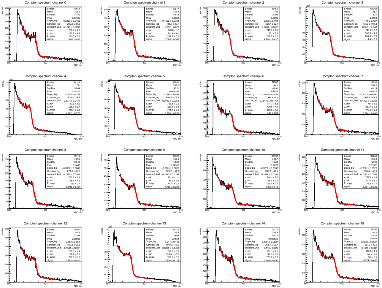
Figure B.14: Determination of the Compton edge position for the all channels of matrix ID = 02. The spectra taken with the ^{22}\text{Na} source are fitted with a convolution of a Gaussian error function describing the edge and a linear function for the background to extract the position of the Compton edge \mu_{CE} .
