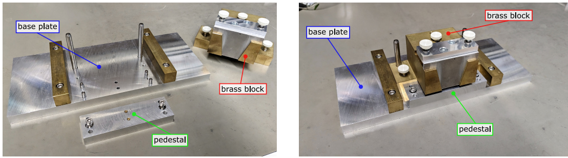
(a) Photo of a disassembled gluing tool.
